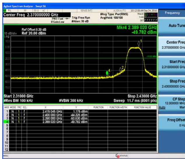
Left bandedge
