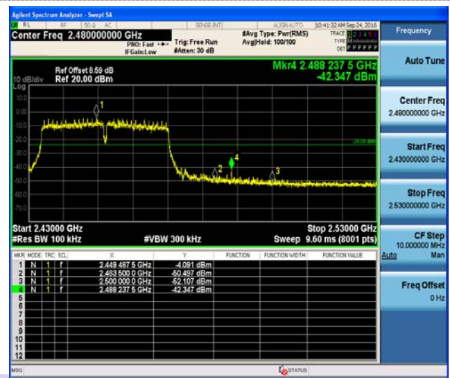
Right bandedge
