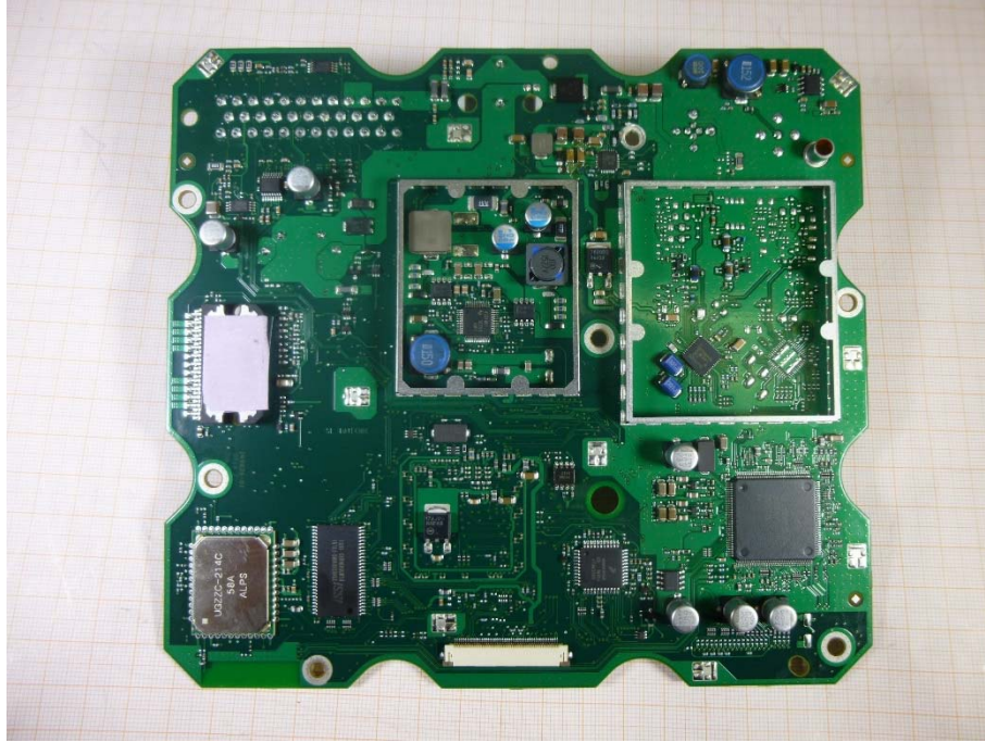
Photo 5: PCB back side view without shieldings
