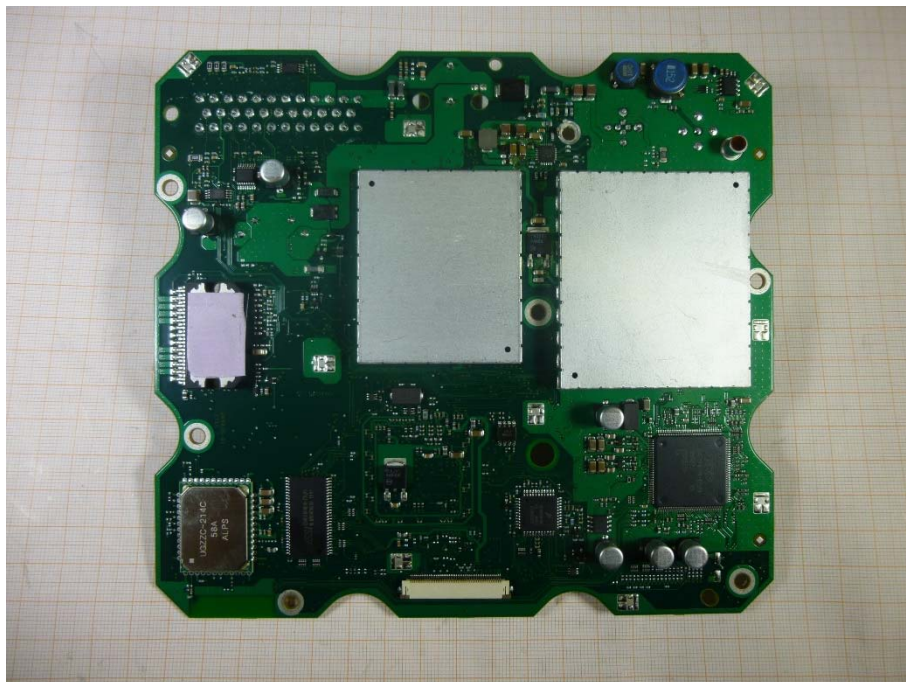
Photo 4: PCB back side view with shieldings
