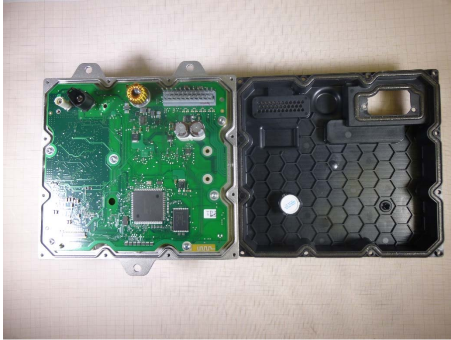
Photo 1: EUT opened
