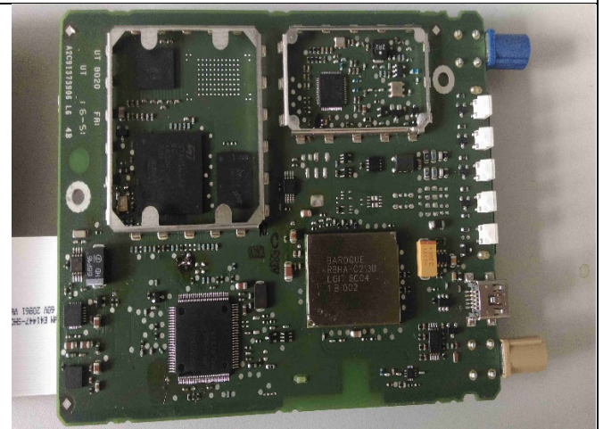
FLEXCM-Main Board- Bottom View
