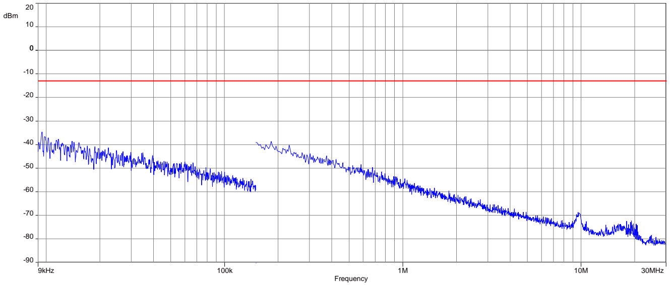
Plot 1: Channel 661 (Traffic mode up to 30 MHz)
