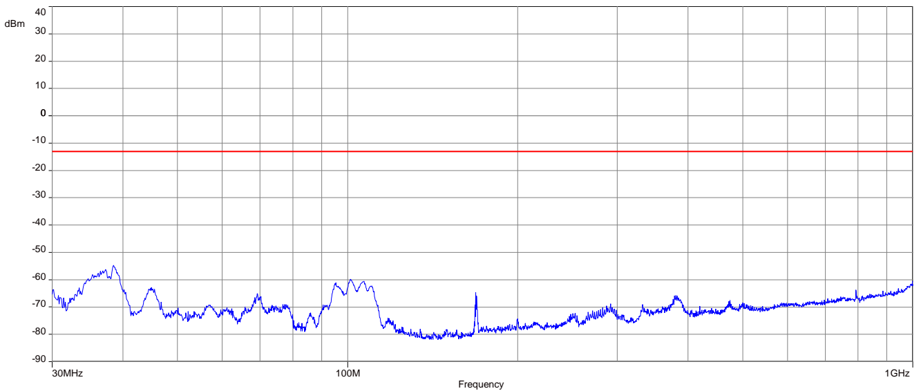
Plot 2: Channel 661 (30 MHz – 1 GHz)
