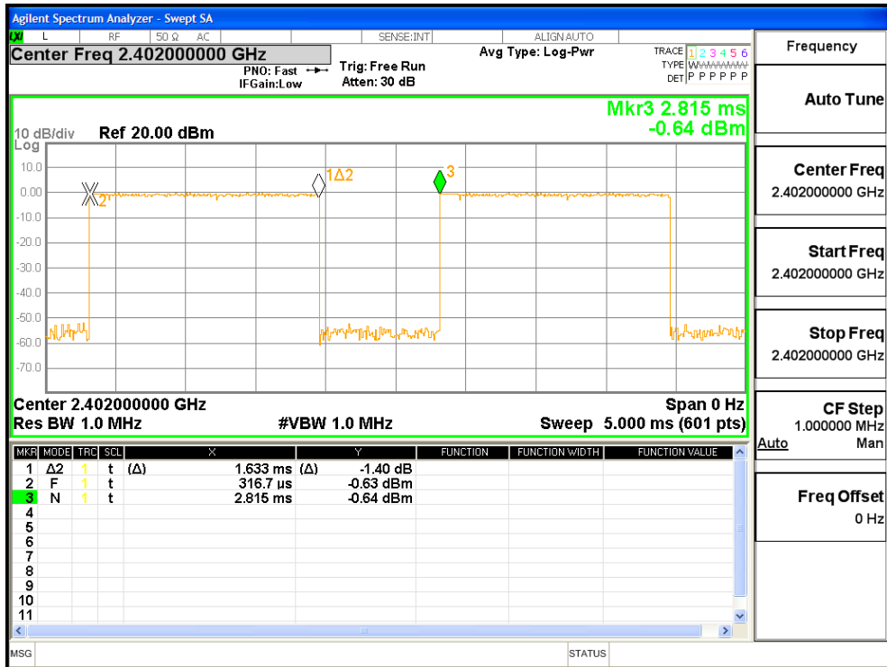
Test Mode: \pi/4 DQPSK ---2DH3
