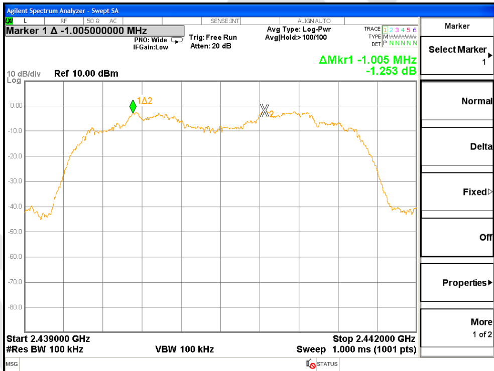
Test Mode:8DPSK---Middle
