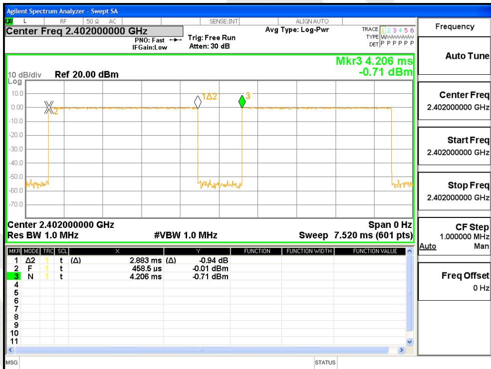
Test Mode: \pi/4 DQPSK ---2DH5
