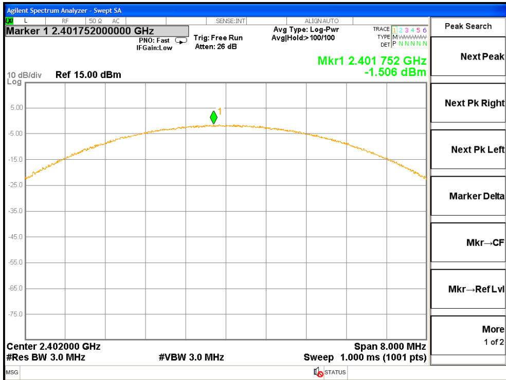
Test Mode:8DPSK---Low
