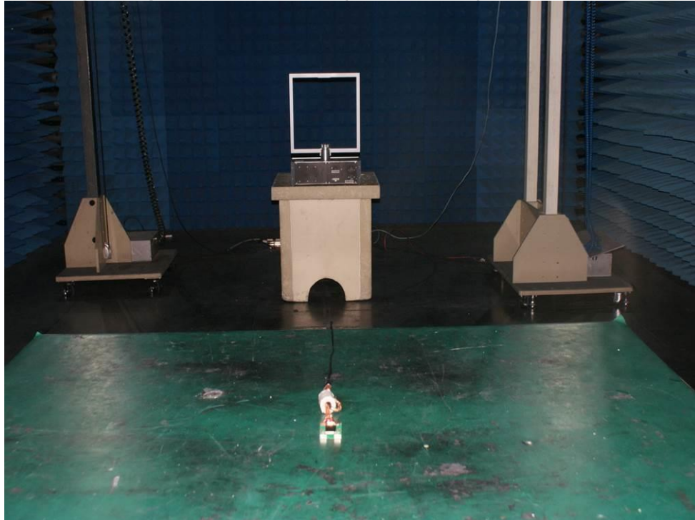
Photograph 1: Set-up for Spurious Emissions (9 kHz-30MHz)
