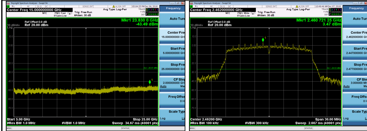
802.11n(HT20),2462MHz,Ant1,Plot 2,Band Edge
