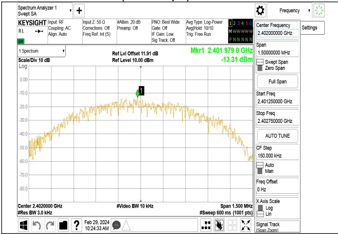
Test Mode: GFSK (LE 1Mbps)
