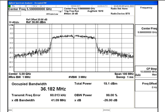
Mode:802.11ac VHT40 Frequency:5590MHz Ant:Chain0
