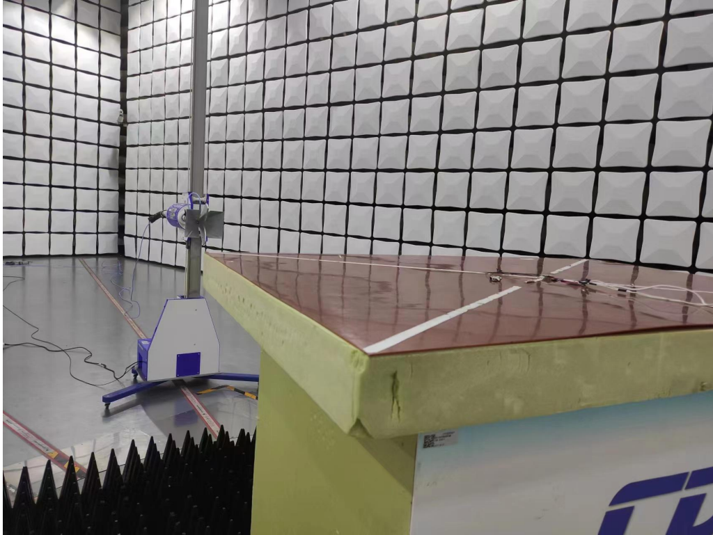
RE>1GHz
