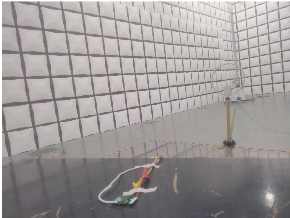
RE 9KHz~30MHz
