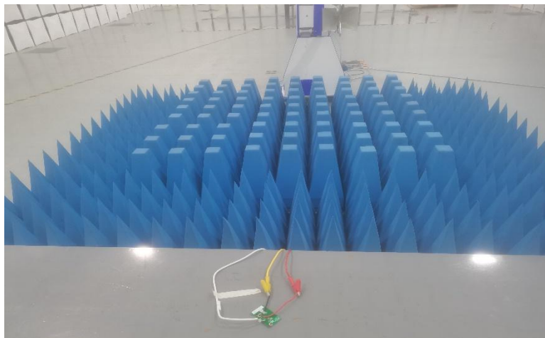
RE >1GHz
