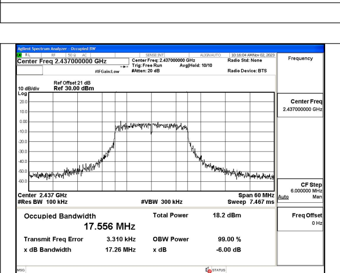
Mode:802.11n HT20 Frequency:2437MHz Ant:Chain0
