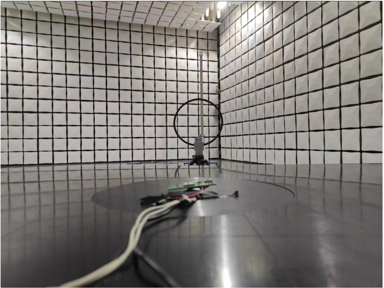
RE 9KHz~30MHz
