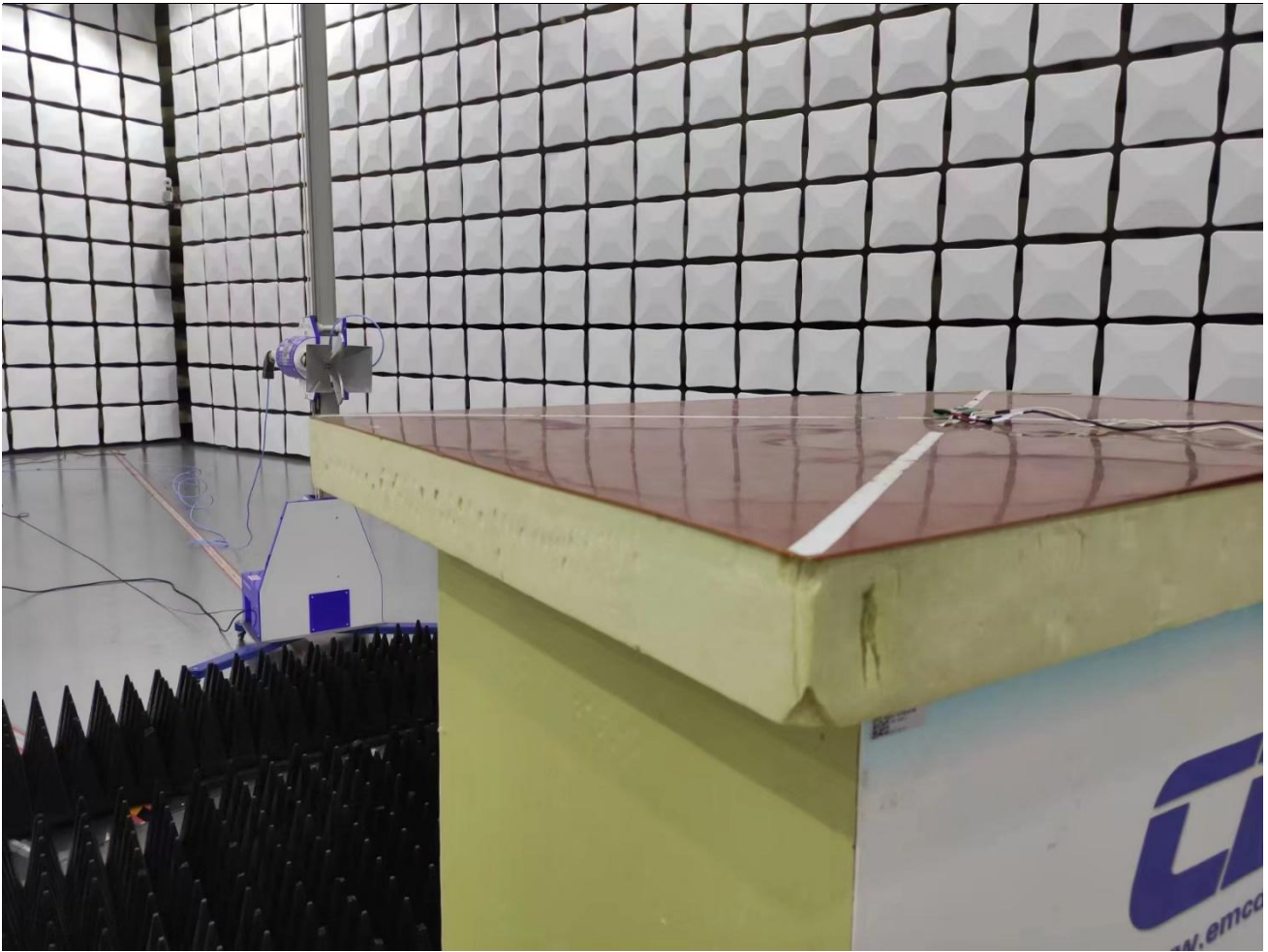
RE >1GHz
