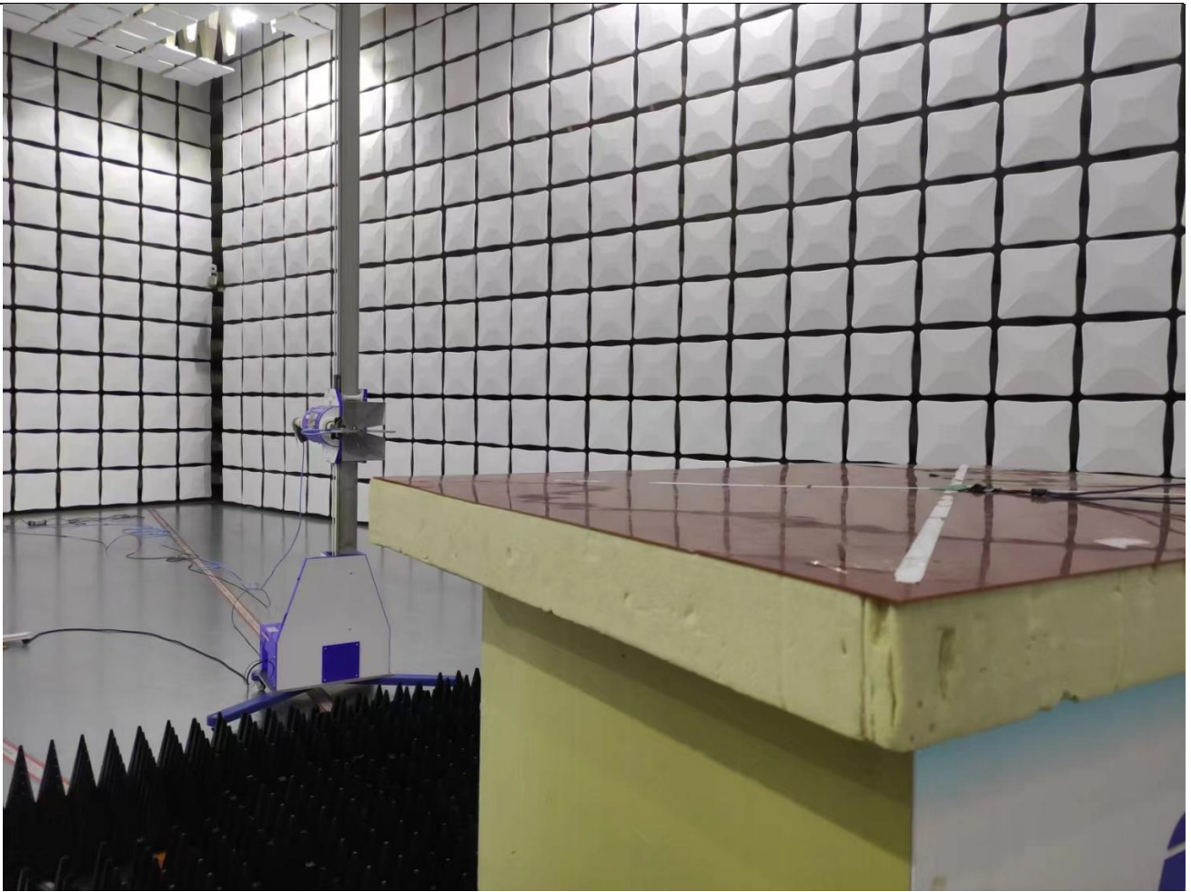
RE>1GHz
