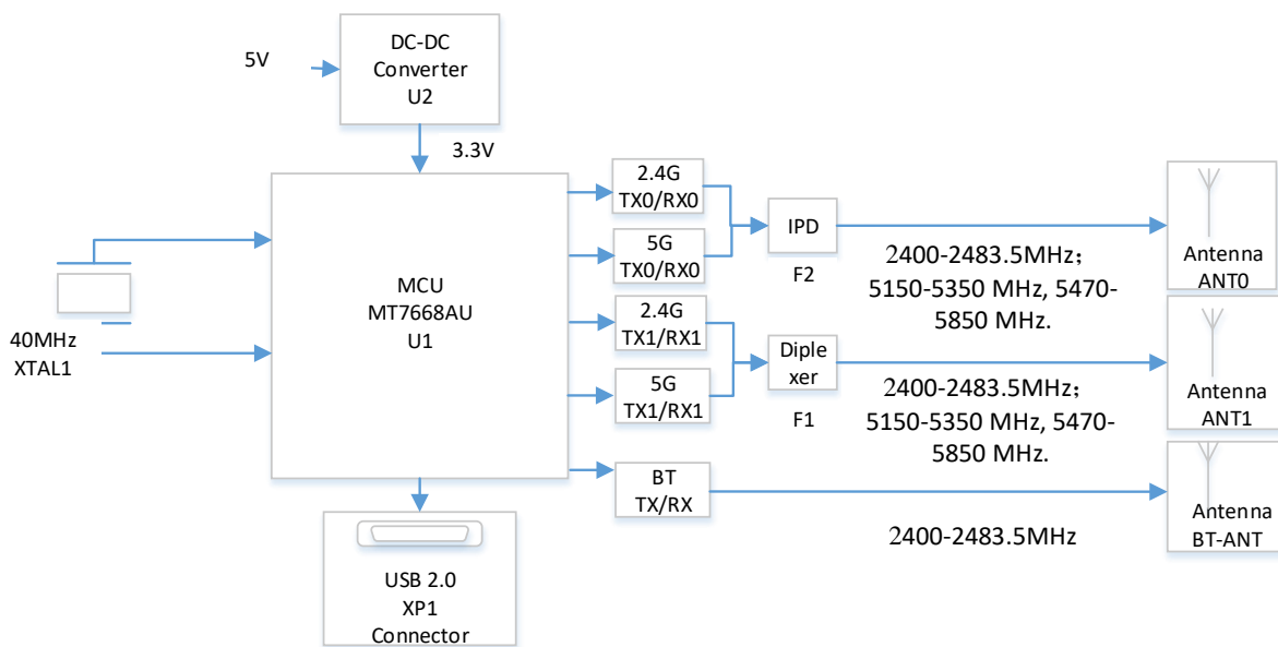
BLOCK DIAGRAM
