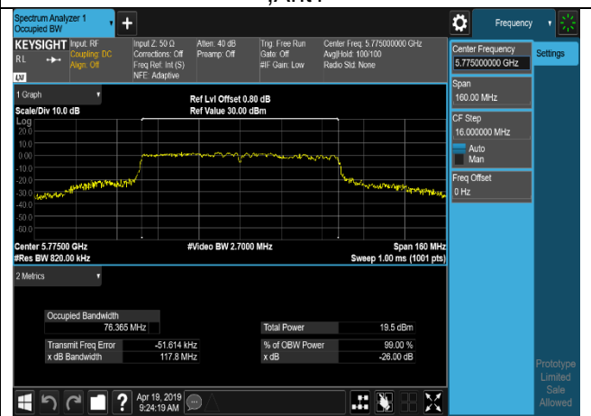
U-NII-3,802.11ac(VHT80),5775MHz,Ant1
