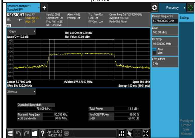
U-NII-3,802.11ac(VHT80),5775MHz,Ant0
