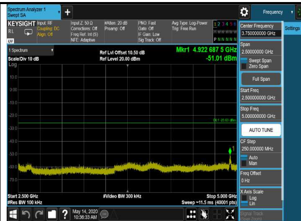
802.11g,2462MHz,Ant1,Plot 1,Reference Level
