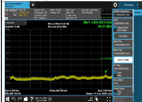
802.11n(HT40),2437MHz,Ant0,Plot 1,Reference Level
