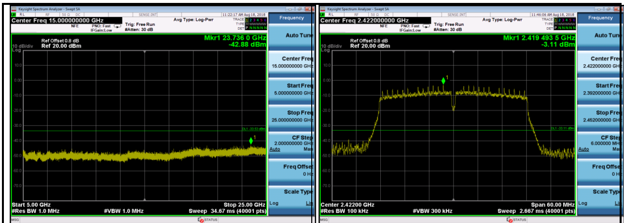
802.11n(HT40),2422MHz,Ant1,Plot 2,Band Edge
