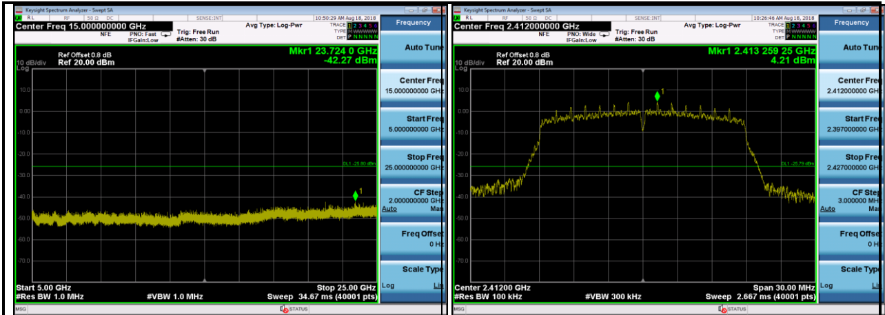
802.11n(HT20),2412MHz,Ant1,Plot 2,Band Edge
