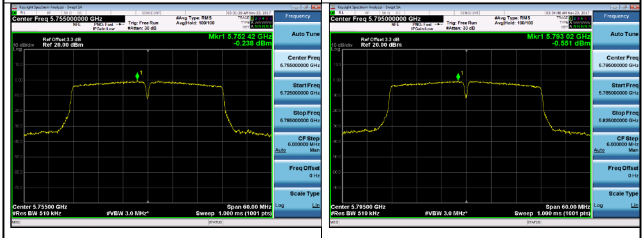
U-NII-3 Power spectral density : 802.11n(40MHz),5755MHz,Ant1
