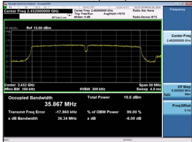
802.11n (HT40)2452MHz
