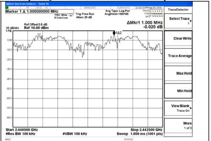
Test Plot Of Frequency Separation (2Mbps)
