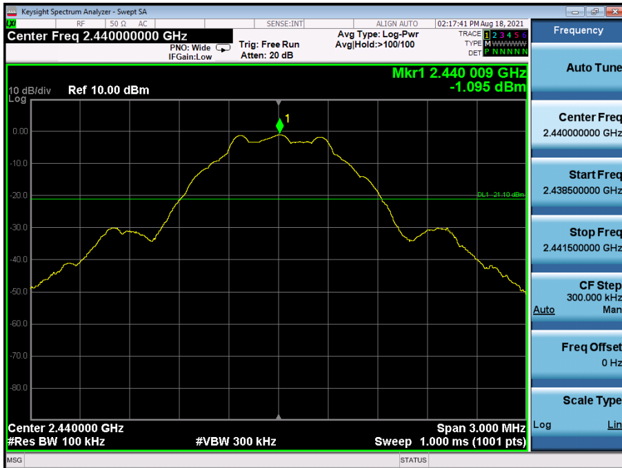
CH: 2440MHz
