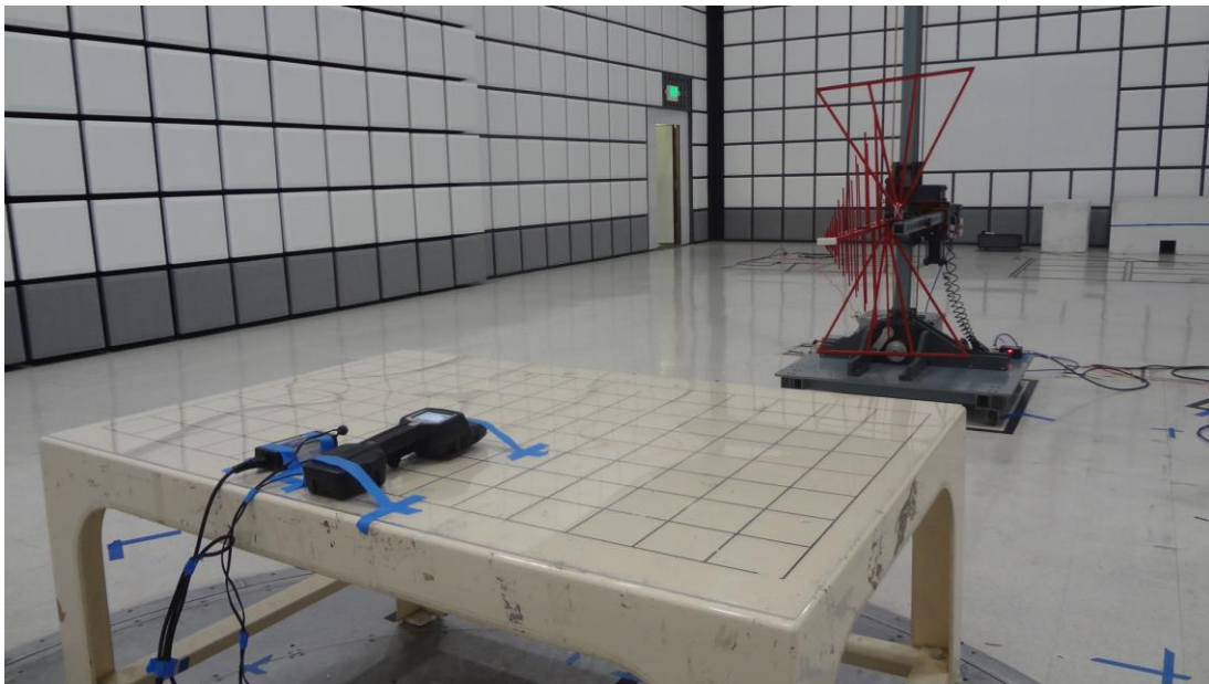
Radiated Emissions Test Setup (below 1GHz)
