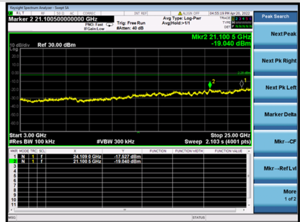
LOW CHANNEL, SPURIOUS 3 GHz ~ 25 GHz
