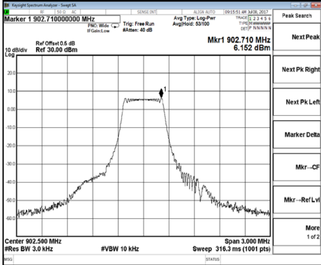
Channel 0 / 902.5 MHz
