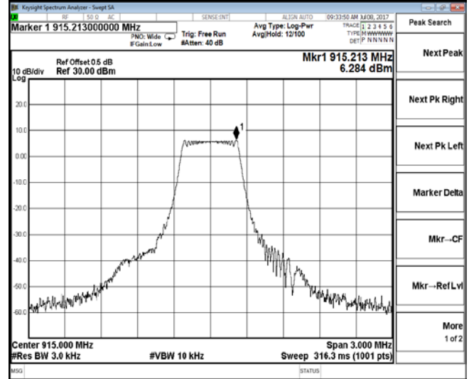
Channel 05 / 915 MHz
