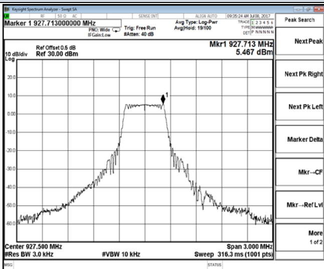
Channel 10 / 927.5 MHz
