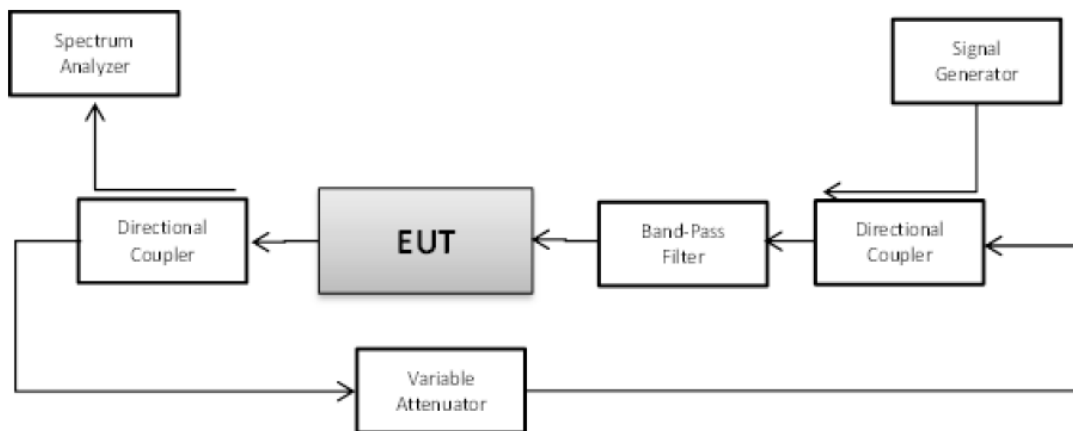
Figure 8 – Oscillation mitigation/shutdown test setup
