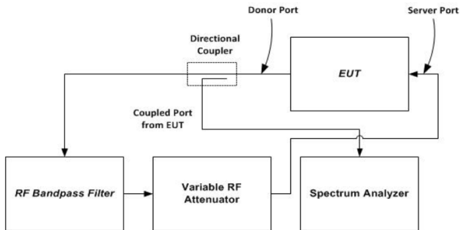
Figure 7 – Oscillation detection (7.11.2) test setup
