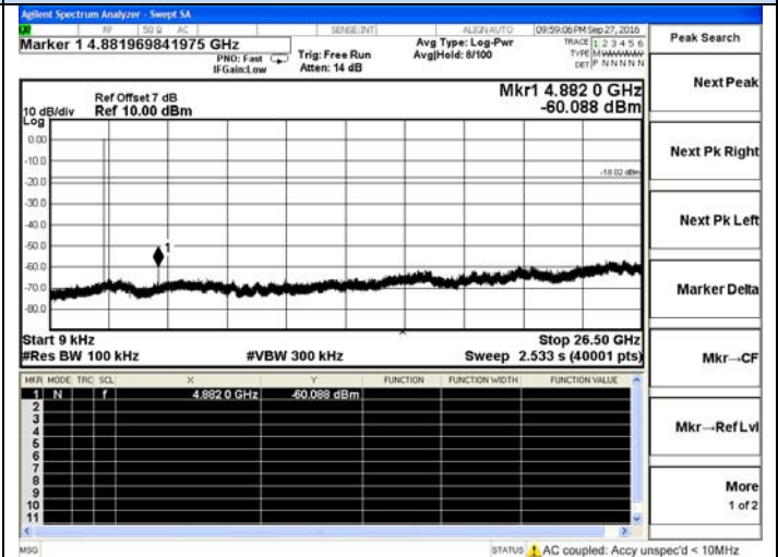
3DH1-Middle channel
