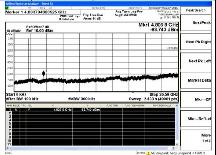
3DH1-Low channel
