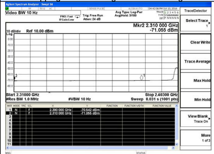
Hopping Off- \pi/4 -DQPSK- Low channel-Average
