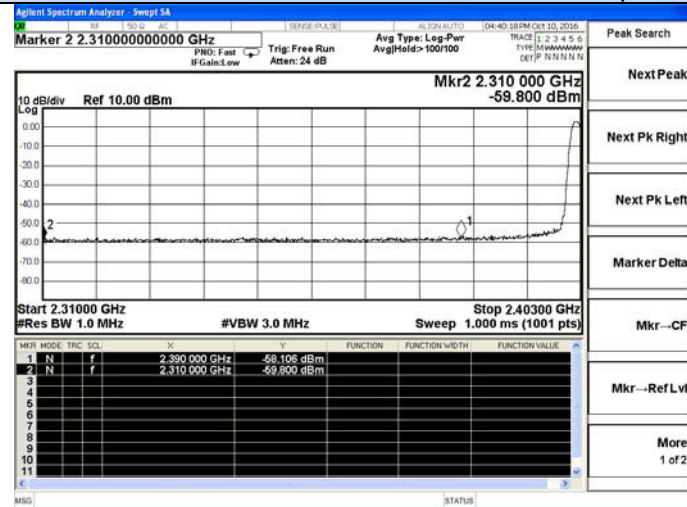
Hopping Off-GFSK-Low channel-Peak
