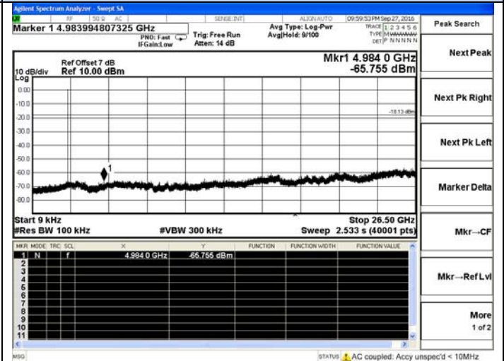
3DH1-High channel
