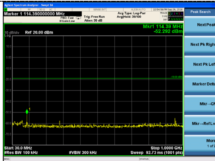
30MHz~1GHz
