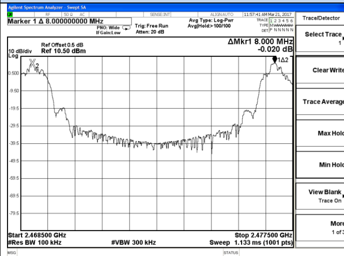
Channel 15 / 2477 MHz
