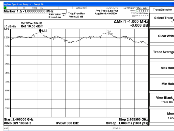
Channel 0 / 2407 MHz
