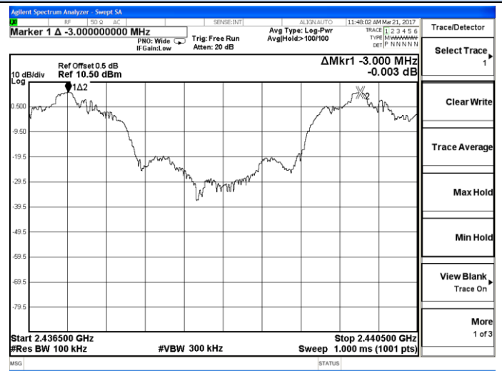
Channel 5 / 2440 MHz
