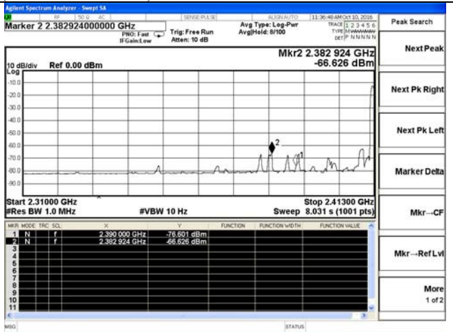
Test frequency: 2412MHz-Average
