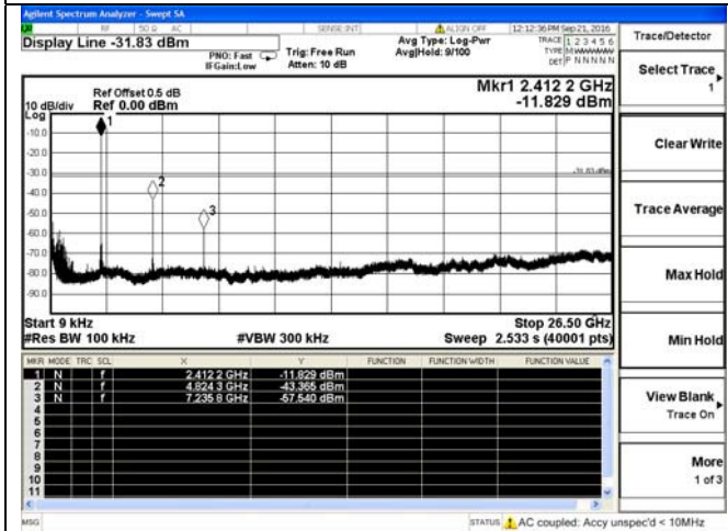
Test frequency: 2412MHz
