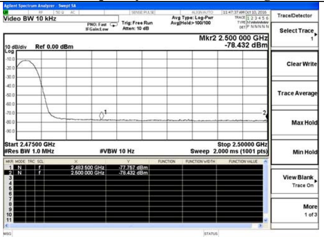
Test frequency: 2476MHz-Average
