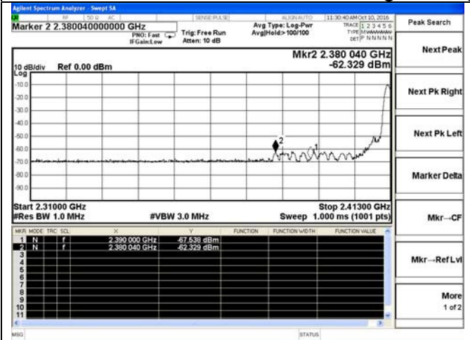
Test frequency: 2412MHz-Peak
