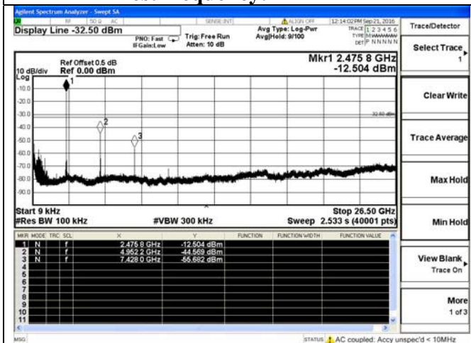
Test frequency: 2476MHz
