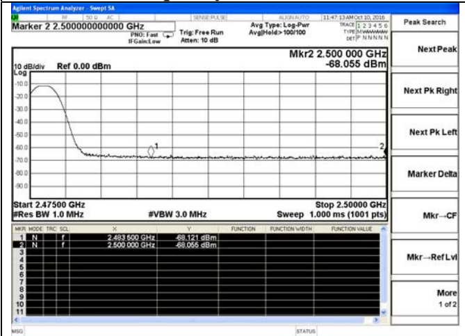
Test frequency: 2476MHz-Peak
