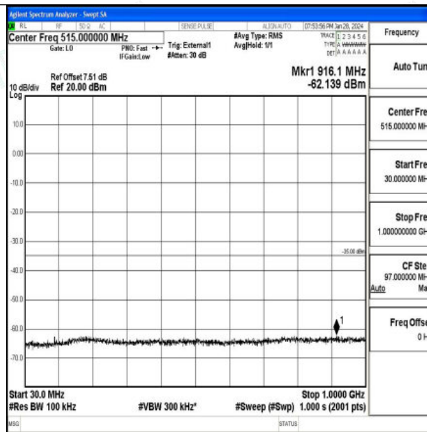
Band41_15MHz_QPSK_41515_1RB#0_30~1000_30~1000
