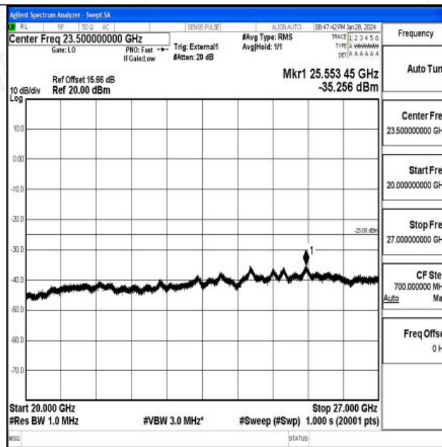
Band41_10MHz_QPSK_40620_1RB#0_20000~27000_20000~27000
