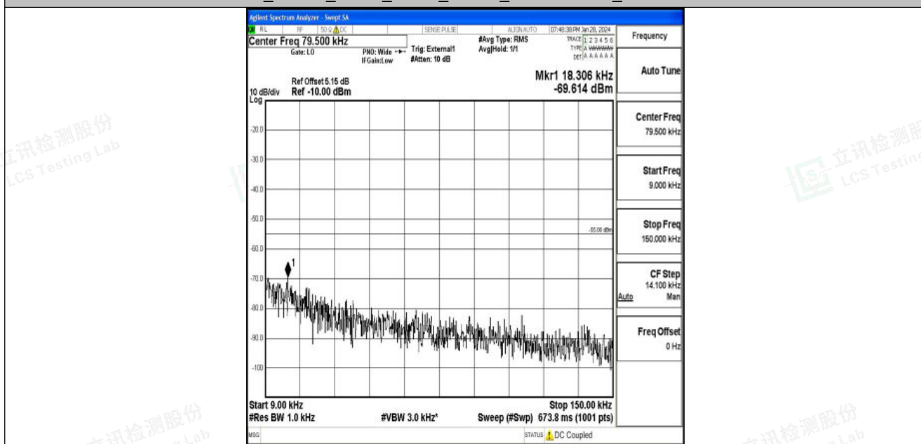
Band41_15MHz_16QAM_39725_1RB#0_0.009~0.15_0.009~0.15
