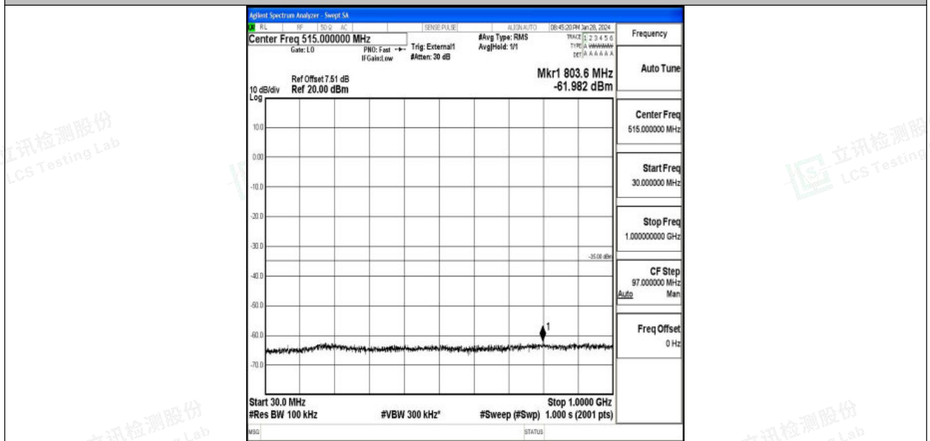
Band41_10MHz_16QAM_39700_1RB#0_30~1000_30~1000
