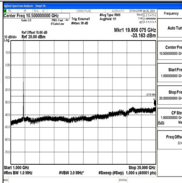
Band41_15MHz_QPSK_41515_1RB#0_1000~20000_1000~20000
