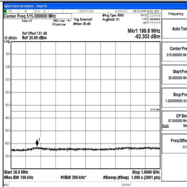
Band41_20MHz_16QAM_40620_1RB#0_30~1000_30~1000
