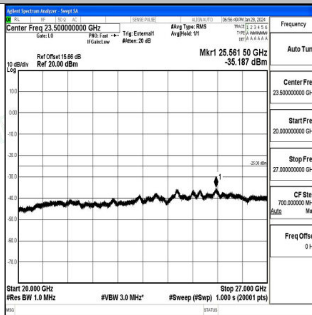
Band41_5MHz_16QAM_40620_1RB#0_20000~27000_20000~27000
