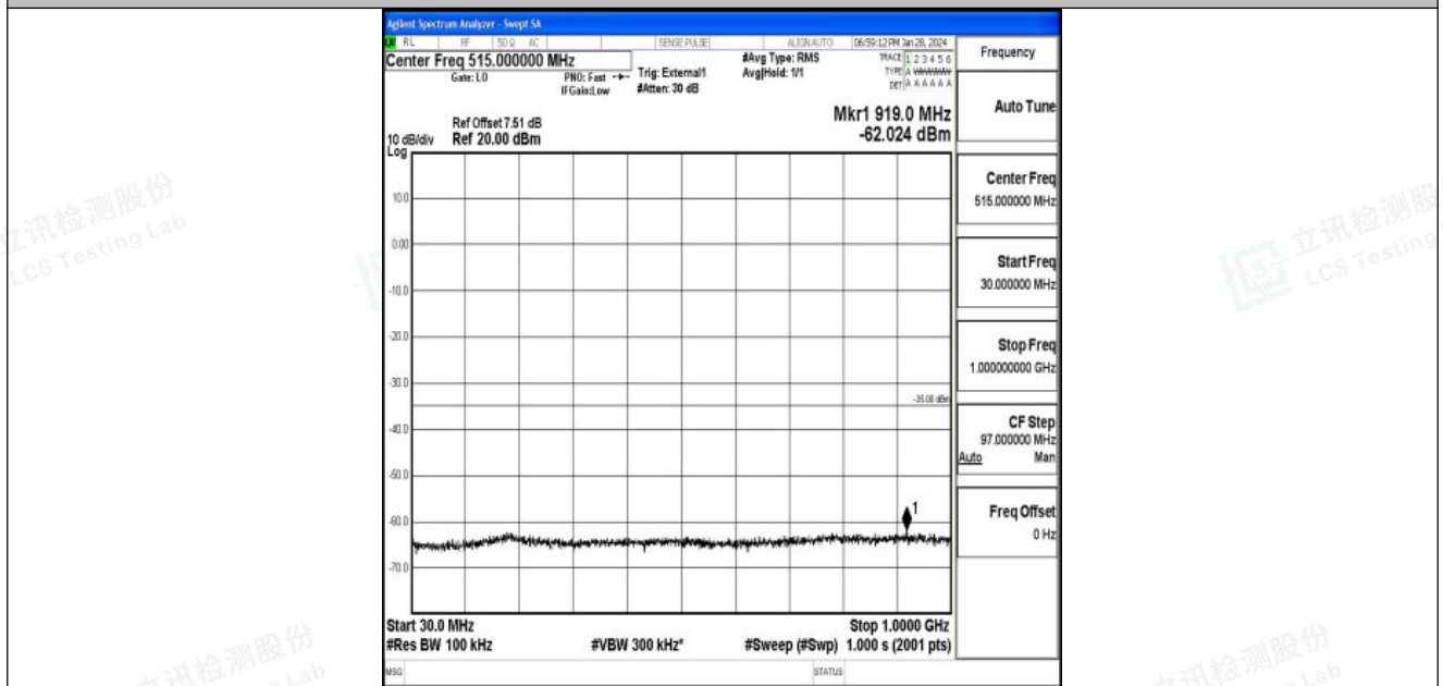
Band41_5MHz_16QAM_41565_1RB#0_30~1000_30~1000
