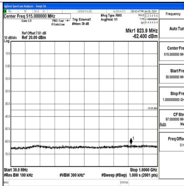
Band41_10MHz_QPSK_39700_1RB#0_30~1000_30~1000
