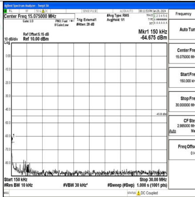
Band41_20MHz_16QAM_39750_1RB#0_0.15~30_0.15~30
