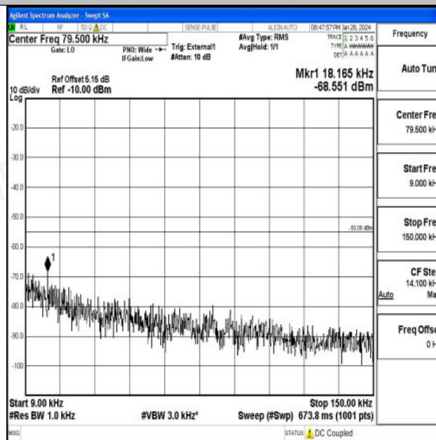
Band41_10MHz_16QAM_40620_1RB#0_0.009~0.15_0.009~0.15
