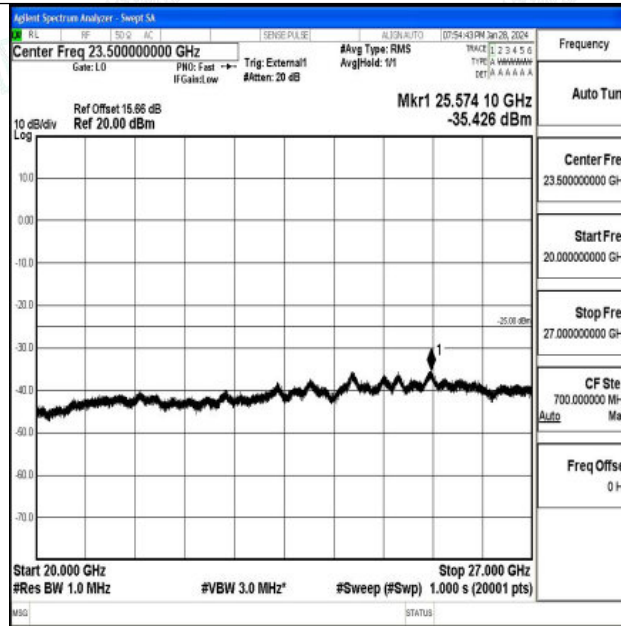
Band41_15MHz_QPSK_41515_1RB#0_20000~27000_20000~27000
