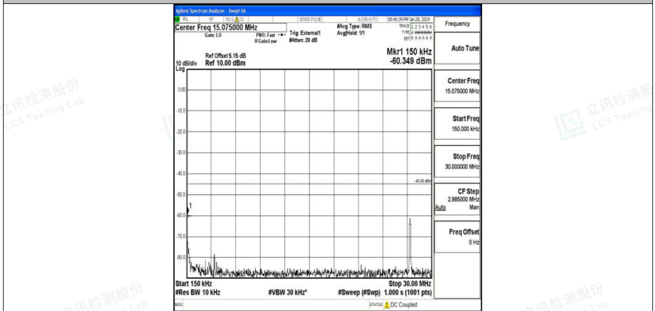
Band41_10MHz_QPSK_40620_1RB#0_0.15~30_0.15~30
