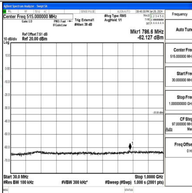
Band41_10MHz_16QAM_40620_1RB#0_30~1000_30~1000
