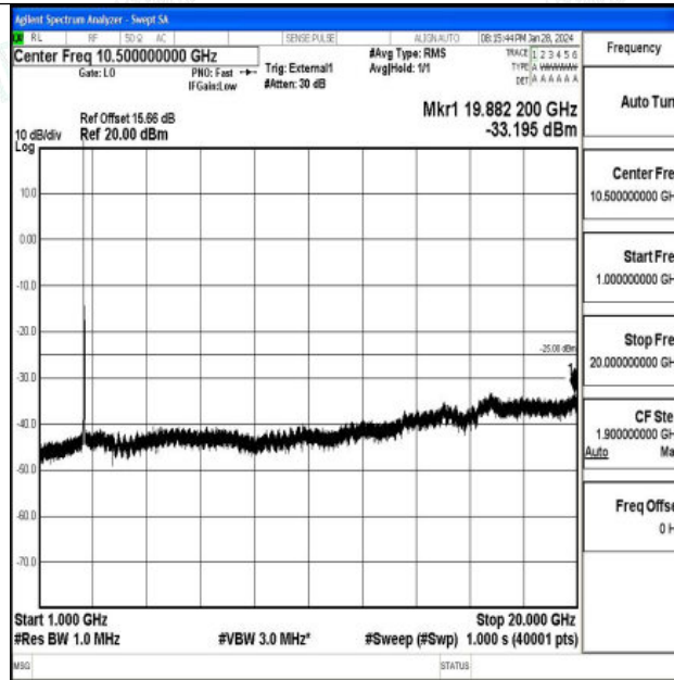
Band41_20MHz_16QAM_40620_1RB#0_1000~20000_1000~20000
