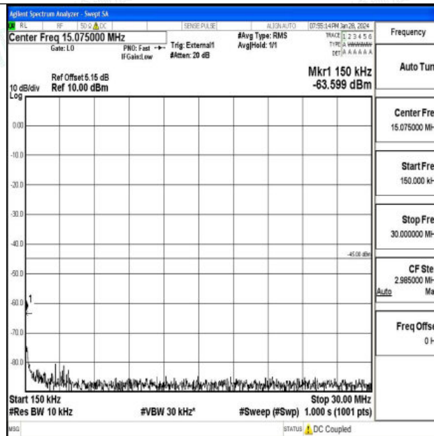
Band41_15MHz_16QAM_41515_1RB#0_0.15~30_0.15~30
