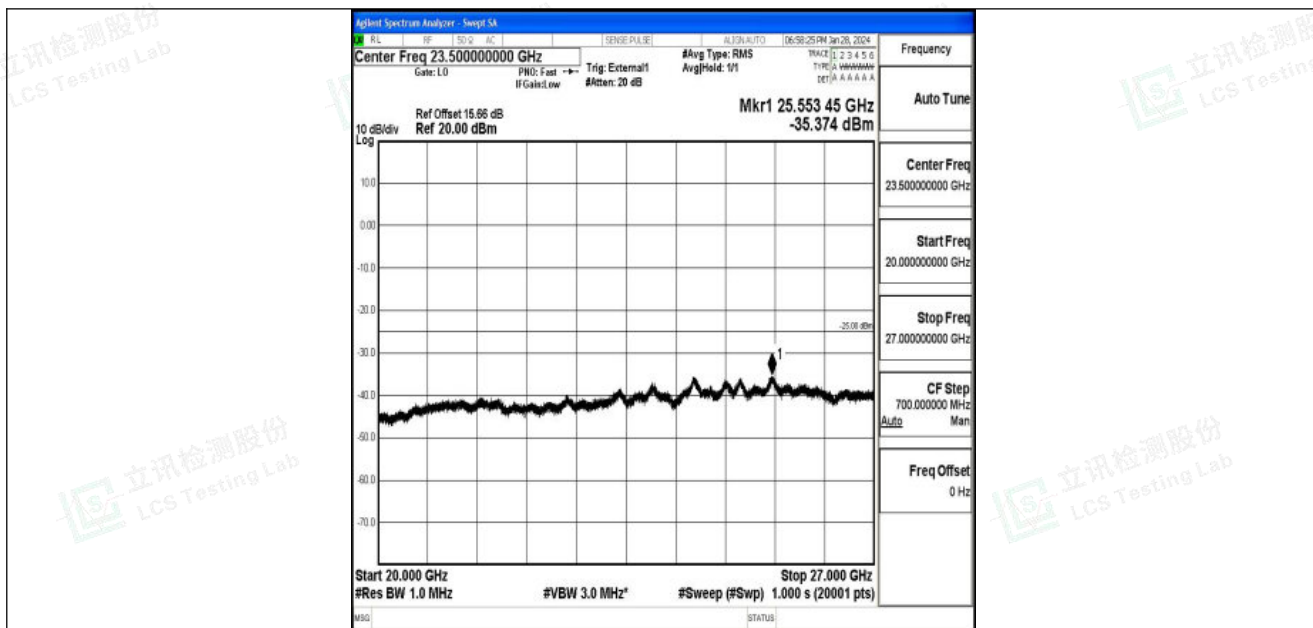
Band41_5MHz_QPSK_41565_1RB#0_20000~27000_20000~27000
