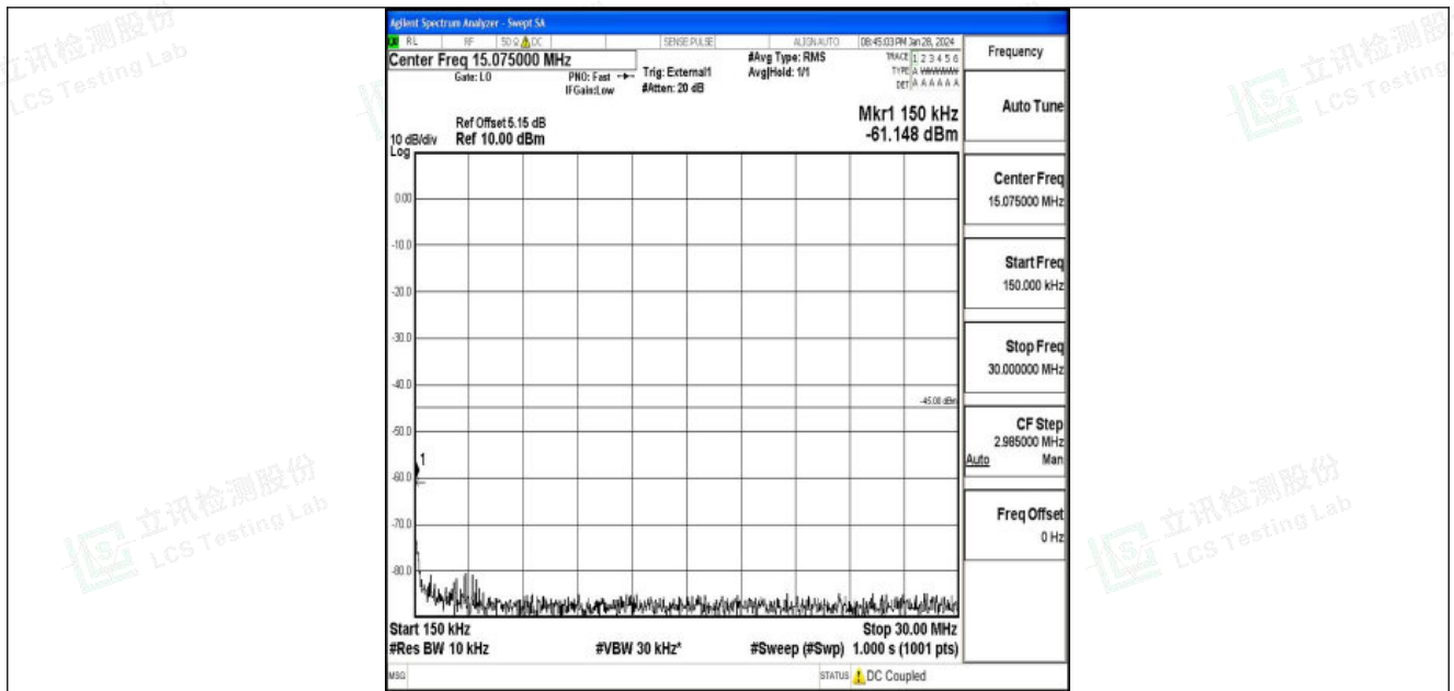
Band41_10MHz_16QAM_39700_1RB#0_0.15~30_0.15~30
