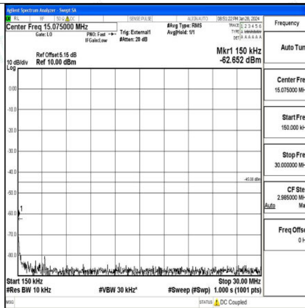
Band41_10MHz_16QAM_41540_1RB#0_0.15~30_0.15~30
