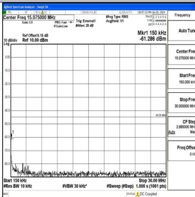
Band41_5MHz_QPSK_41565_1RB#0_0.15~30_0.15~30
