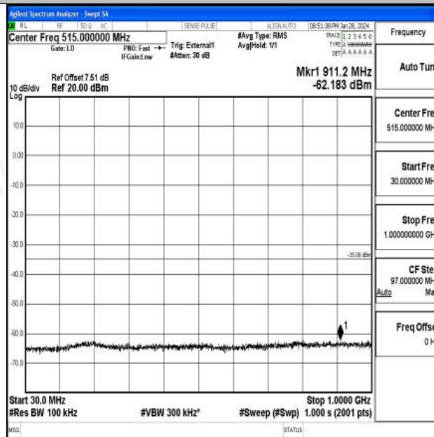
Band41_10MHz_16QAM_41540_1RB#0_30~1000_30~1000
