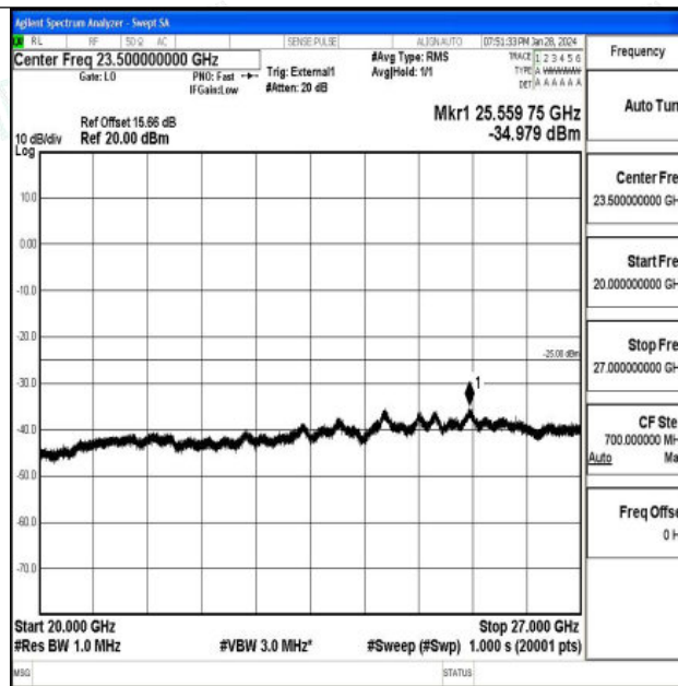
Band41_15MHz_QPSK_40620_1RB#0_20000~27000_20000~27000
