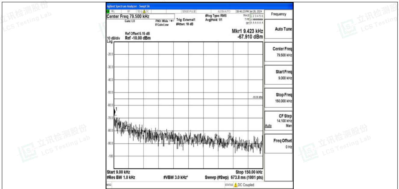
Band41_10MHz_QPSK_40620_1RB#0_0.009~0.15_0.009~0.15
