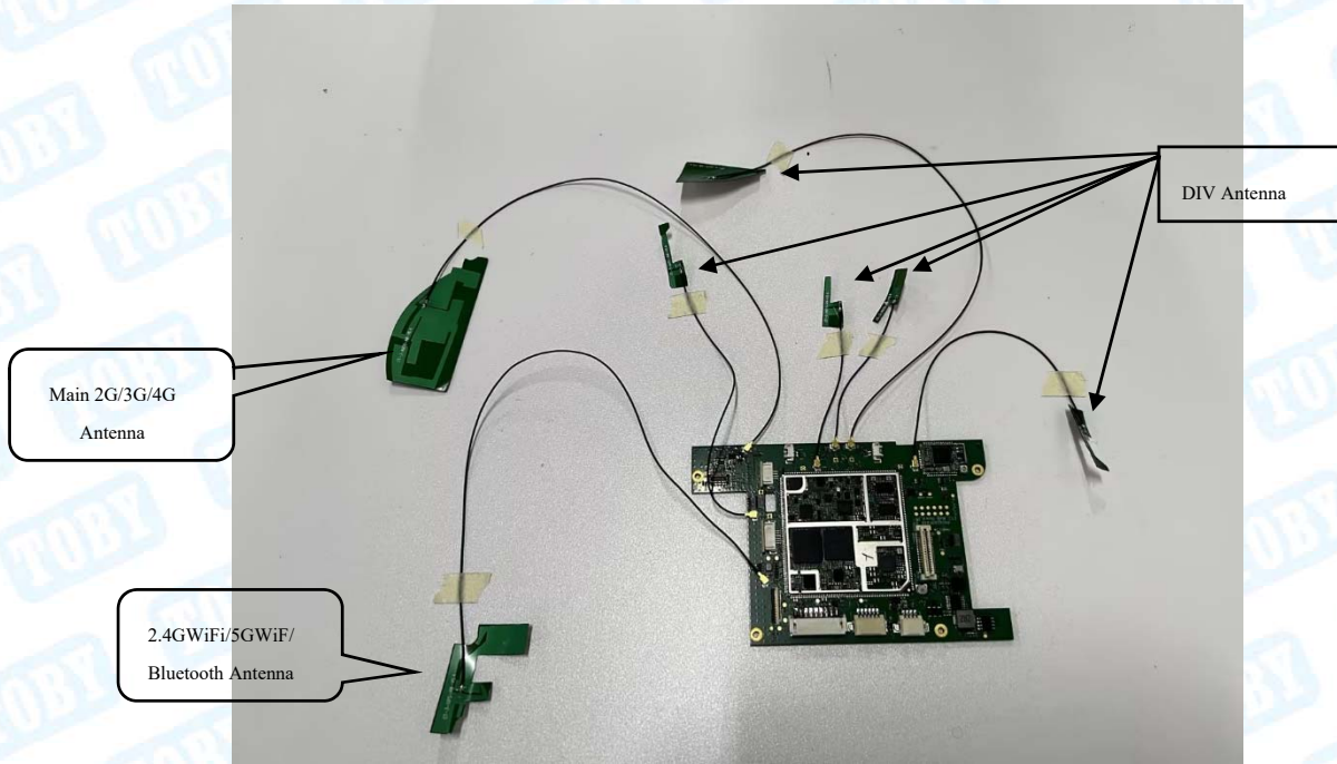
Photo 29 Appearance of PCB
