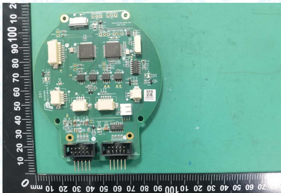
Photo 25 Appearance of PCB
