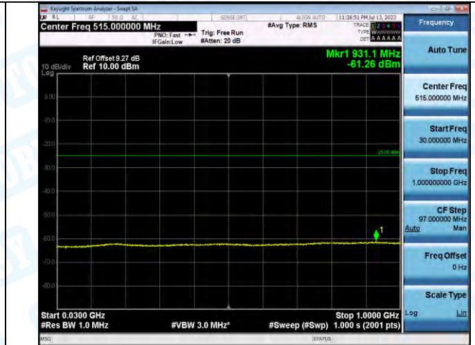
Band7_Band7_5MHz_16QAM_20775_1RB#0_30-1000_30-1000
