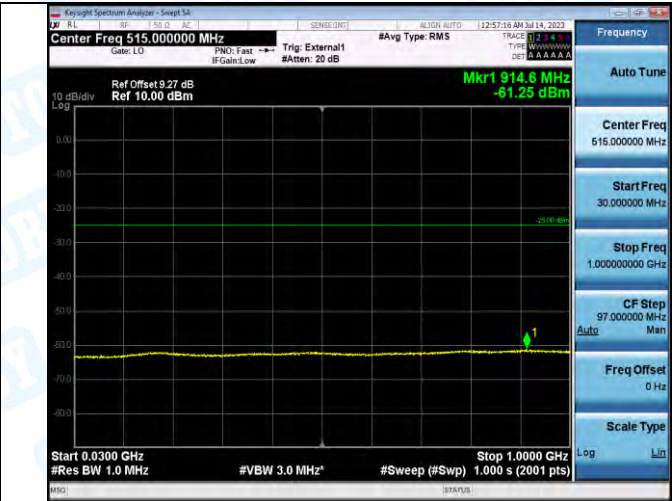
Band41_Band41_5MHz_16QAM_39675_1RB#0_30-1000_30-1000
