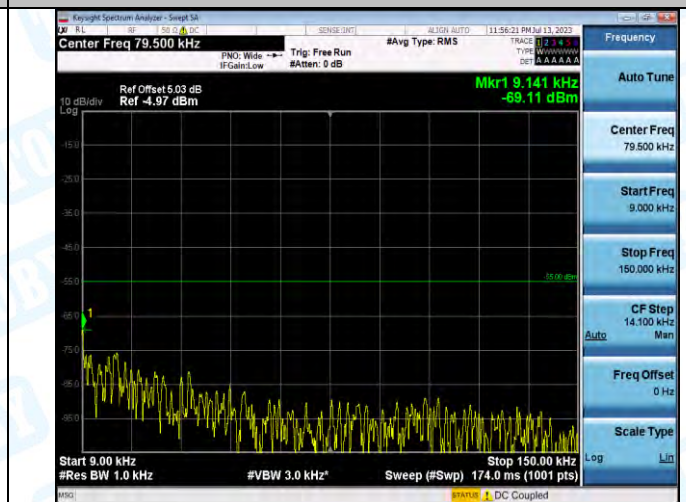
Band7_Band7_20MHz_QPSK_21100_1RB#0_0.009-0.15_0.009-0.15
