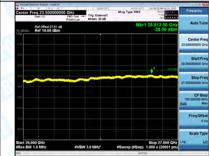
Band41_Band41_5MHz_16QAM_41565_1RB#0_20000~27000_20000~27000
