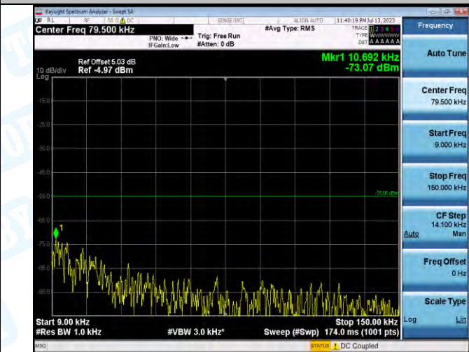
Band7_ Band7_5MHz_16QAM_21100_1RB#0_0.009-0.15_0.009-0.15
