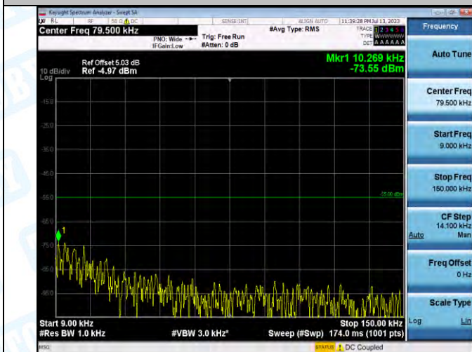
Band7_Band7_5MHz_QPSK_21100_1RB#0_0.009-0.15_0.009-0.15
