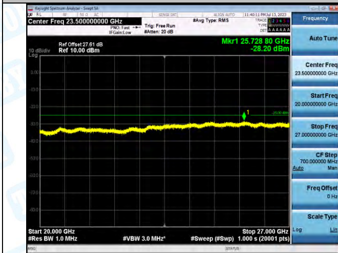
Band7_ Band7_5MHz_QPSK_21100_1RB#0_20000-27000_20000-27000
