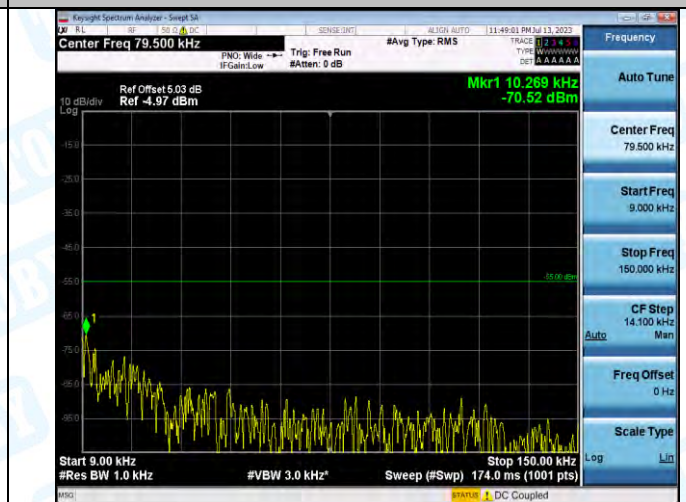
Band7_Band7_15MHz_QPSK_20825_1RB#0_0.009~0.15_0.009~0.15
