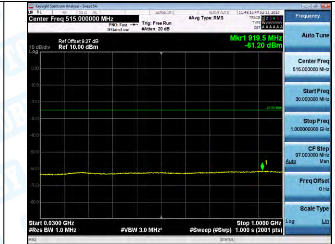
Band7_Band7_15MHz_QPSK_20825_1RB#0_30~1000_30~1000
