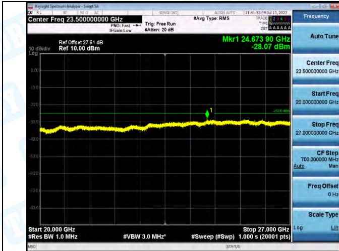
Band7_ Band7_ 5MHz_QPSK_21425_1RB#0_20000-27000_20000-27000
