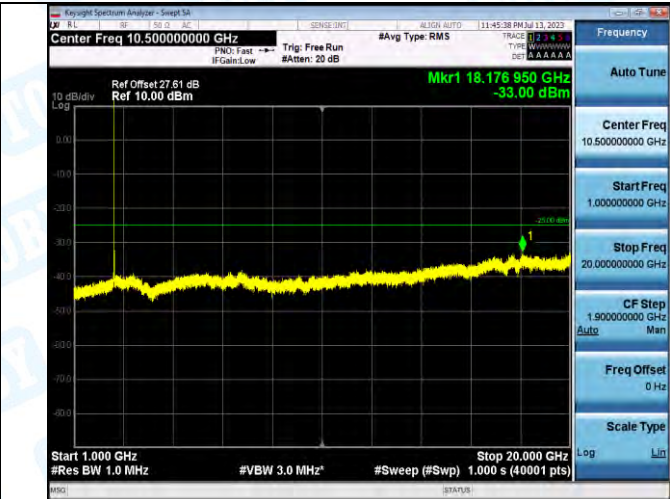
Band7_Band7_10MHz_QPSK_21100_1RB#0_1000~20000_1000~20000
