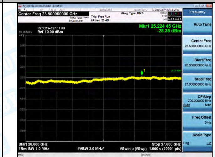
Band7_Band7_15MHz_16QAM_20825_1RB#0_20000~27000_20000~27000
