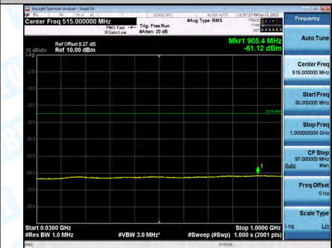
Band7_Band7_20MHz_16QAM_21100_1RB#0_30-1000_30-1000
