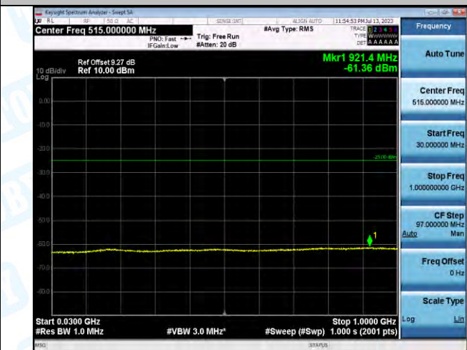
Band7_Band7_20MHz_QPSK_20850_1RB#0_30~1000_30~1000
