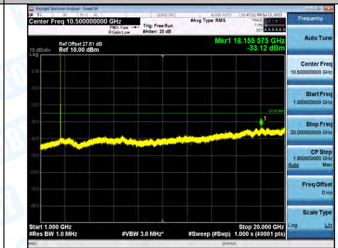
Band7_Band7_10MHz_QPSK_21400_1RB#0_1000~20000_1000~20000
