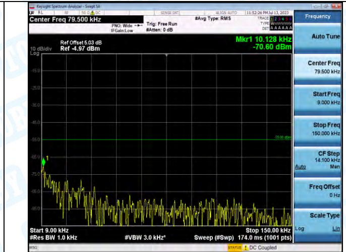
Band7_Band7_15MHz_QPSK_21375_1RB#0_0.009~0.15_0.009~0.15
