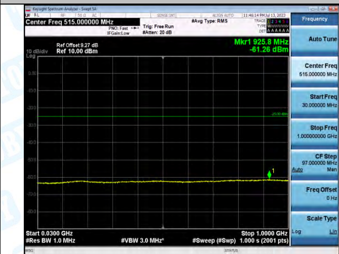
Band7_Band7_10MHz_16QAM_21100_1RB#0_30~1000_30~1000
