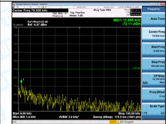
Band7_Band7_20MHz_16QAM_21100_1RB#0_0.009-0.15_0.009-0.15
