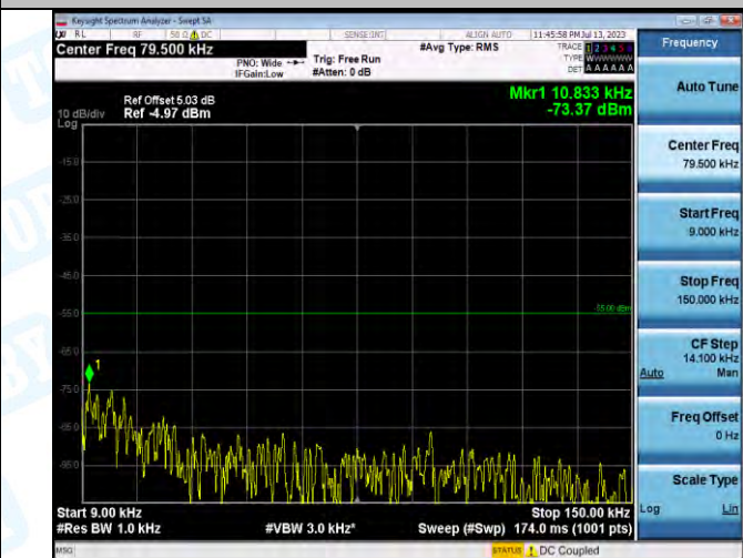
Band7_Band7_10MHz_16QAM_21100_1RB#0_0.009~0.15_0.009~0.15
