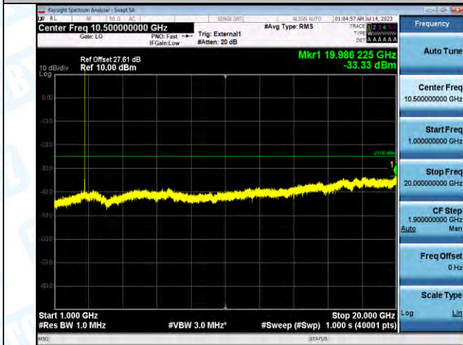
Band41_Band41_5MHz_16QAM_41565_1RB#0_1000~20000_1000~20000
