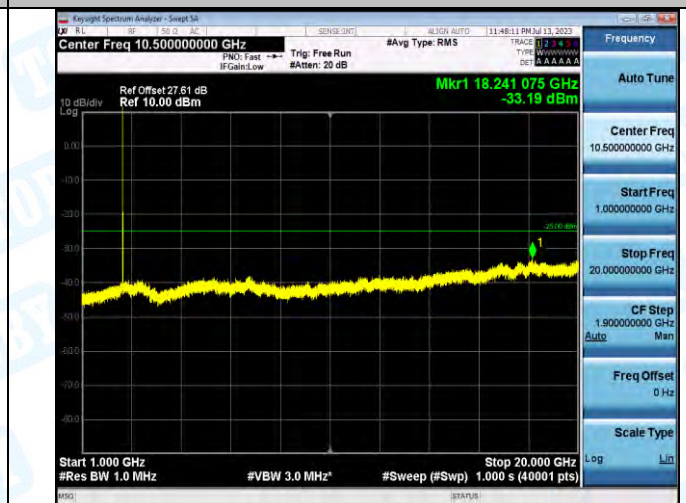
Band7_Band7_10MHz_16QAM_21400_1RB#0_1000~20000_1000~20000
