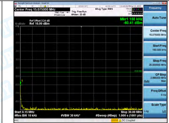
Band7_Band7_10MHz_QPSK_20800_1RB#0_0.15-30_0.15-30
