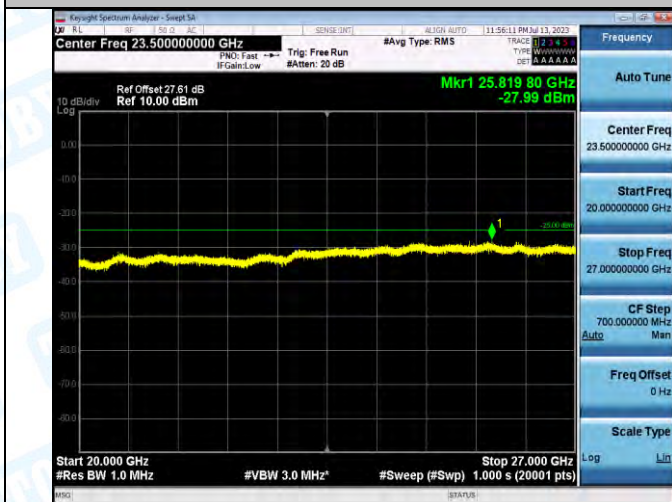
Band7_Band7_20MHz_16QAM_20850_1RB#0_20000-27000_20000-27000
