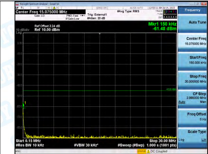
Band41_Band41_5MHz_QPSK_39675_1RB#0_0.15~0.15~30
