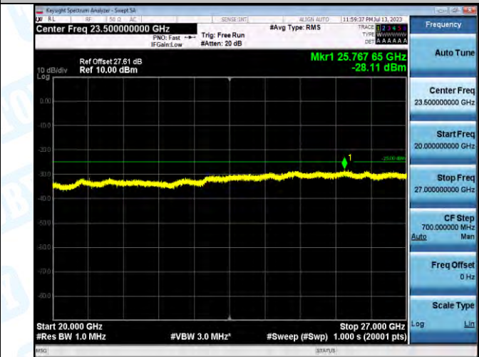
Band7_Band7_20MHz_16QAM_21350_1RB#0_20000-27000_20000-27000
