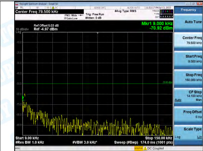
Band7_Band7_15MHz_16QAM_21375_1RB#0_0.009~0.15_0.009~0.15
