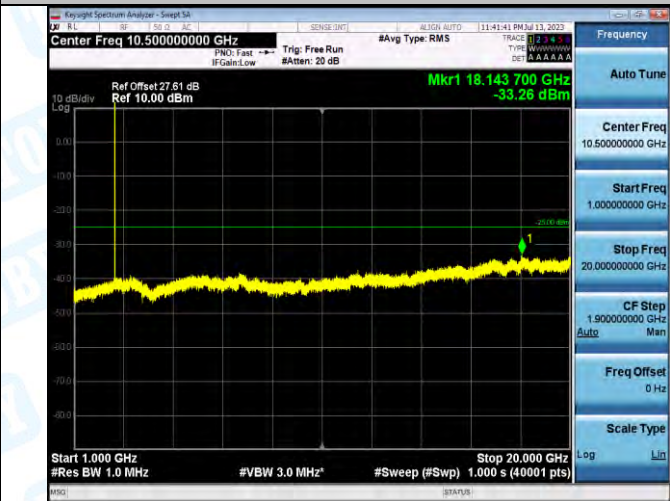
Band7_Band7_5MHz_QPSK_21425_1RB#0_1000-20000_1000-20000
