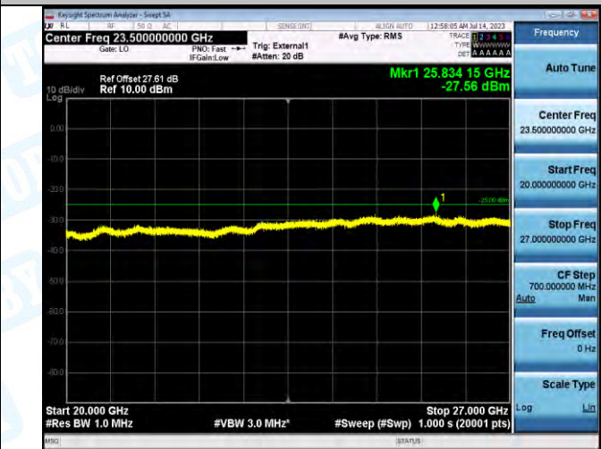
Band41_Band41_5MHz_16QAM_39675_1RB#0_20000-27000_20000-27000
