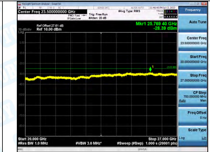
Band7_Band7_10MHz_16QAM_21100_1RB#0_20000~27000_20000~27000
