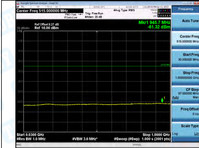
Band7_ Band7_5MHz_QPSK_21100_1RB#0_30-1000_30-1000
