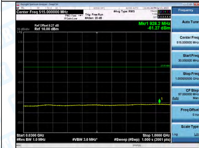
Band7_Band7_5MHz_QPSK_21425_1RB#0_30-1000_30-1000
