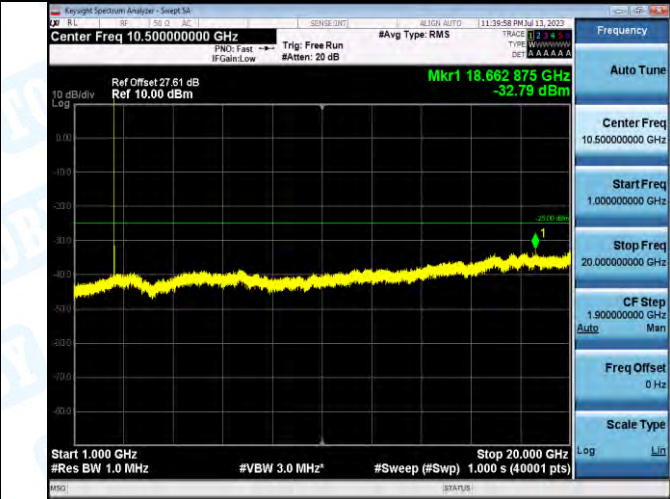
Band7_ Band7_5MHz_QPSK_21100_1RB#0_1000-20000_1000-20000
