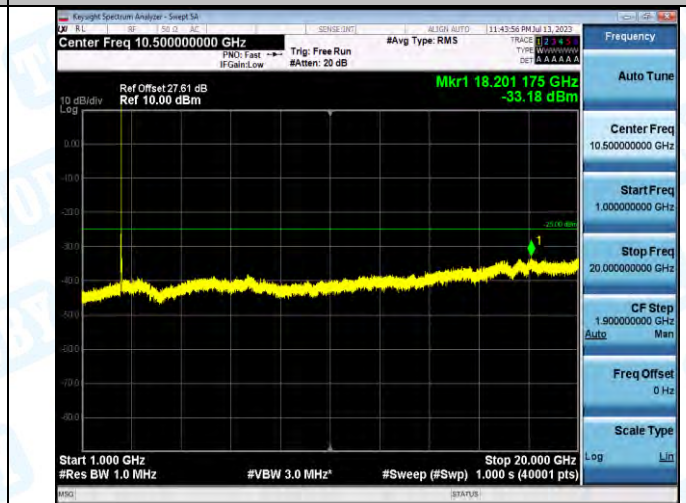
Band7_Band7_10MHz_QPSK_20800_1RB#0_1000-20000_1000-20000
