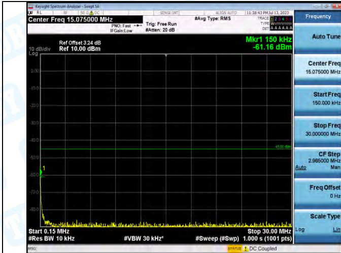
Band7_Band7_5MHz_16QAM_20775_1RB#0_0.15-30_0.15-30
