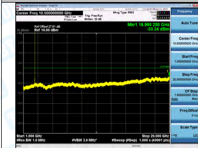
Band7_Band7_5MHz_16QAM_20775_1RB#0_1000-20000_1000-20000
