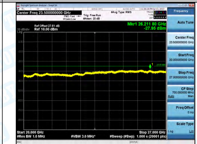
Band7_Band7_5MHz_16QAM_20775_1RB#0_20000-27000_20000-27000
