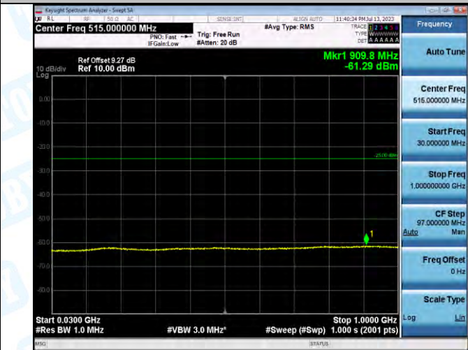
Band7_ Band7_5MHz_16QAM_21100_1RB#0_30-1000_30-1000
