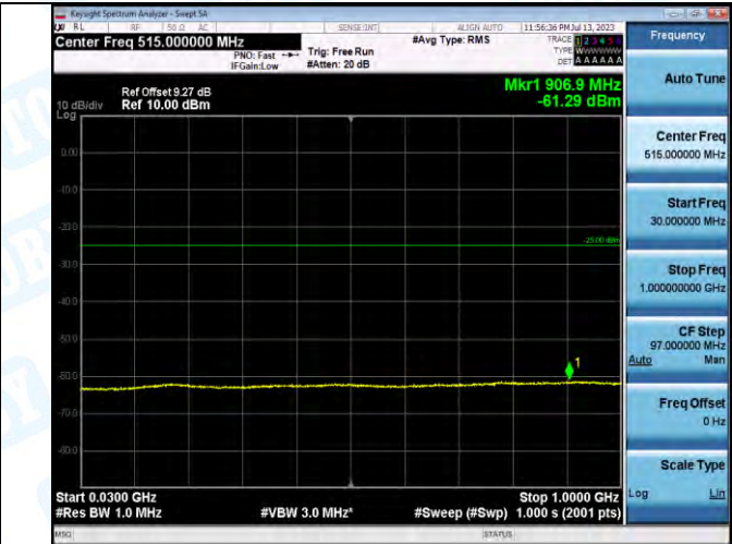
Band7_Band7_20MHz_QPSK_21100_1RB#0_30-1000_30-1000
