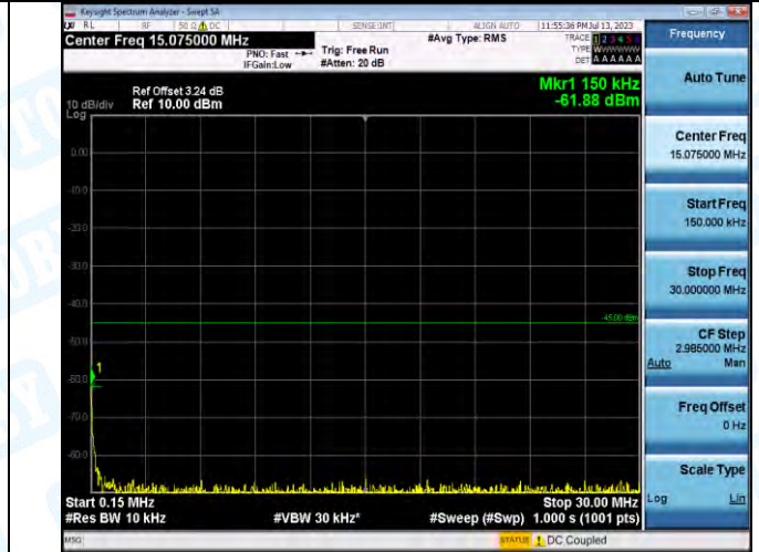
Band7_Band7_20MHz_16QAM_20850_1RB#0_0.15-30_0.15-30
