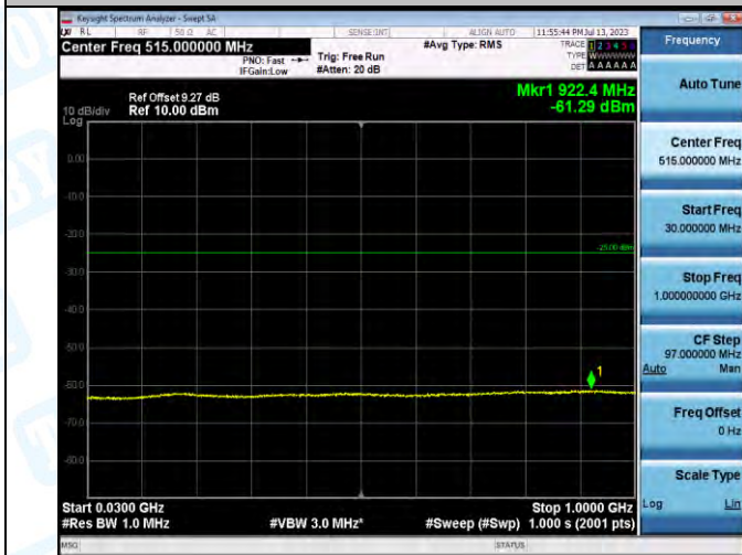
Band7_Band7_20MHz_16QAM_20850_1RB#0_30-1000_30-1000
