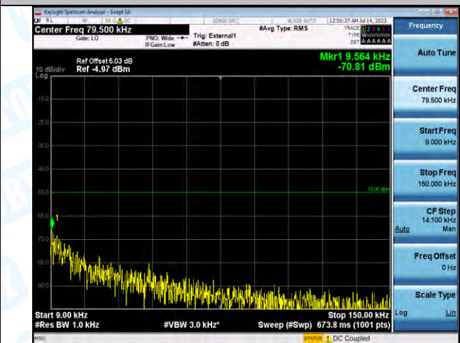
Band41_Band41_5MHz_16QAM_39675_1RB#0_0.009~0.15_0.009~0.15
