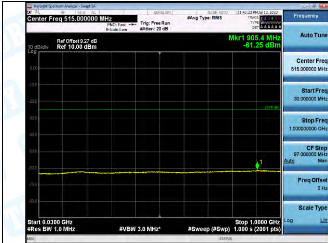
Band7_Band7_10MHz_QPSK_21100_1RB#0_30~1000_30~1000
