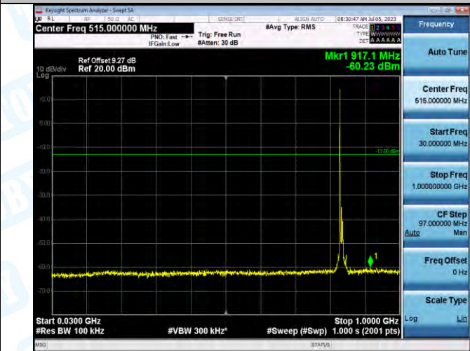
Band5_Band5_10MHz_16QAM_20525_1RB#0_30~1000_30~1000
