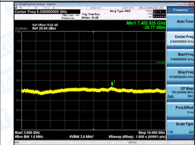
Band5_Band5_5MHz_16QAM_20625_1RB#0_3000-10000_3000-10000
