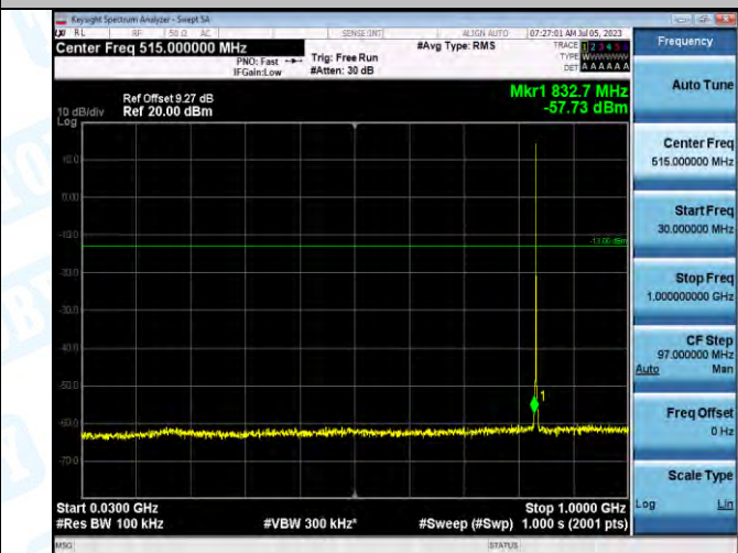
Band5_Band5_1.4MHz_16QAM_20525_1RB#0_30-1000_30-1000
