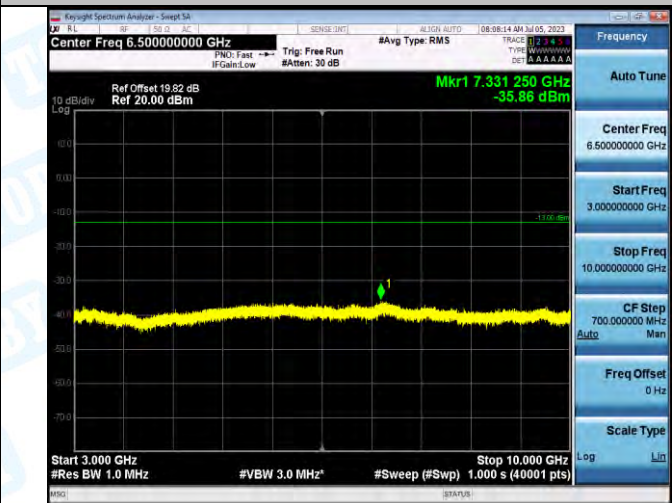
Band5_Band5_5MHz_16QAM_20425_1RB#0_3000~10000_3000~10000
