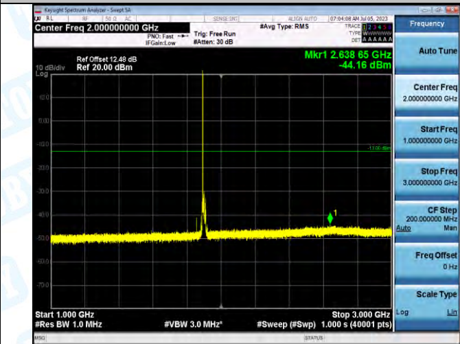
Band2_Band2_20MHz_QPSK_19100_1RB#0_1000-3000_1000-3000
