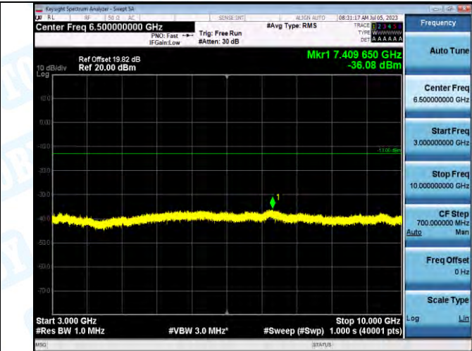
Band5_Band5_10MHz_16QAM_20525_1RB#0_3000-10000_3000-10000
