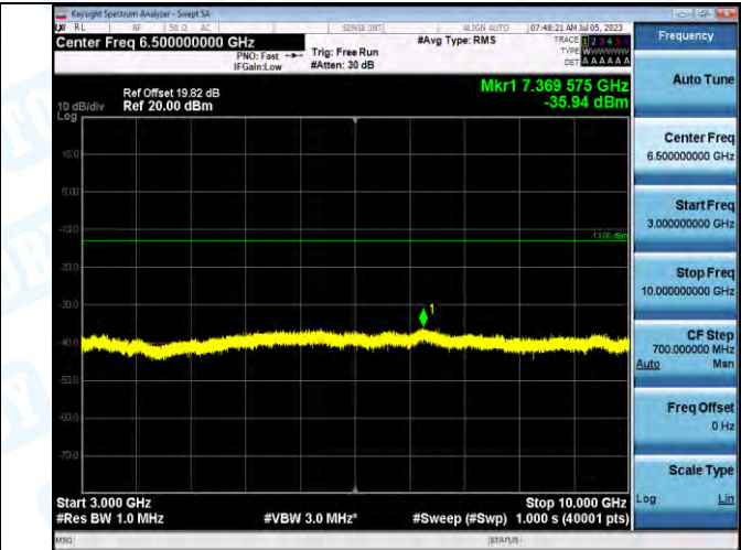
Band5_Band5_3MHz_16QAM_20525_1RB#0_3000~10000_3000~10000
