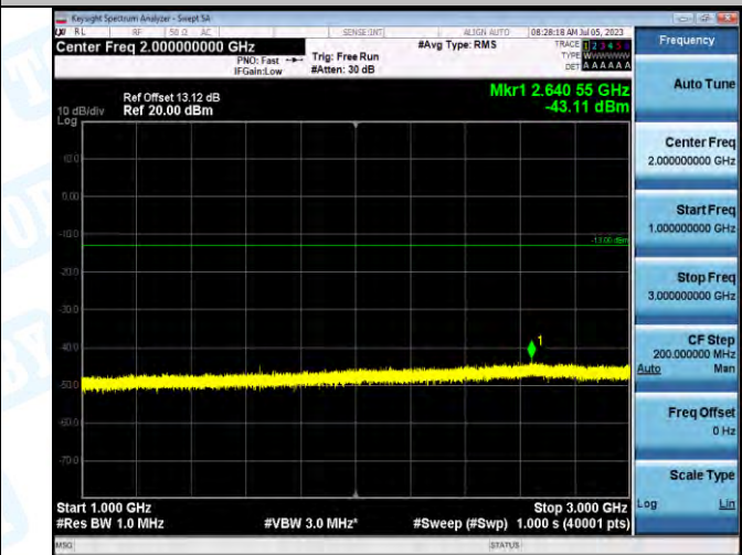
Band5_Band5_10MHz_QPSK_20450_1RB#0_1000-3000_1000-3000
