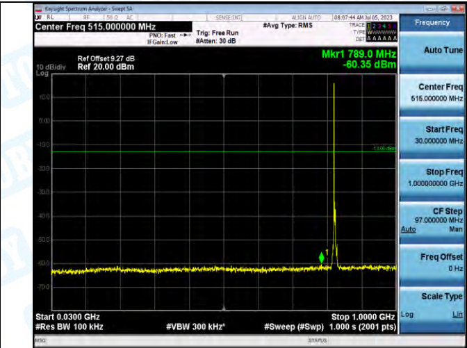
Band5_Band5_5MHz_16QAM_20425_1RB#0_30~1000_30~1000
