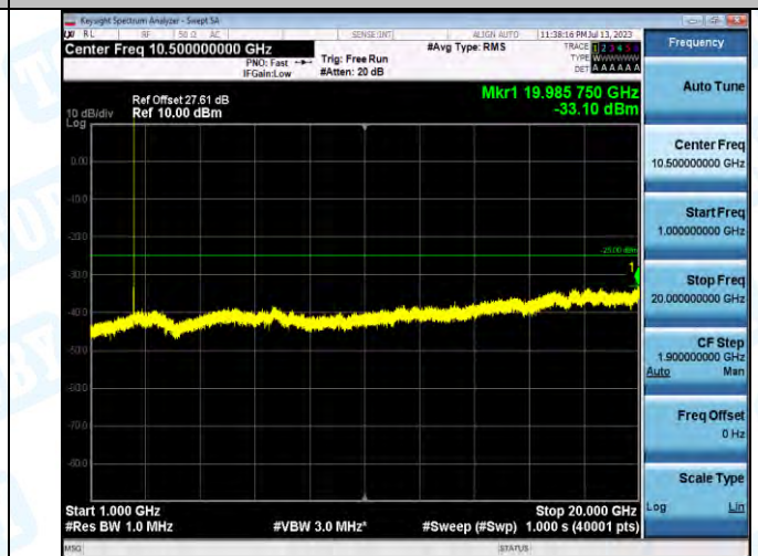
Band7_Band7_5MHz_QPSK_20775_1RB#0_1000-20000_1000-20000
