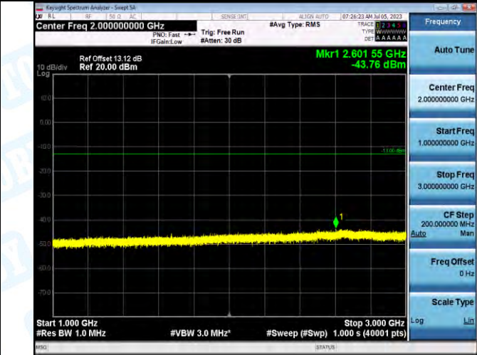
Band5_Band5_1.4MHz_QPSK_20525_1RB#0_1000-3000_1000-3000
