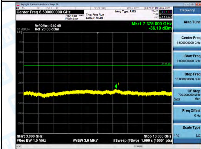
Band5_Band5_10MHz_QPSK_20450_1RB#0_3000-10000_3000-10000
