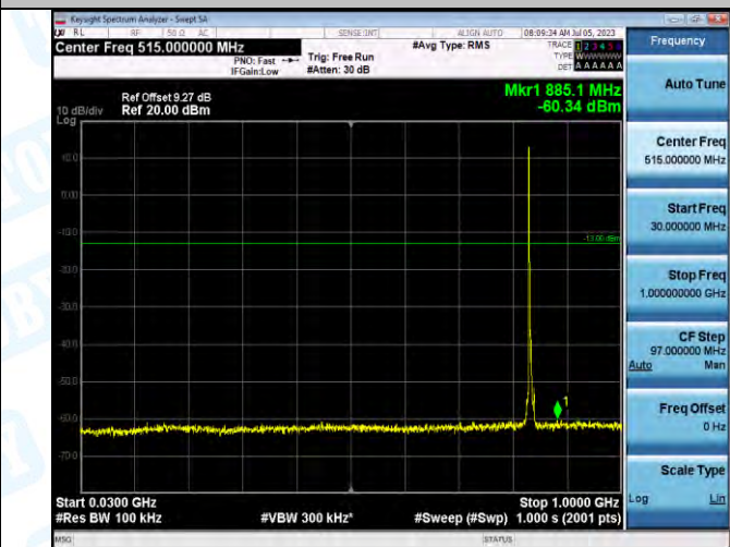
Band5_Band5_5MHz_16QAM_20525_1RB#0_30-1000_30-1000
