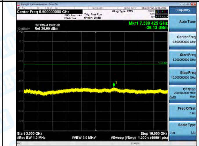
Band5_Band5_10MHz_16QAM_20600_1RB#0_3000-10000_3000-10000
