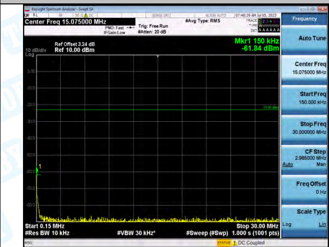
Band5_Band5_3MHz_QPSK_20635_1RB#0_0.15~30_0.15~30
