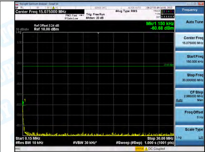
Band5_Band5_10MHz_QPSK_20450_1RB#0_0.15-30_0.15-30
