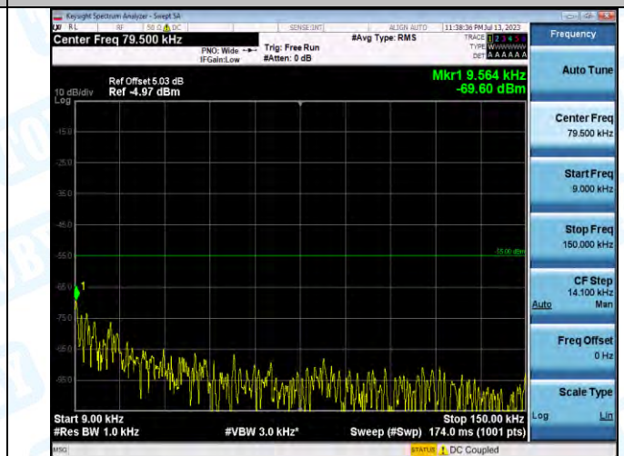
Band7_Band7_5MHz_16QAM_20775_1RB#0_0.009-0.15_0.009-0.15
