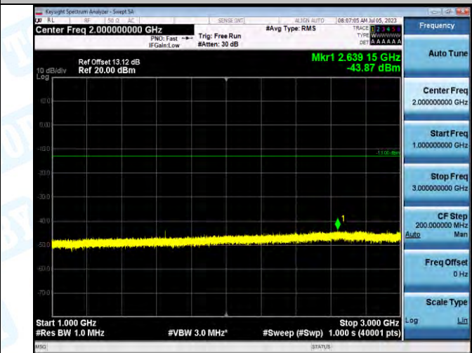
Band5_Band5_5MHz_QPSK_20425_1RB#0_1000-3000_1000-3000
