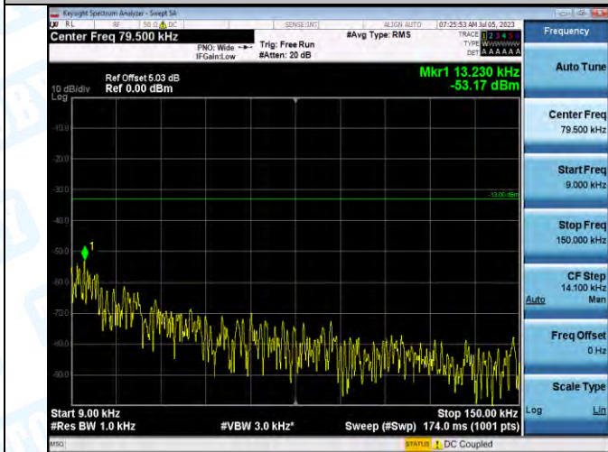
Band5_Band5_1.4MHz_QPSK_20525_1RB#0_0.009-0.15_0.009-0.15
