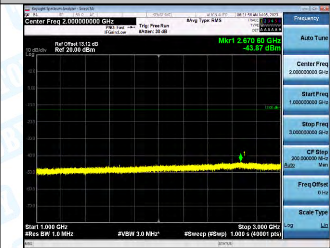
Band5_Band5_10MHz_QPSK_20600_1RB#0_1000-3000_1000-3000
