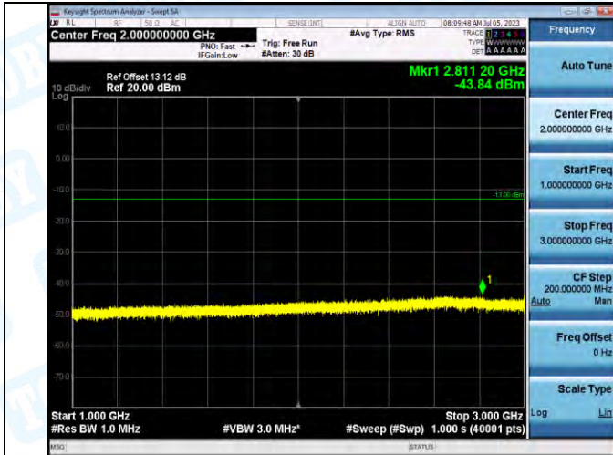
Band5_Band5_5MHz_16QAM_202525_1RB#0_1000-3000_1000-3000
