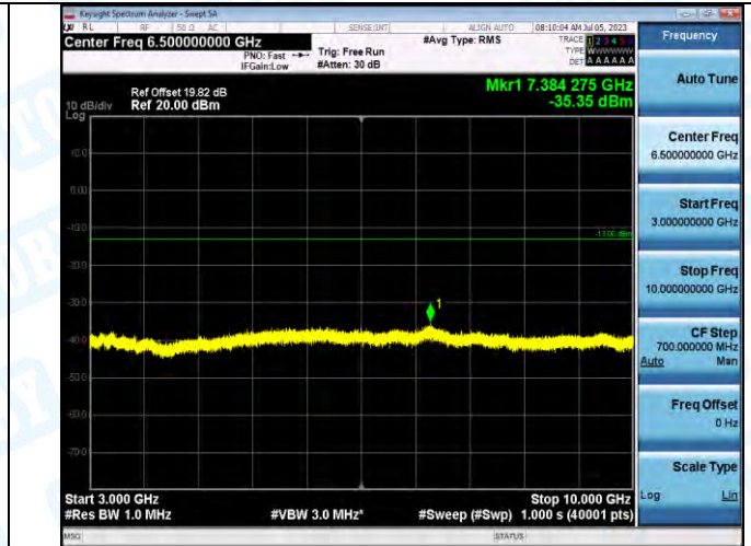
Band5_Band5_5MHz_16QAM_202525_1RB#0_3000-10000_3000-10000
