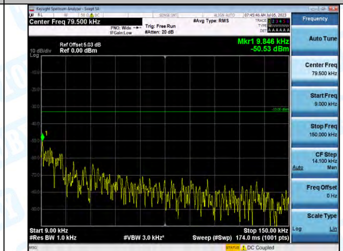
Band5_Band5_3MHz_16QAM_20415_1RB#0_0.009-0.15_0.009-0.15
