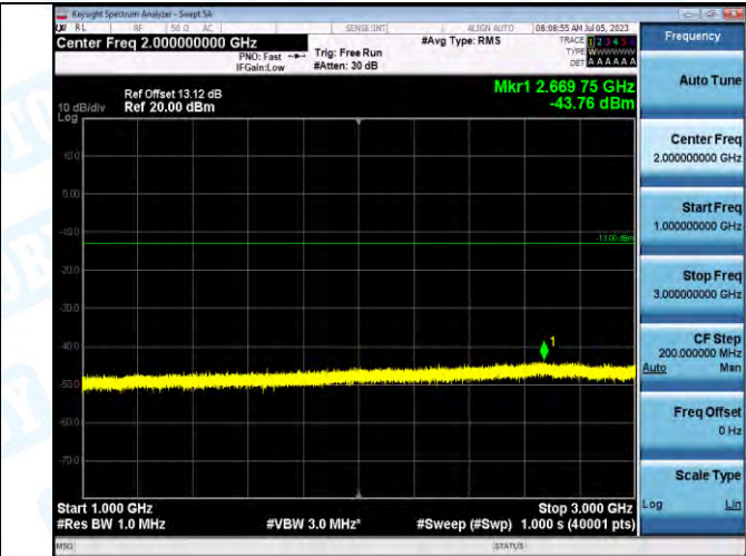
Band5_Band5_5MHz_QPSK_20525_1RB#0_1000-3000_1000-3000
