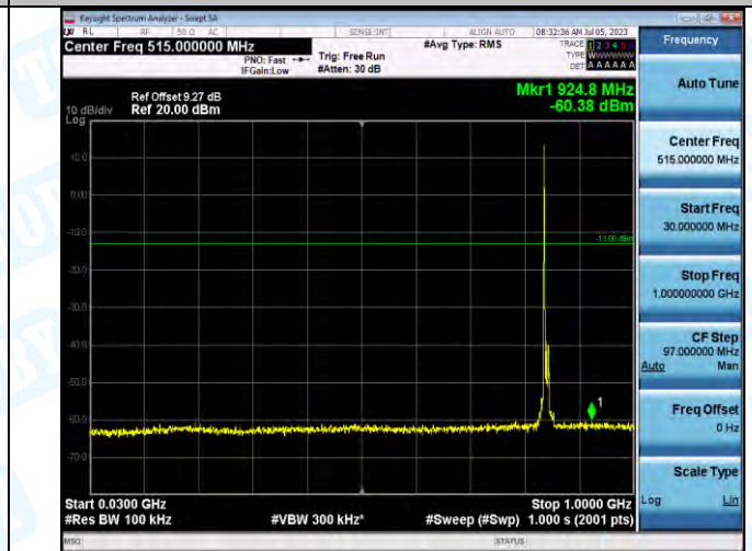
Band5_Band5_10MHz_16QAM_20600_1RB#0_30-1000_30-1000
