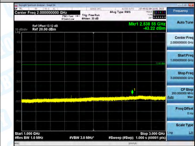
Band5_Band5_3MHz_QPSK_20635_1RB#0_1000~3000_1000~3000
