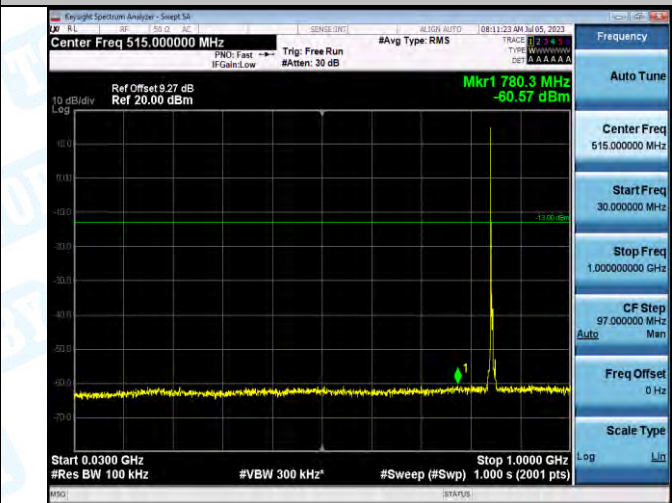
Band5_Band5_5MHz_16QAM_20625_1RB#0_30-1000_30-1000
