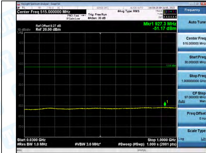
Band2_Band2_20MHz_QPSK_18900_1RB#0_30~1000_30~1000
