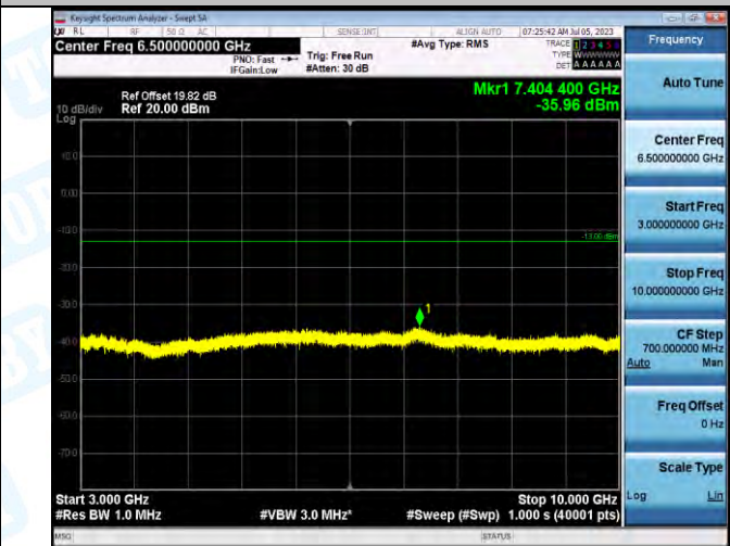
Band5_Band5_1.4MHz_16QAM_20407_1RB#0_3000-10000_3000-10000
