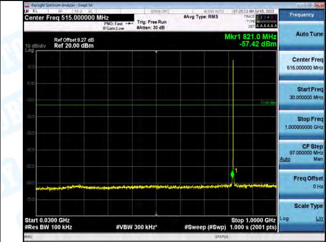
Band5_Band5_1.4MHz_16QAM_20407_1RB#0_30-1000_30-1000
