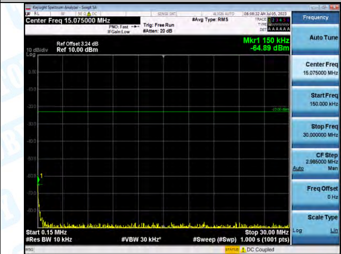
Band5_Band5_5MHz_QPSK_20525_1RB#0_0.15~30_0.15~30
