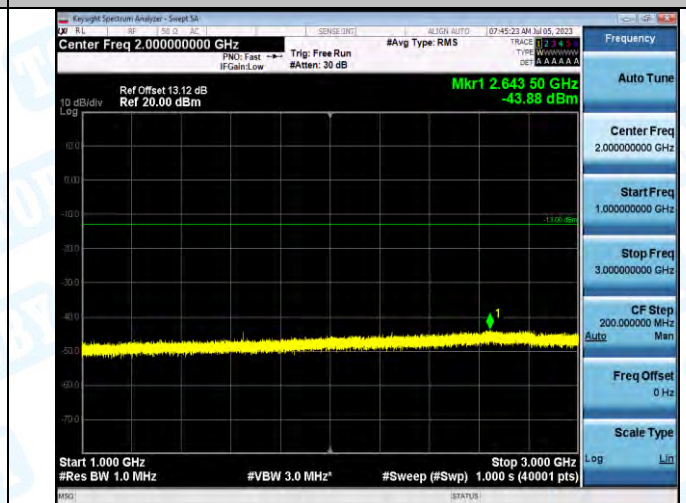
Band5_Band5_3MHz_QPSK_20415_1RB#0_1000-3000_1000-3000
