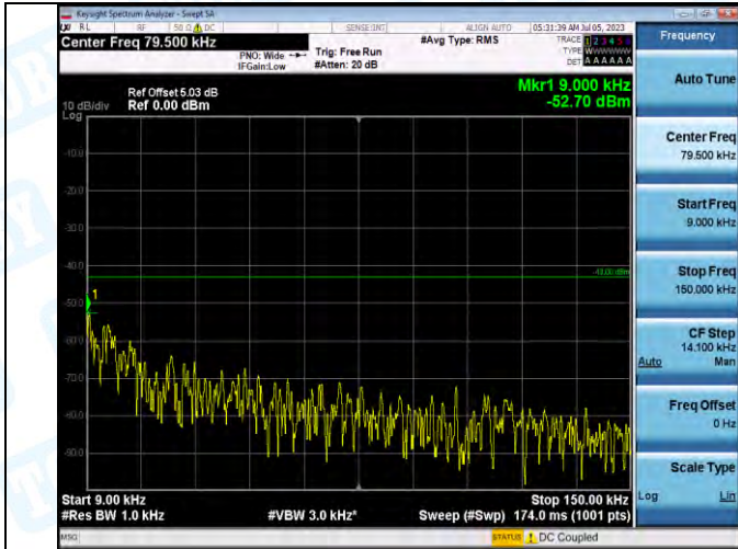
Band2_Band2_3MHz_QPSK_18615_1RB#0_0.009-0.15_0.009-0.15
