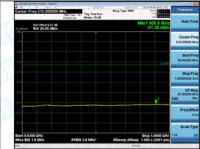
Band2_Band2_3MHz_16QAM_18615_1RB#0_30~1000_30~1000
