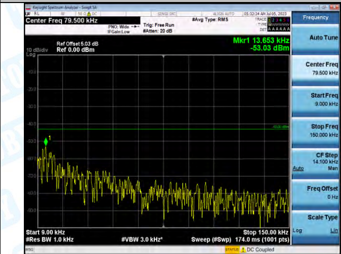
Band2_Band2_3MHz_16QAM_18615_1RB#0_0.009-0.15_0.009-0.15
