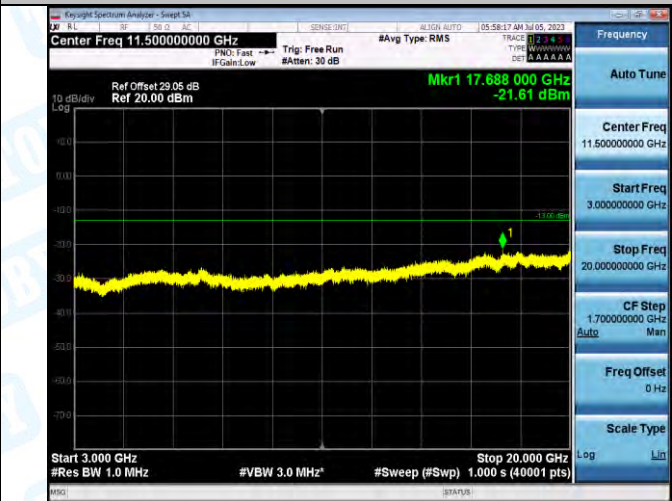
Band2_Band2_5MHz_16QAM_19175_1RB#0_3000-20000_3000-20000
