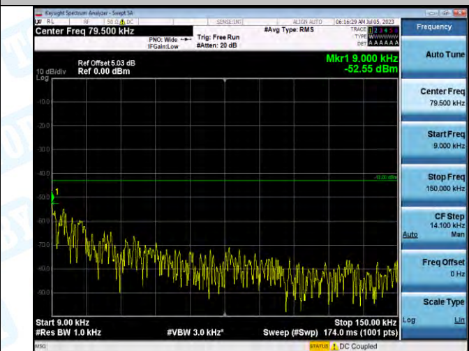
Band2_Band2_10MHz_16QAM_18900_1RB#0_0.009~0.15_0.009~0.15
