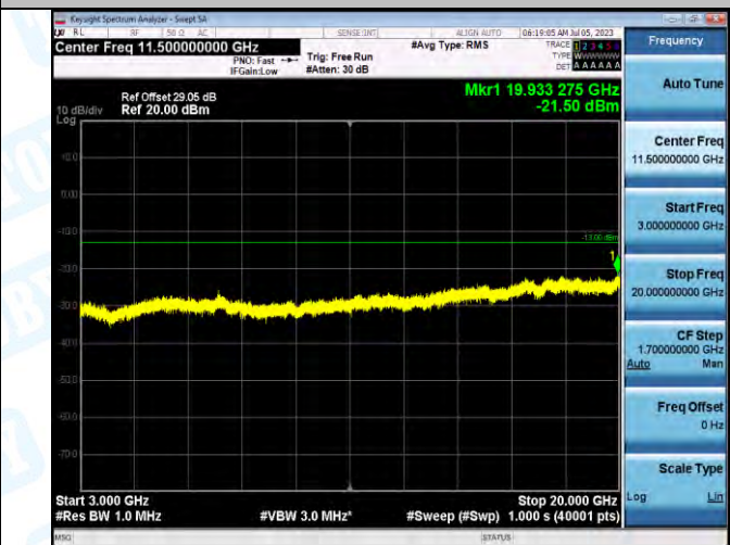
Band2_Band2_10MHz_16QAM_19150_1RB#0_3000-20000_3000-20000
