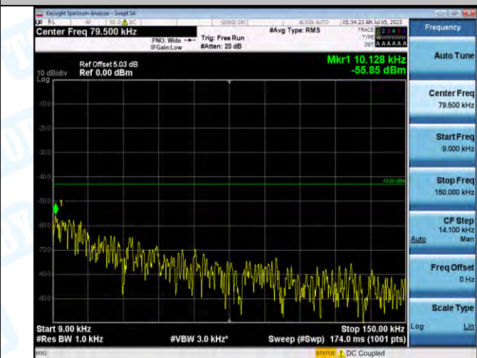
Band2_Band2_3MHz_16QAM_18900_1RB#0_0.009-0.15_0.009-0.15
