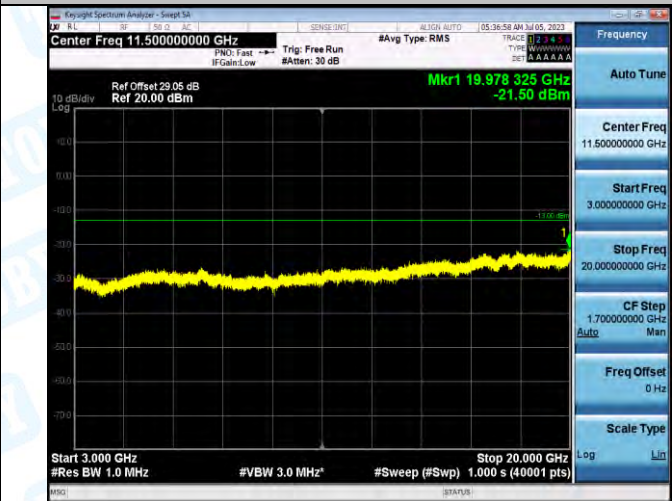
Band2_Band2_3MHz_16QAM_19185_1RB#0_3000-20000_3000-20000
