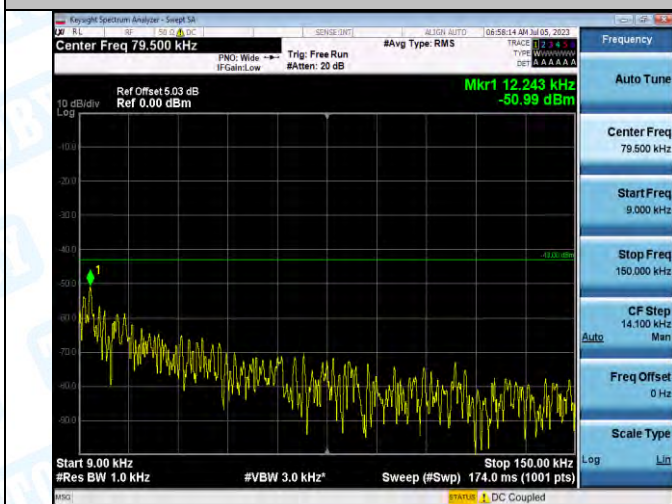
Band2_Band2_20MHz_QPSK_18900_1RB#0_0.009~0.15_0.009~0.15
