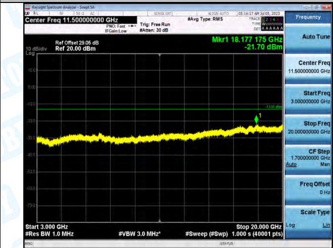
Band2_Band2_1.4MHz_16QAM_19193_1RB#0_3000-20000_3000-20000
