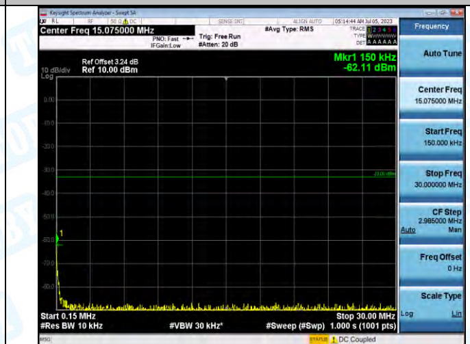
Band2_Band2_1.4MHz_QPSK_19193_1RB#0_0.15-30_0.15-30
