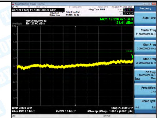
Band2_Band2_15MHz_16QAM_18675_1RB#0_3000~20000_3000~20000
