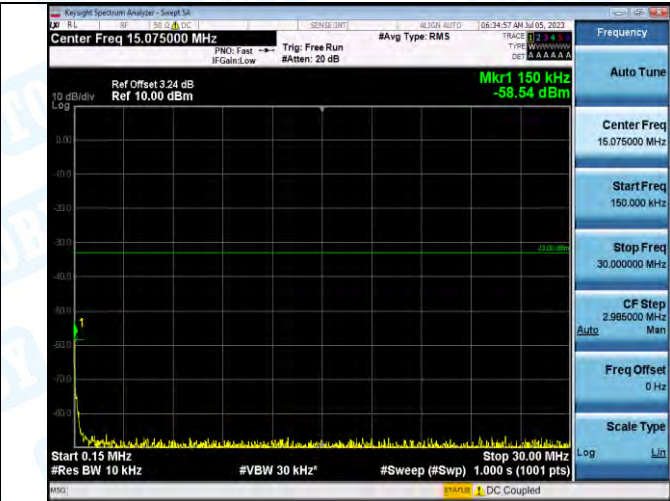
Band2_Band2_15MHz_QPSK_18675_1RB#0_0.15-30_0.15-30
