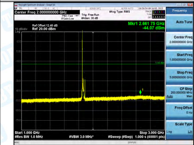
Band2_Band2_20MHz_QPSK_18700_1RB#0_1000-3000_1000-3000
