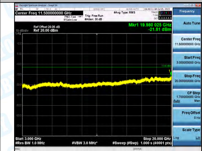
Band2_Band2_15MHz_16QAM_19125_1RB#0_3000-20000_3000-20000
