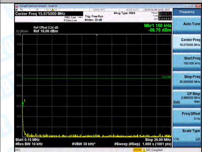
Band2_Band2_5MHz_QPSK_18900_1RB#0_0.15~30_0.15~30
