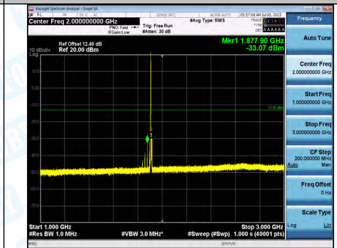
Band2_Band2_5MHz_QPSK_19175_1RB#0_1000-3000_1000-3000
