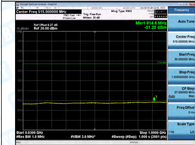
Band2_Band2_15MHz_QPSK_19125_1RB#0_30-1000_30-1000
