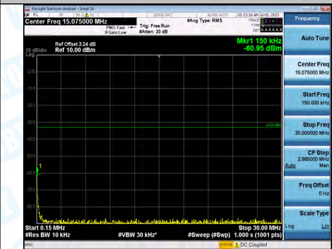
Band2_Band2_3MHz_QPSK_18900_1RB#0_0.15~30_0.15~30
