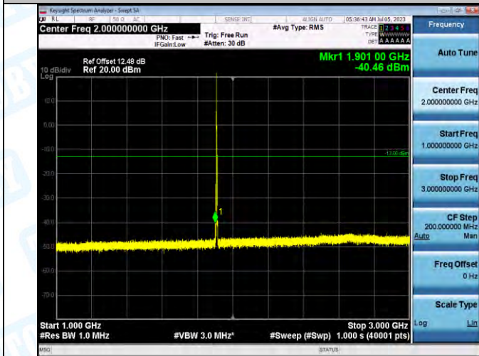
Band2_Band2_3MHz_16QAM_19185_1RB#0_1000-3000_1000-3000
