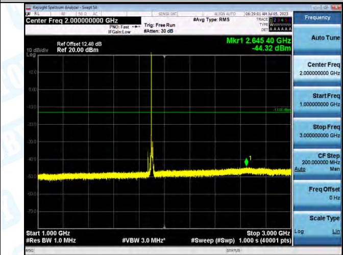
Band2_Band2_15MHz_QPSK_19125_1RB#0_1000-3000_1000-3000
