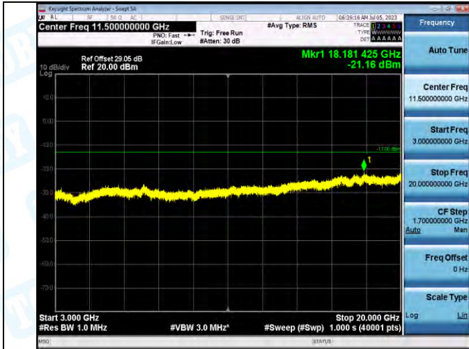
Band2_Band2_15MHz_QPSK_19125_1RB#0_3000-20000_3000-20000
