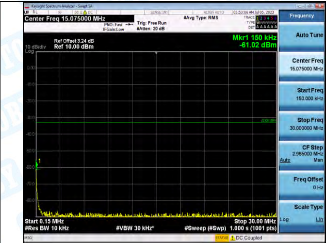
Band2_Band2_5MHz_QPSK_18625_1RB#0_0.15-30_0.15-30
