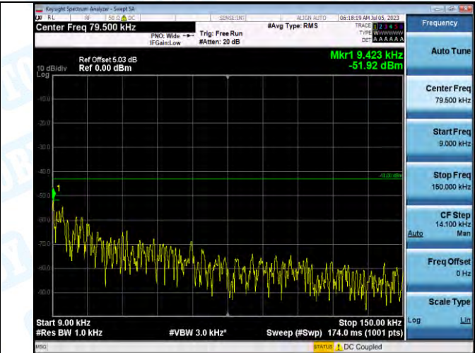
Band2_Band2_10MHz_16QAM_19150_1RB#0_0.009-0.15_0.009-0.15
