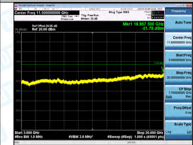
Band2_Band2_5MHz_16QAM_18625_1RB#0_3000~20000_3000~20000
