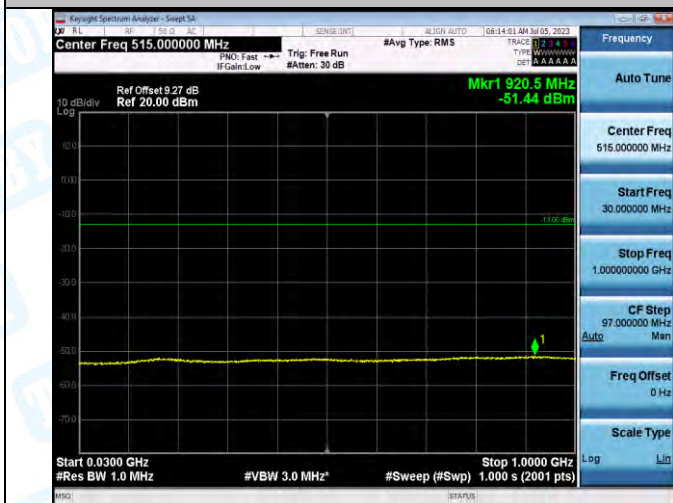
Band2_Band2_10MHz_QPSK_18650_1RB#0_30-1000_30-1000
