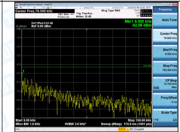
Band2_Band2_5MHz_16QAM_18900_1RB#0_0.009-0.15_0.009-0.15
