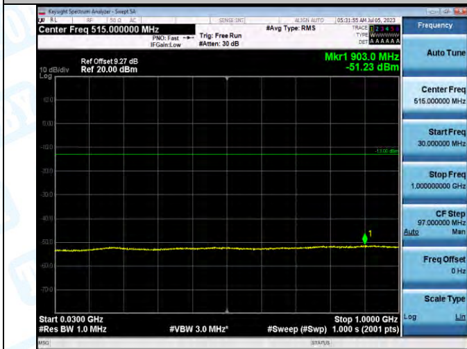
Band2_Band2_3MHz_QPSK_18615_1RB#0_30-1000_30-1000
