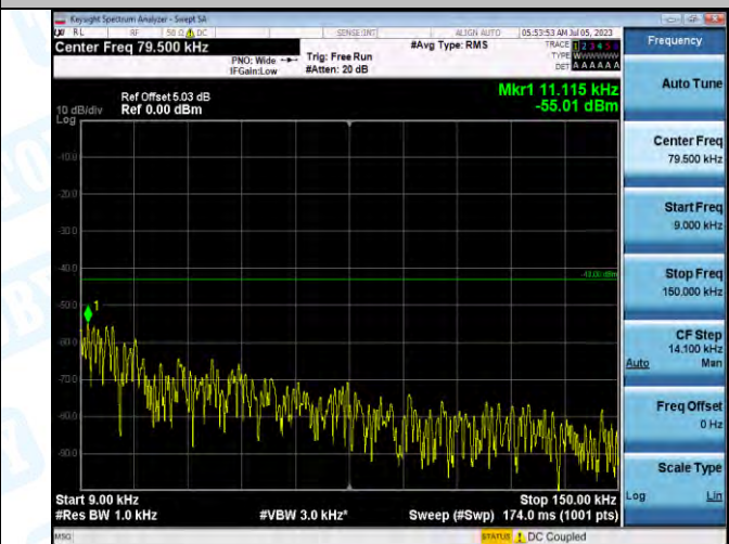
Band2_Band2_5MHz_16QAM_18625_1RB#0_0.009-0.15_0.009-0.15
