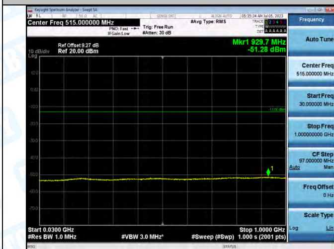
Band2_Band2_3MHz_QPSK_19185_1RB#0_30-1000_30-1000
