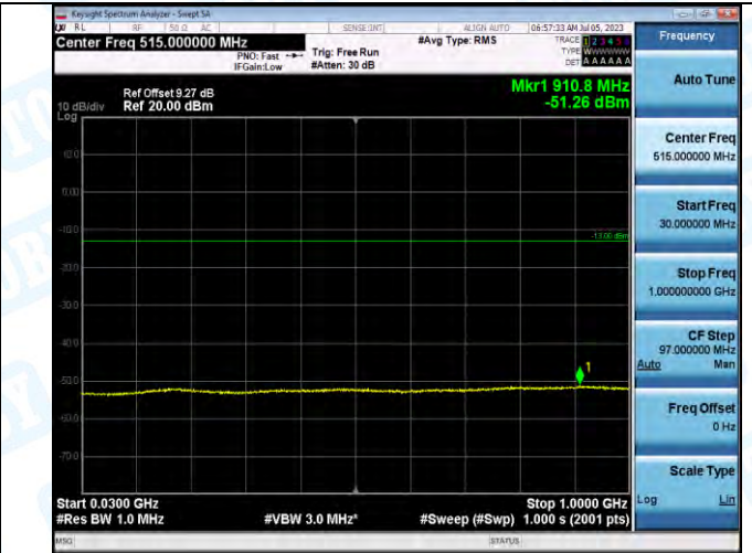
Band2_Band2_20MHz_16QAM_18700_1RB#0_30~1000_30~1000
