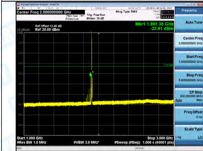
Band2_Band2_5MHz_16QAM_19175_1RB#0_1000-3000_1000-3000
