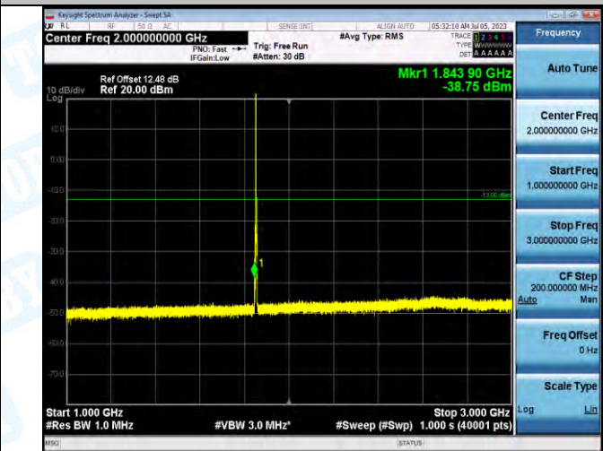
Band2_Band2_3MHz_QPSK_18615_1RB#0_1000-3000_1000-3000
