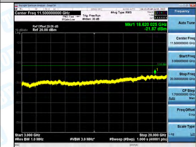
Band2_Band2_10MHz_16QAM_18650_1RB#0_3000~20000_3000~20000
