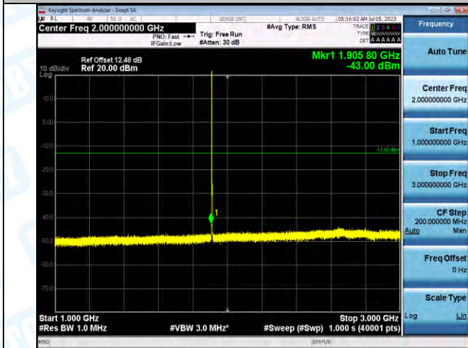
Band2_Band2_1.4MHz_16QAM_19193_1RB#0_1000-3000_1000-3000
