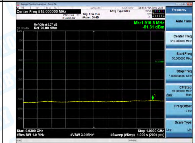
Band2_Band2_5MHz_16QAM_18900_1RB#0_30-1000_30-1000
