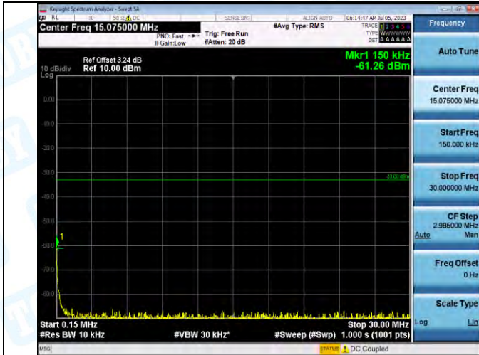
Band2_Band2_10MHz_16QAM_18650_1RB#0_0.15~30_0.15~30
