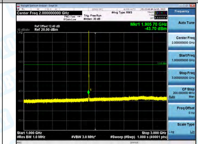
Band2_Band2_1.4MHz_QPSK_19193_1RB#0_1000-3000_1000-3000
