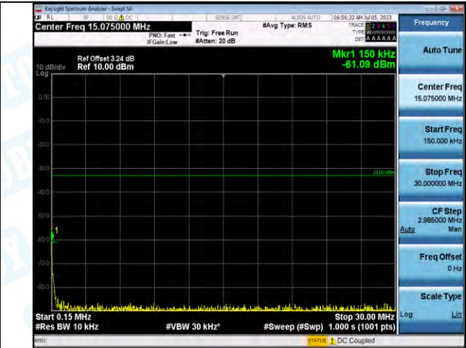
Band2_Band2_20MHz_QPSK_18700_1RB#0_0.15-30_0.15-30
