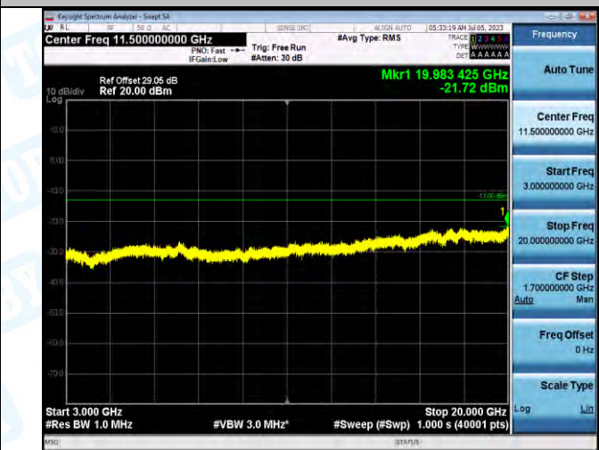
Band2_Band2_3MHz_16QAM_18615_1RB#0_3000~20000_3000~20000
