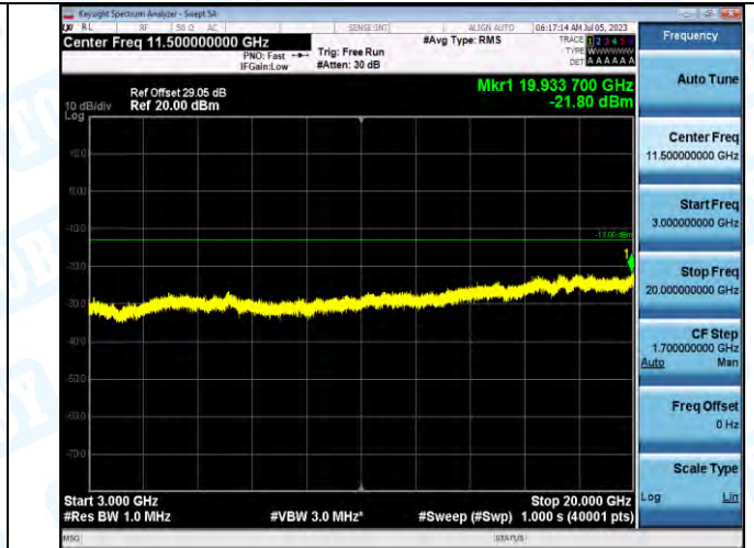
Band2_Band2_10MHz_16QAM_18900_1RB#0_3000-20000_3000-20000
