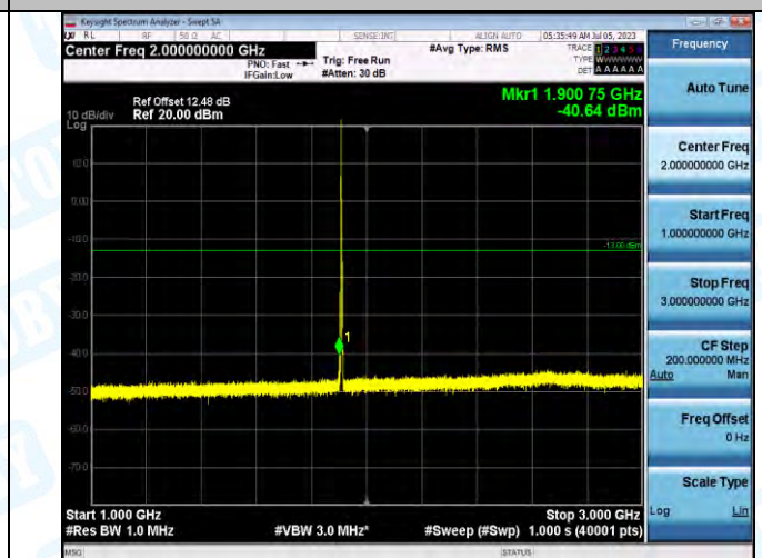
Band2_Band2_3MHz_QPSK_19185_1RB#0_1000-3000_1000-3000
