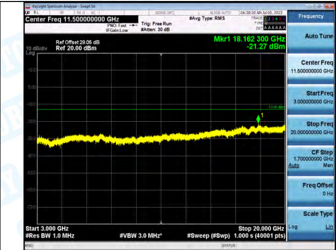
Band2_Band2_15MHz_16QAM_18900_1RB#0_3000-20000_3000-20000
