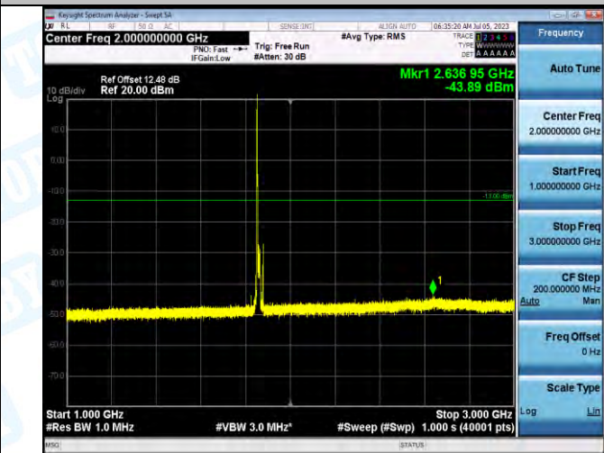
Band2_Band2_15MHz_QPSK_18675_1RB#0_1000-3000_1000-3000
