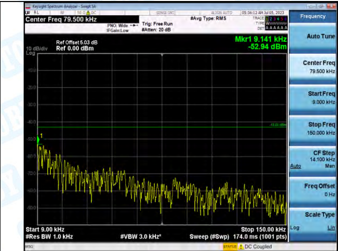
Band2_Band2_3MHz_16QAM_19185_1RB#0_0.009-0.15_0.009-0.15
