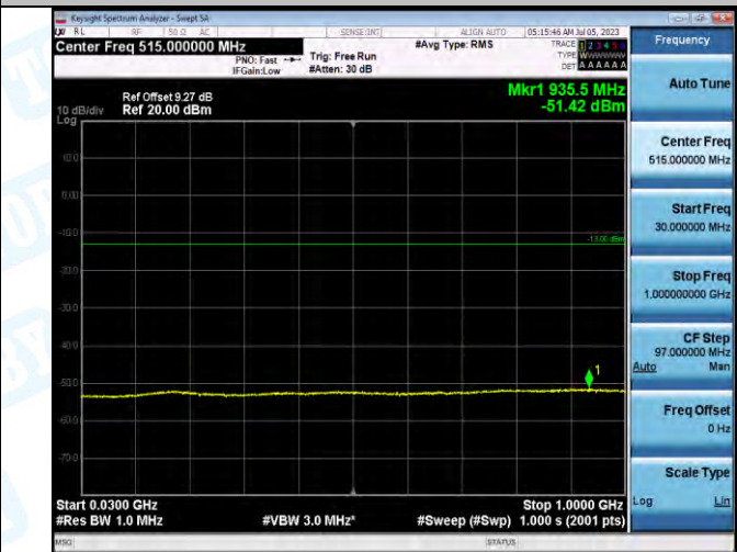
Band2_Band2_1.4MHz_16QAM_19193_1RB#0_30-1000_30-1000
