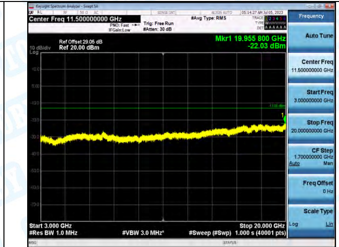
Band2_Band2_1.4MHz_16QAM_18900_1RB#0_3000-20000_3000-20000
