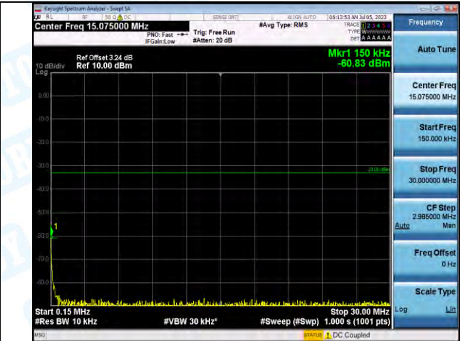
Band2_Band2_10MHz_QPSK_18650_1RB#0_0.15-30_0.15-30
