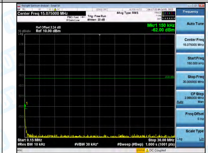
Band2_Band2_10MHz_QPSK_19150_1RB#0_0.15-30_0.15-30
