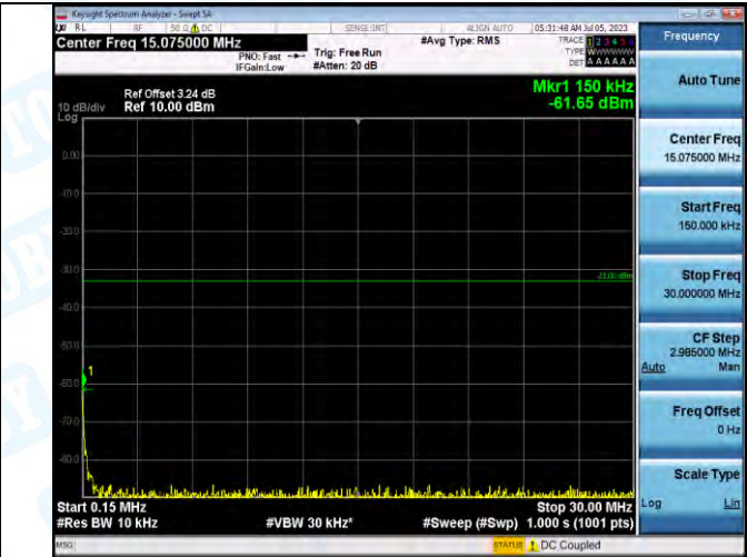
Band2_Band2_3MHz_QPSK_18615_1RB#0_0.15-30_0.15-30
