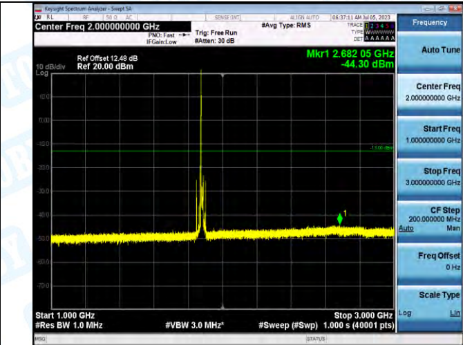
Band2_Band2_15MHz_QPSK_18900_1RB#0_1000~3000_1000~3000
