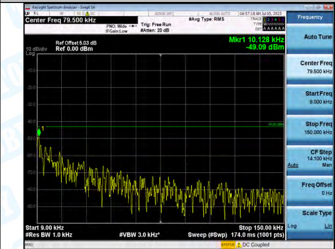
Band2_Band2_20MHz_16QAM_18700_1RB#0_0.009-0.15_0.009-0.15
