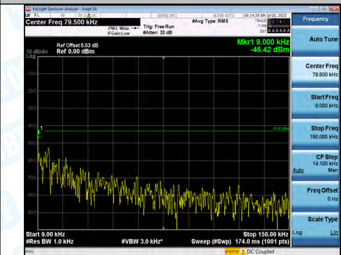
Band2_Band2_10MHz_16QAM_18650_1RB#0_0.009-0.15_0.009-0.15
