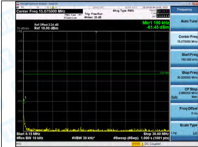
Band2_Band2_5MHz_16QAM_18625_1RB#0_0.15~30_0.15~30
