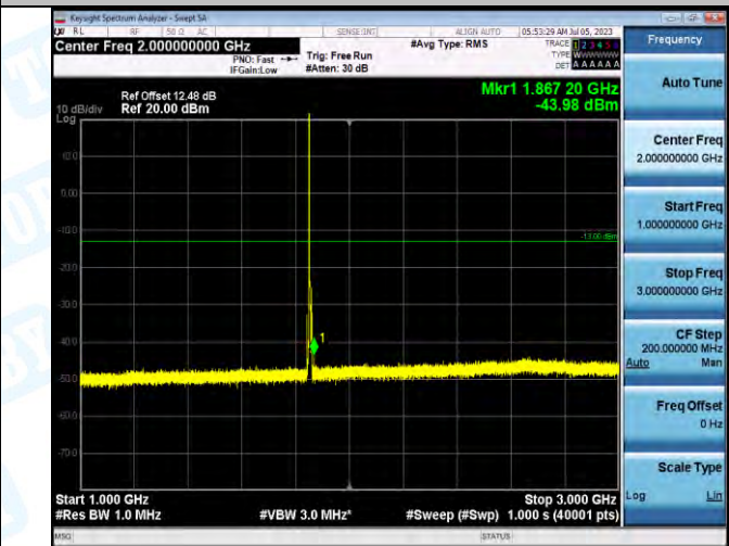
Band2_Band2_5MHz_QPSK_18625_1RB#0_1000-3000_1000-3000
