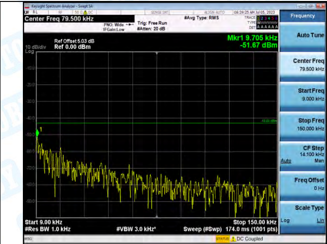
Band2_Band2_15MHz_16QAM_19125_1RB#0_0.009-0.15_0.009-0.15
