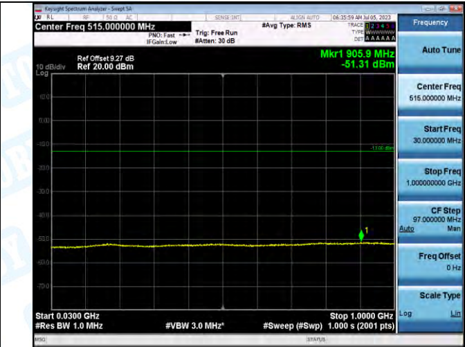
Band2_Band2_15MHz_16QAM_18675_1RB#0_30~1000_30~1000
