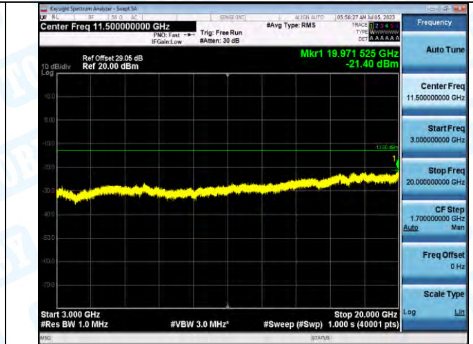
Band2_Band2_5MHz_16QAM_18900_1RB#0_3000-20000_3000-20000
