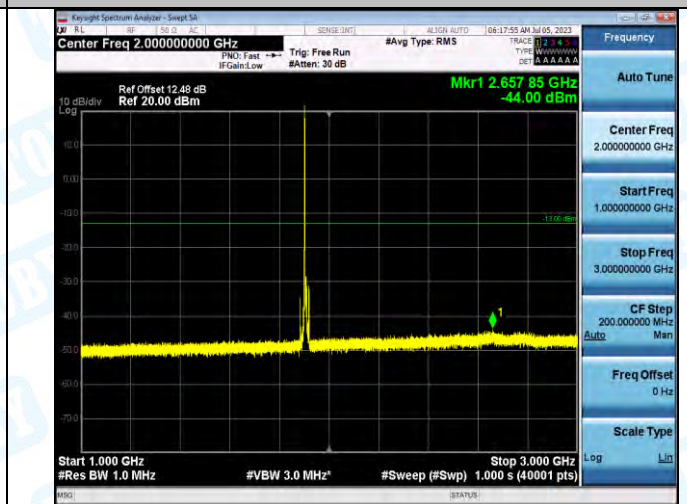
Band2_Band2_10MHz_QPSK_19150_1RB#0_1000-3000_1000-3000
