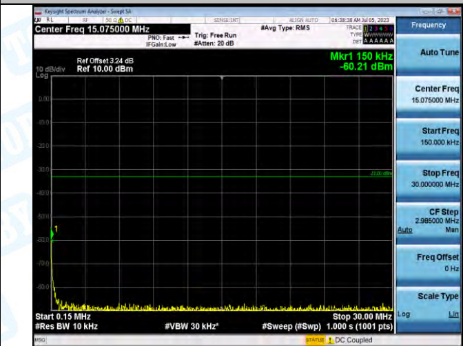
Band2_Band2_15MHz_QPSK_19125_1RB#0_0.15-30_0.15-30
