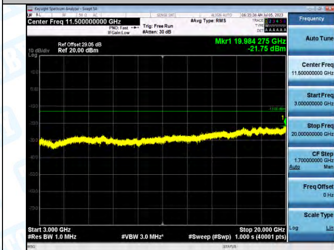
Band2_Band2_15MHz_QPSK_18675_1RB#0_3000-20000_3000-20000
