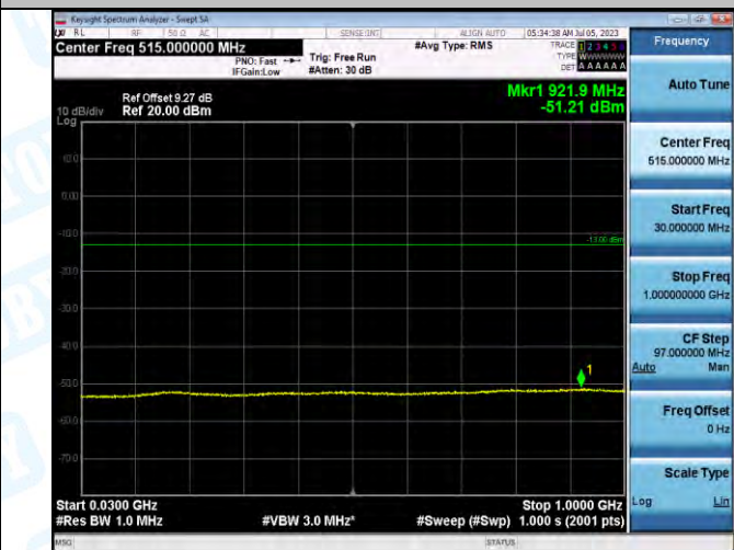
Band2_Band2_3MHz_16QAM_18900_1RB#0_30-1000_30-1000
