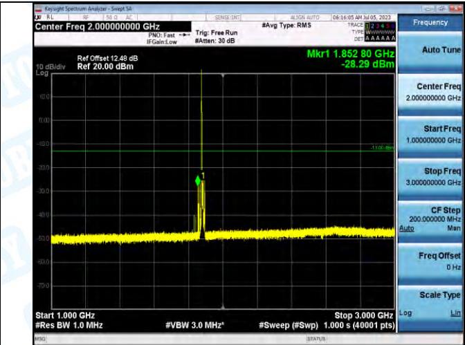
Band2_Band2_10MHz_QPSK_18900_1RB#0_1000~3000_1000~3000
