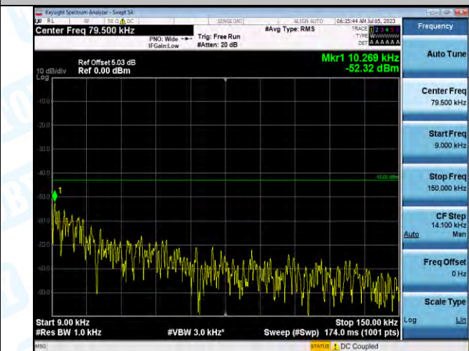
Band2_Band2_15MHz_16QAM_18675_1RB#0_0.009-0.15_0.009-0.15
