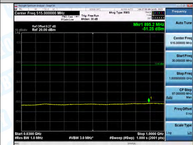
Band2_Band2_15MHz_16QAM_18900_1RB#0_30~1000_30~1000
