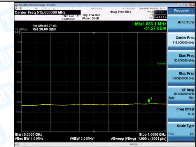
Band2_Band2_15MHz_16QAM_19125_1RB#0_30-1000_30-1000
