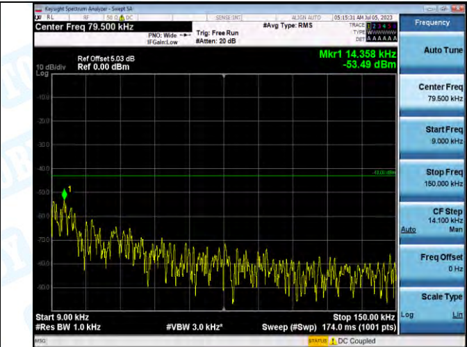
Band2_Band2_1.4MHz_16QAM_19193_1RB#0_0.009-0.15_0.009-0.15
