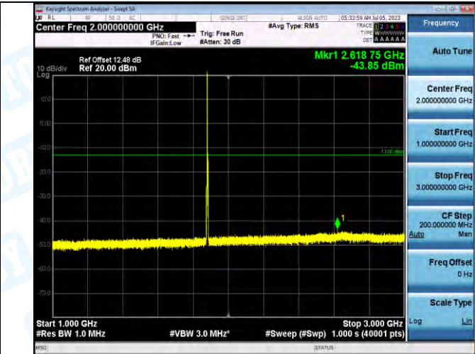
Band2_Band2_3MHz_QPSK_18900_1RB#0_1000-3000_1000-3000
