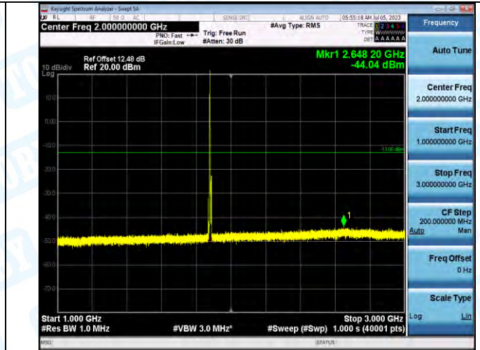
Band2_Band2_5MHz_QPSK_18900_1RB#0_1000-3000_1000-3000
