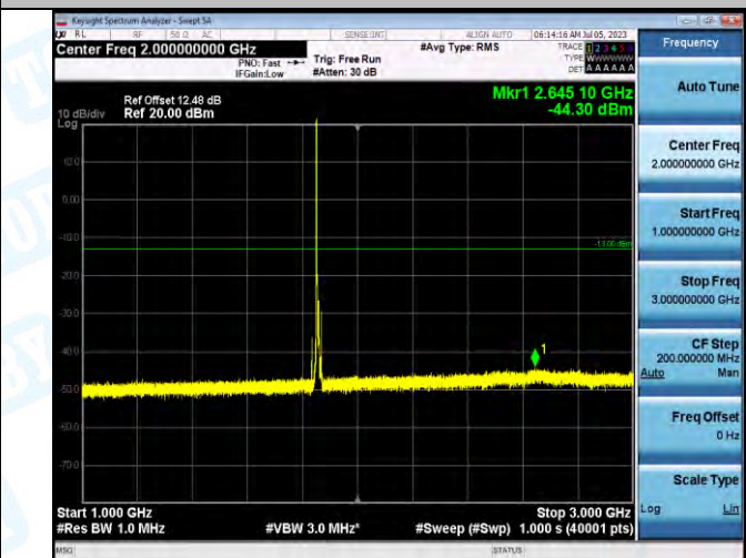
Band2_Band2_10MHz_QPSK_18650_1RB#0_1000-3000_1000-3000
