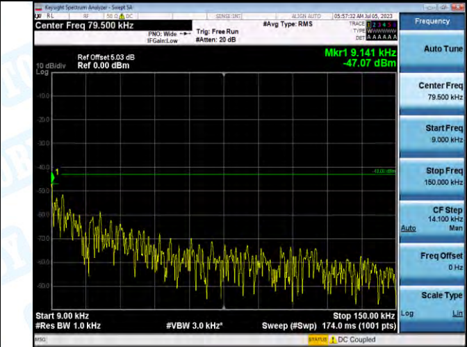
Band2_Band2_5MHz_16QAM_19175_1RB#0_0.009-0.15_0.009-0.15
