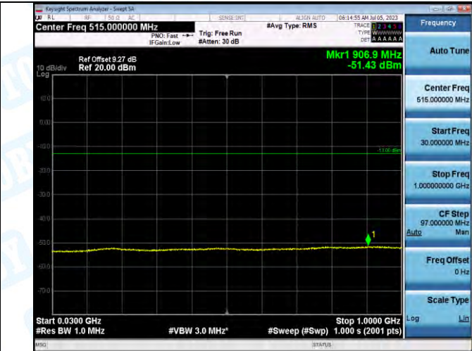
Band2_Band2_10MHz_16QAM_18650_1RB#0_30~1000_30~1000
