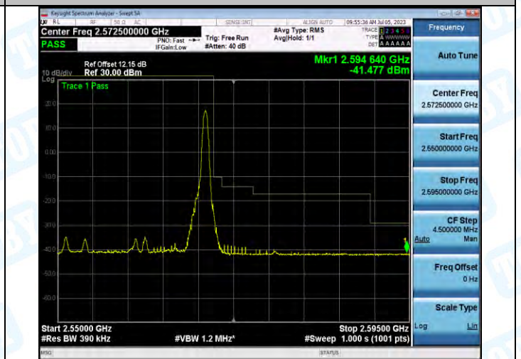
Band7_Band7_20MHz_16QAM_21350_1RB#99
