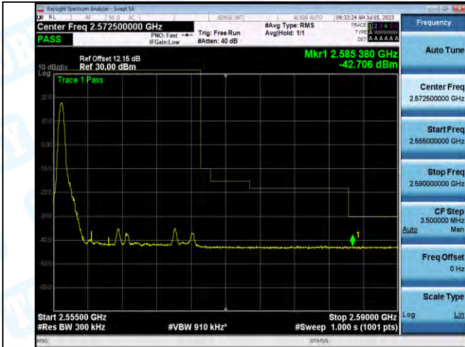
Band7_Band7_15MHz_QPSK_21375_1RB#0
