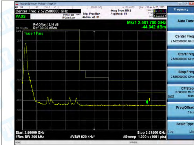
Band7_Band7_10MHz_QPSK_21400_1RB#0
