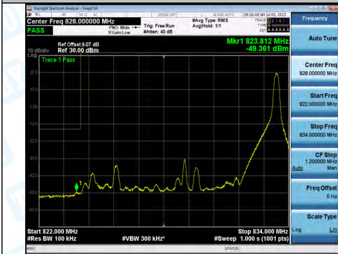
Band5_Band5_10MHz_QPSK_20450_1RB#49
