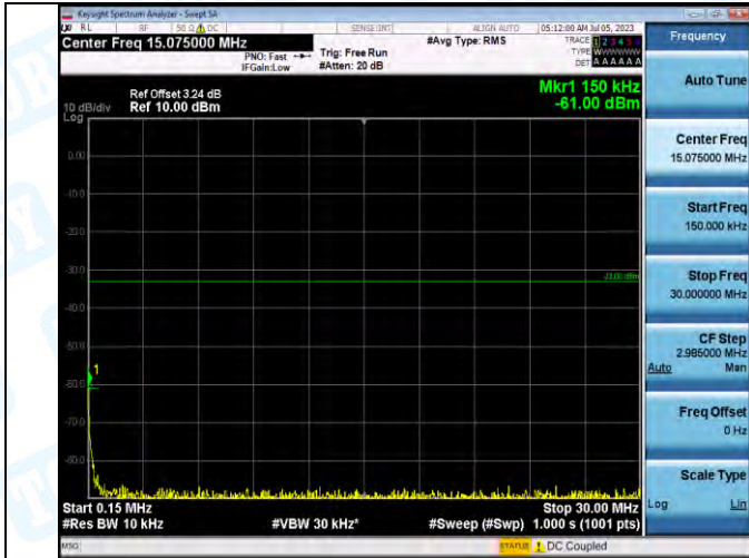
Band2_Band2_1.4MHz_16QAM_18607_1RB#0_0.15-30_0.15-30
