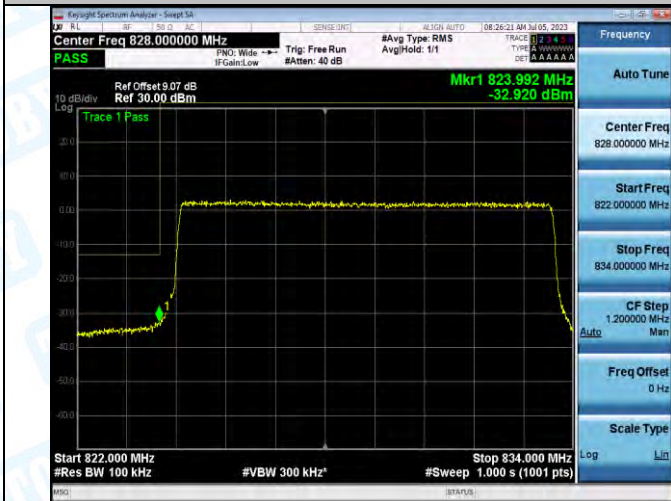
Band5_Band5_10MHz_QPSK_20450_50RB#0
