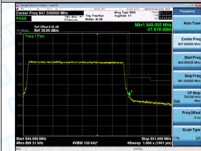
Band5_Band5_5MHz_QPSK_20625_25RB#0
