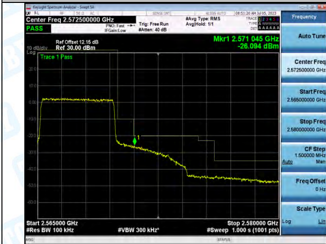
Band7_Band7_5MHz_QPSK_21425_25RB#0
