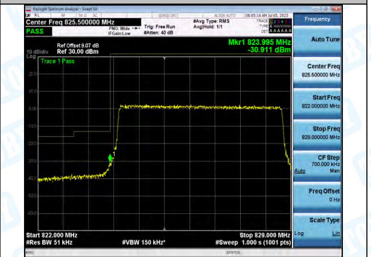
Band5_Band5_5MHz_16QAM_20425_25RB#0
