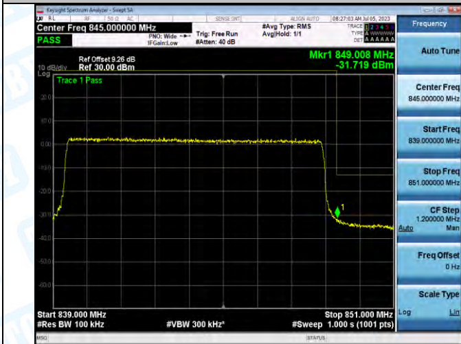
Band5_Band5_10MHz_QPSK_20600_50RB#0
