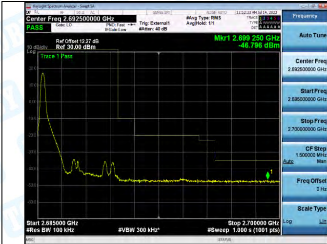
Band41_Band41_5MHz_QPSK_41565_1RB#0
