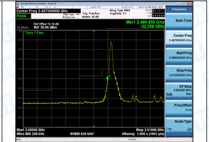
Band7_Band7_10MHz_16QAM_20800_1RB#0
