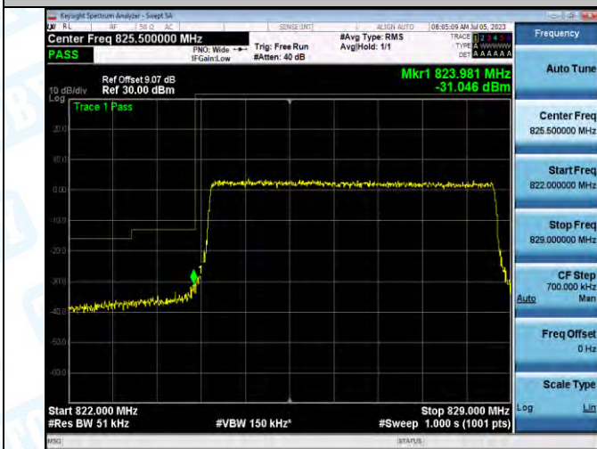
Band5_Band5_5MHz_QPSK_20425_25RB#0
