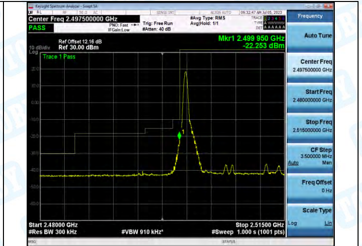
Band7_Band7_15MHz_16QAM_20825_1RB#0
