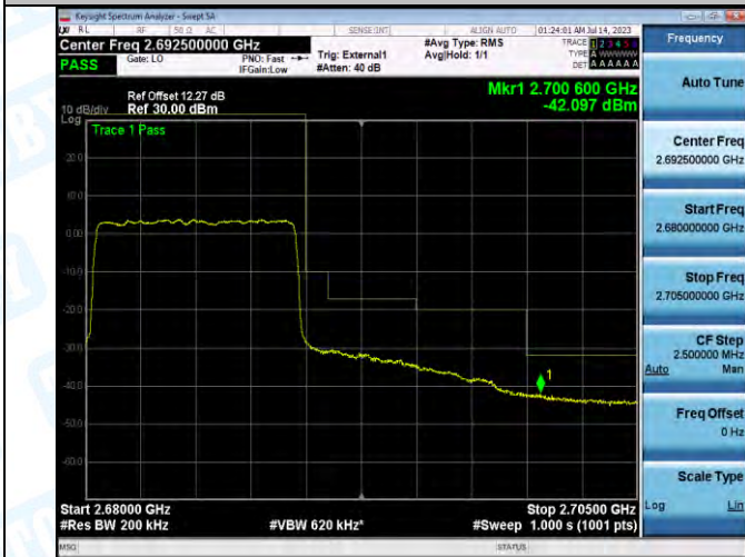
Band41_Band41_10MHz_QPSK_41540_50RB#0
