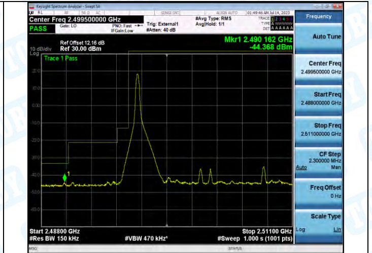
Band41_Band41_15MHz_16QAM_39725_1RB#0
