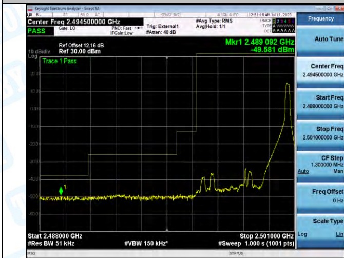
Band41_Band41_5MHz_QPSK_39675_2RB#24
