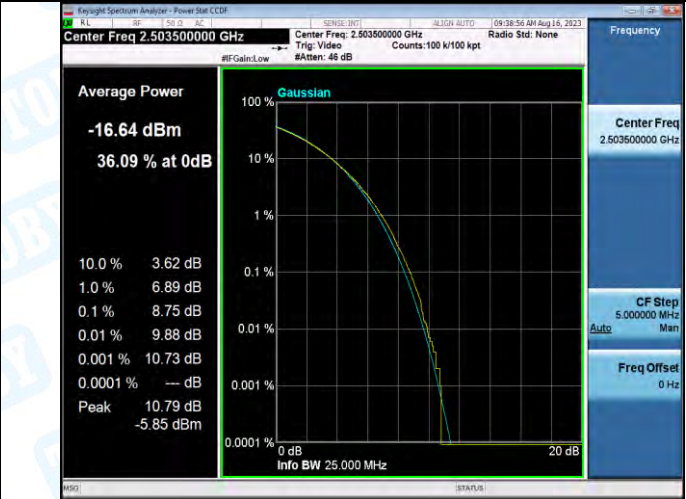
Band41-15MHz-16QAM-39725-1RB#0-PASS
