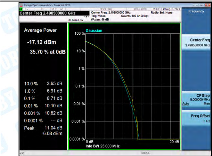
Band41-5MHz-16QAM-39675-25RB#0-PASS
