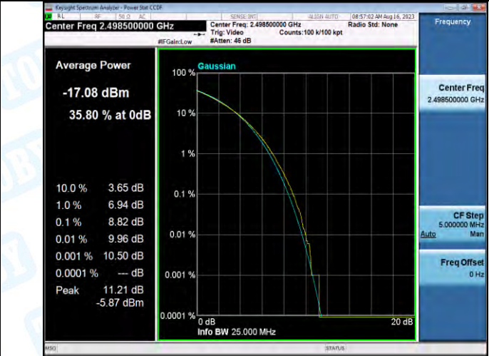
Band41-5MHz-16QAM-39675-1RB#0-PASS
