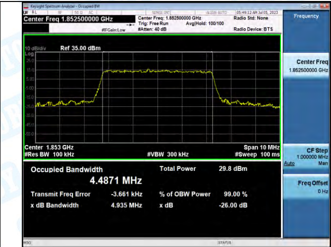
Band2-5MHz-16QAM-18625-25RB#0-PASS
