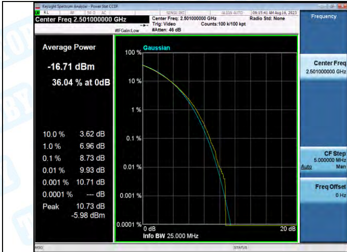
Band41-10MHz-QPSK-39700-1RB#0-PASS
