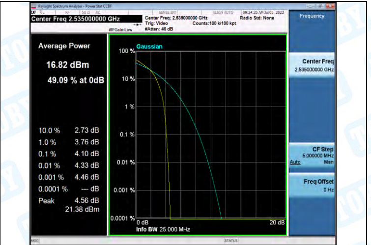
Band7-10MHz-16QAM-21100-50RB#0-PASS
