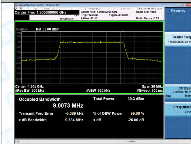
Band2-10MHz-QPSK-19150-50RB#0-PASS
