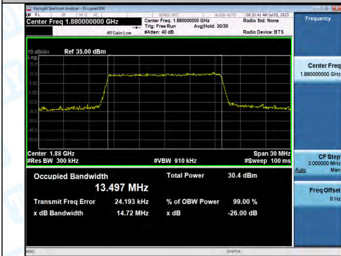
Band2-15MHz-QPSK-18900-75RB#0-PASS
