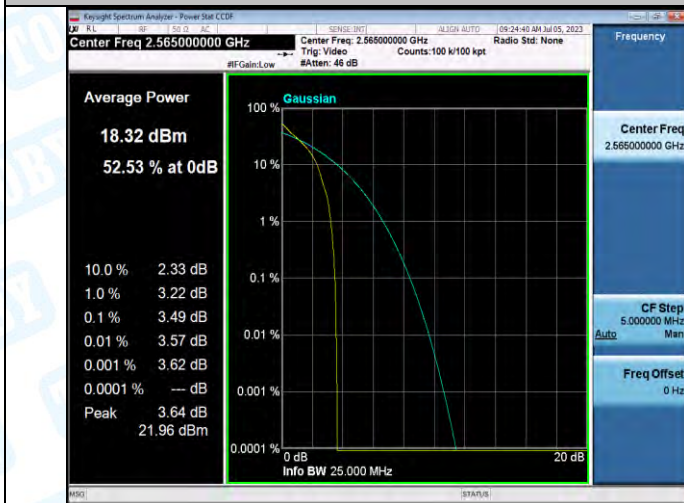
Band7-10MHz-QPSK-21400-1RB#0-PASS
