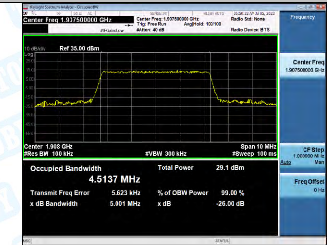
Band2-5MHz-16QAM-19175-25RB#0-PASS
