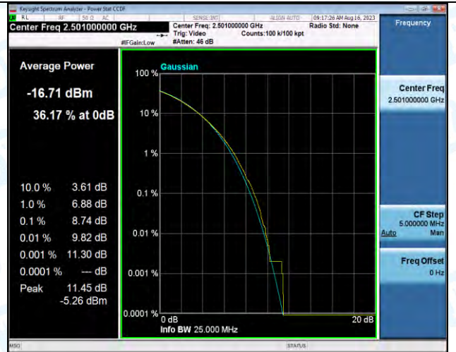
Band41-10MHz-16QAM-39700-1RB#0-PASS
