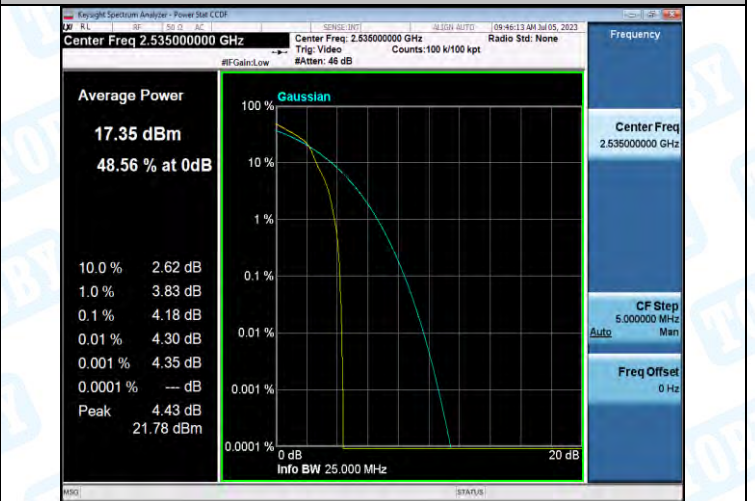
Band7-15MHz-16QAM-21100-1RB#0-PASS
