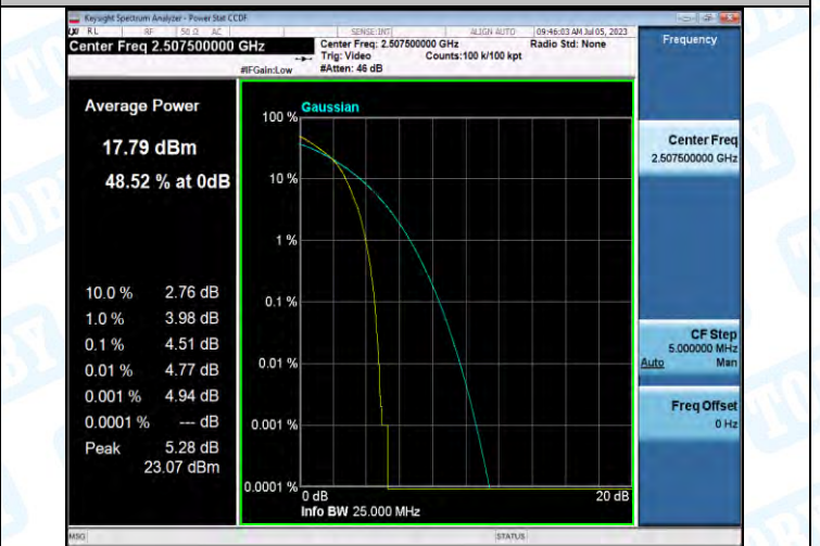
Band7-15MHz-16QAM-20825-75RB#0-PASS
