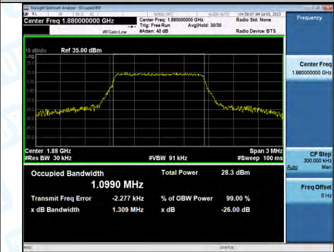
Band2-1.4MHz-16QAM-18900-6RB#0-PASS
