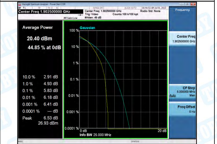
Band2-15MHz-16QAM-19125-75RB#0-PASS
