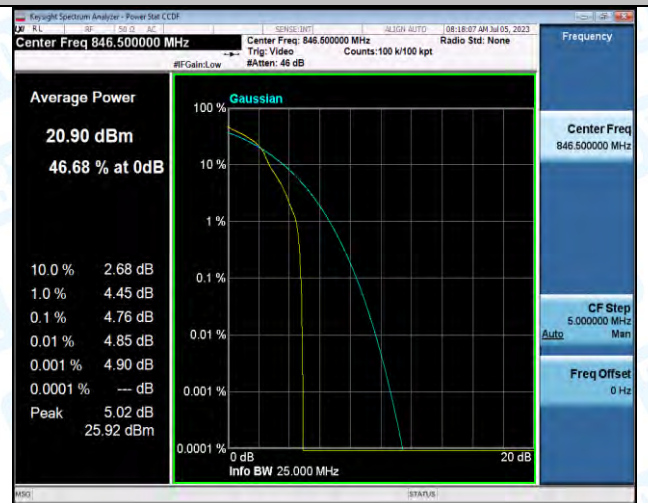
Band5-5MHz-16QAM-20625-1RB#0-PASS
