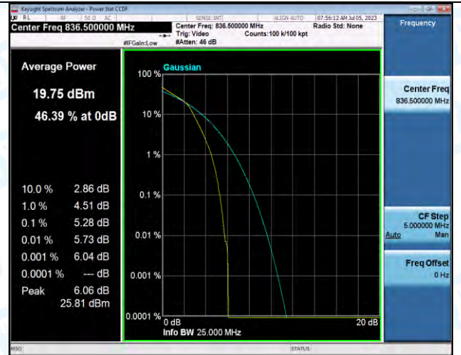
Band5-3MHz-16QAM-20525-15RB#0-PASS
