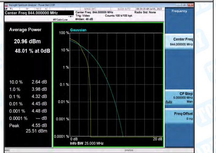
Band5-10MHz-16QAM-20600-1RB#0-PASS
