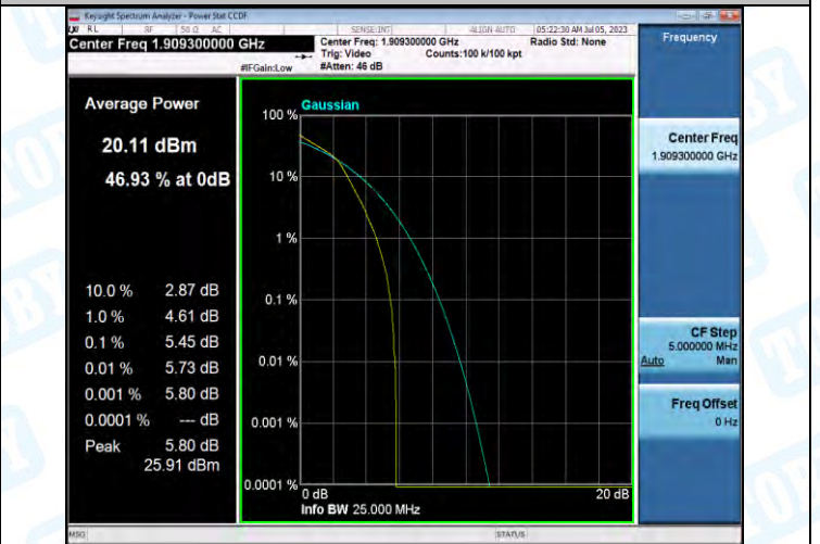
Band2-1.4MHz-16QAM-19193-6RB#0-PASS
