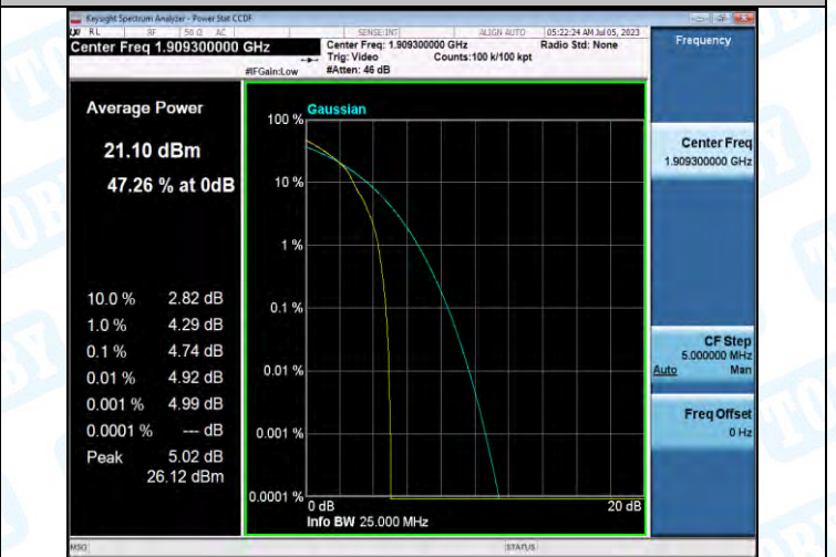
Band2-1.4MHz-16QAM-19193-1RB#0-PASS
