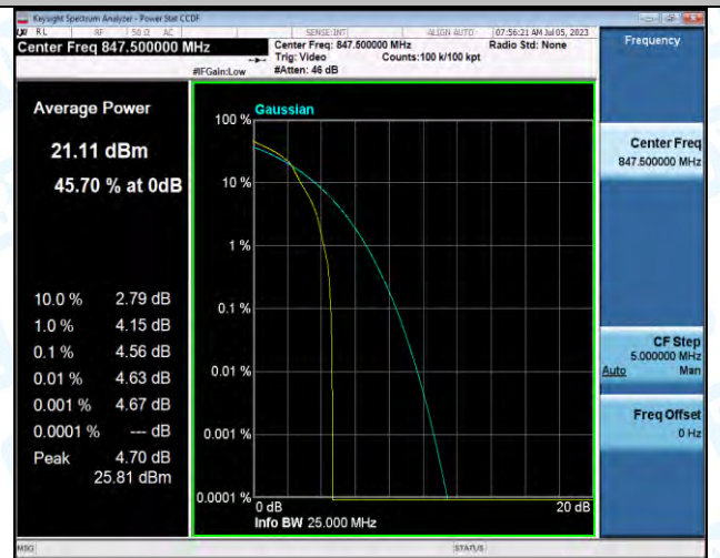
Band5-3MHz-16QAM-20635-1RB#0-PASS
