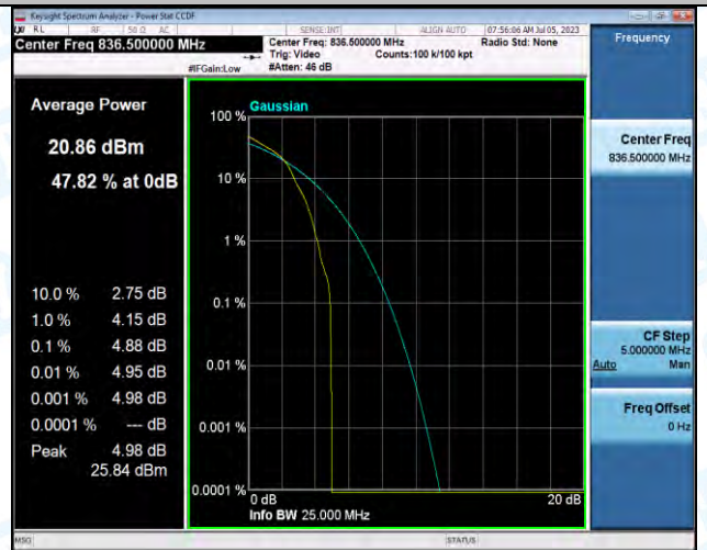
Band5-3MHz-16QAM-20525-1RB#0-PASS
