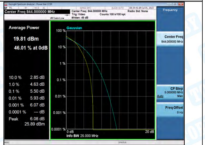
Band5-10MHz-16QAM-20600-50RB#0-PASS
