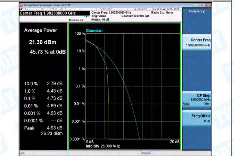
Band2-15MHz-16QAM-19125-1RB#0-PASS
