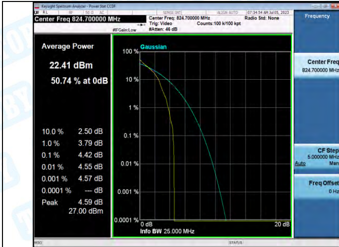
Band5-1.4MHz-QPSK-20407-1RB#0-PASS
