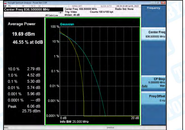
Band5-10MHz-16QAM-20525-50RB#0-PASS
