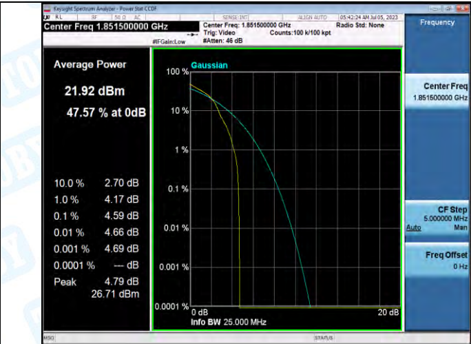
Band2-3MHz-16QAM-18615-1RB#0-PASS
