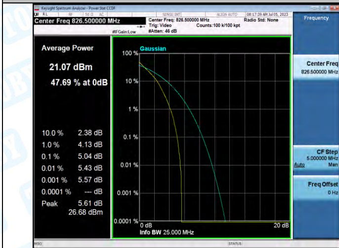
Band5-5MHz-QPSK-20425-25RB#0-PASS
