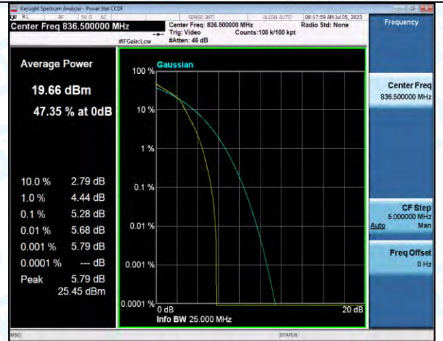
Band5-5MHz-16QAM-20525-25RB#0-PASS
