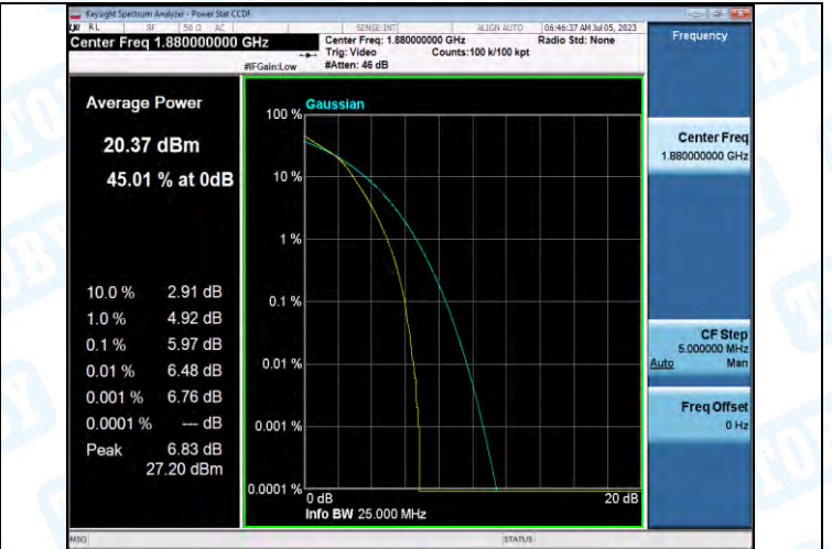
Band2-15MHz-16QAM-18900-75RB#0-PASS
