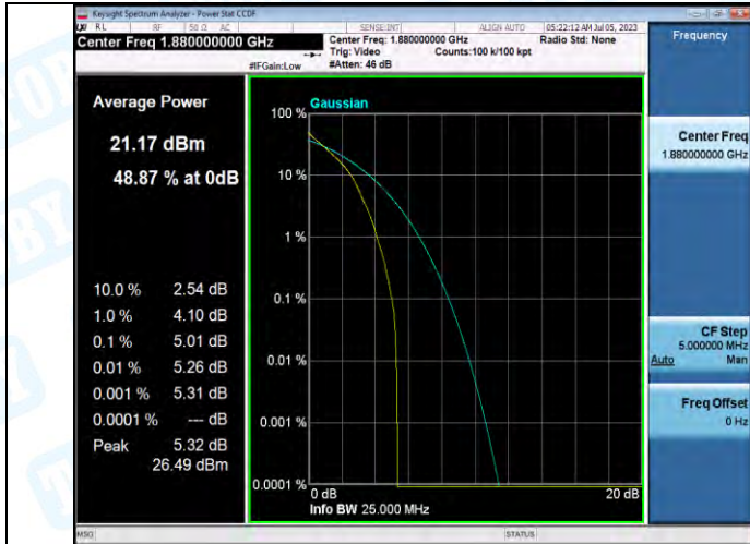
Band2-1.4MHz-QPSK-18900-6RB#0-PASS
