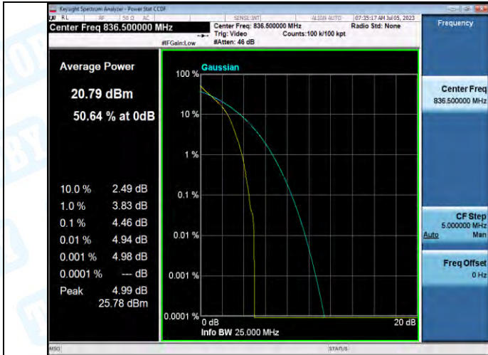
Band5-1.4MHz-QPSK-20525-6RB#0-PASS
