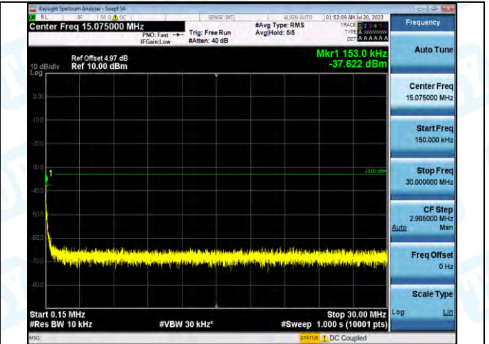
EGPRS1900-512-2-0.15~30MHz-PASS
