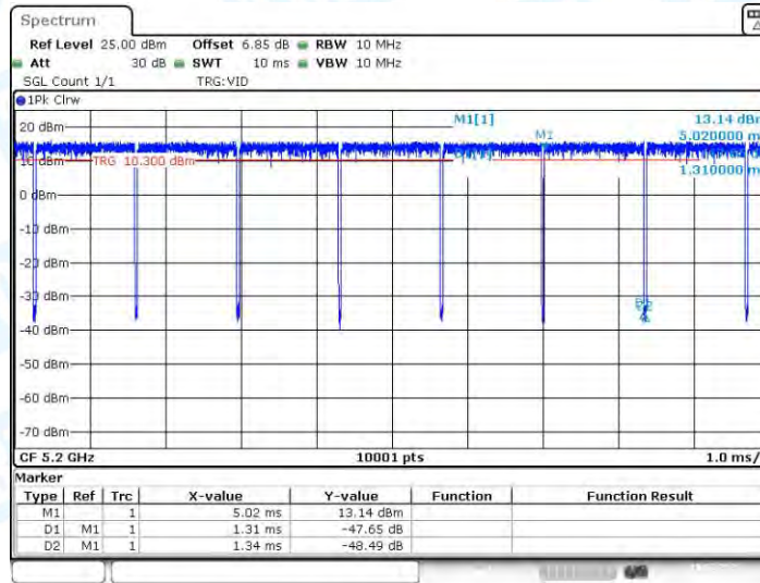
11AC20SISO_Ant1_5200
