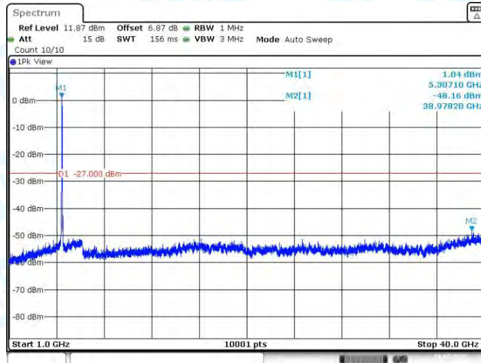
11N40SISO_Ant1_5310_1000~40000
