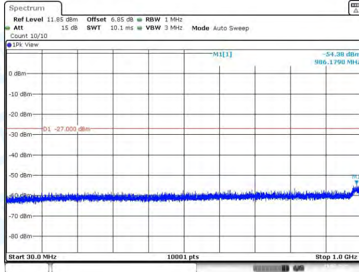
11AC40SISO_Ant1_5190_30~1000
