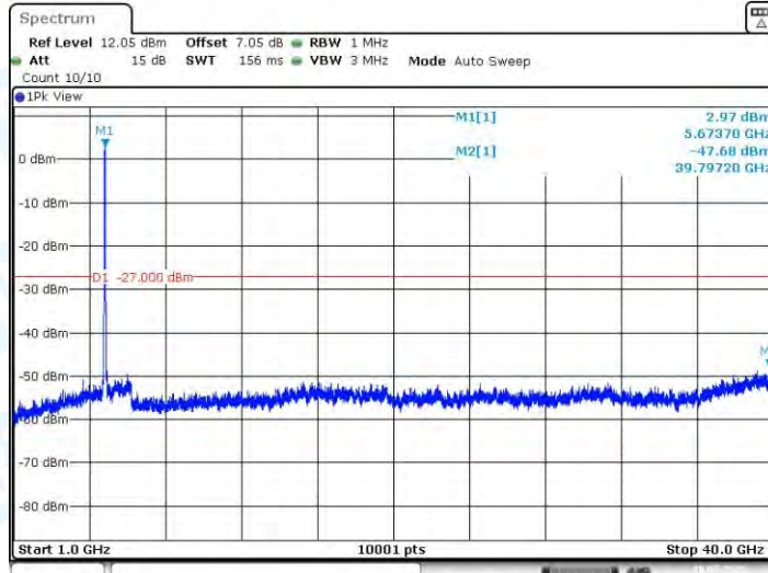
11N40SISO_Ant1_5670_1000~40000
