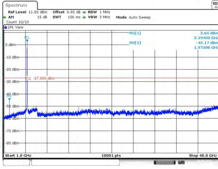
11N40SISO_Ant1_5190_1000~40000
