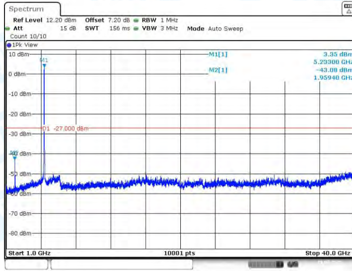
11N40SISO_Ant1_5230_1000~40000
