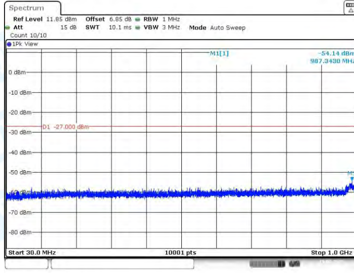
11N40SISO_Ant1_5190_30~1000
