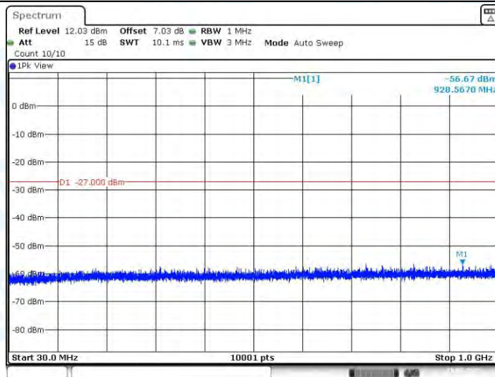
11N40SISO_Ant1_5550_30~1000
