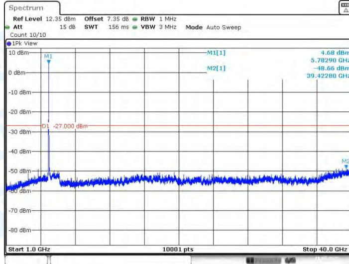
11AC20SISO_Ant1_5785_1000~40000
