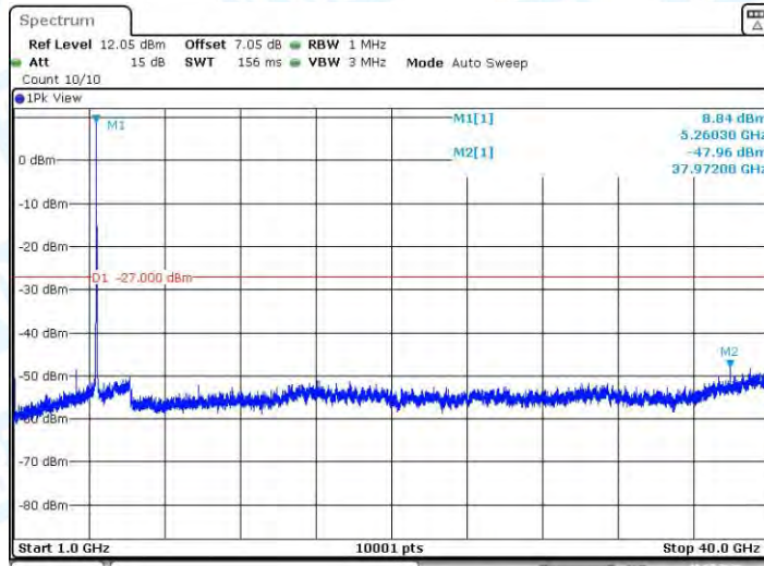
11AC20SISO_Ant1_5260_1000~40000
