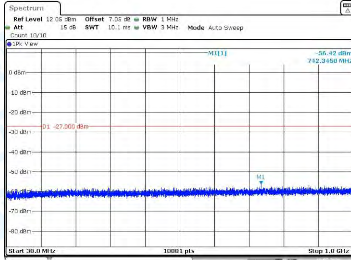
11N40SISO_Ant1_5670_30~1000
