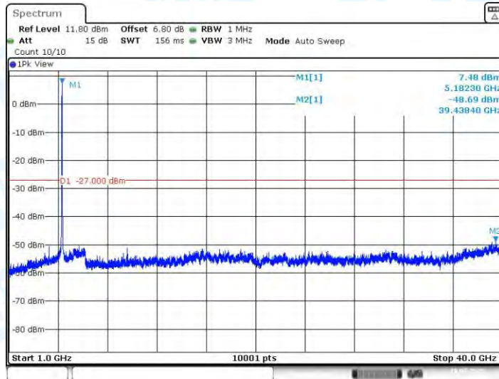
11AC20SISO_Ant1_5180_1000~40000
