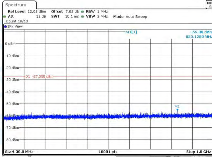
11AC20SISO_Ant1_5260_30~1000
