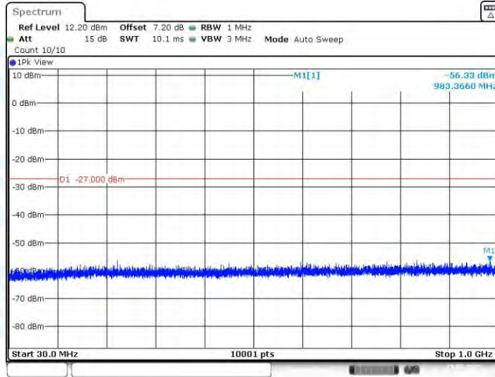
11AC20SISO_Ant1_5240_30~1000
