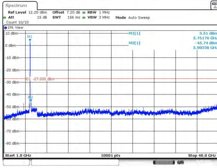
11N40SISO_Ant1_5755_1000~40000
