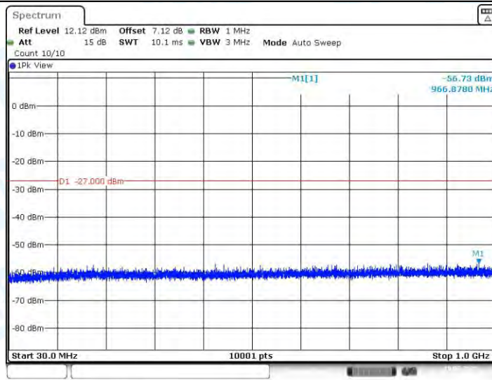
11N40SISO_Ant1_5270_30~1000
