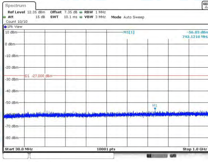
11N40SISO_Ant1_5795_30~1000
