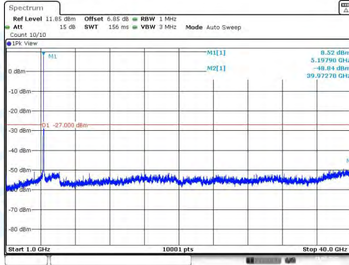
11AC20SISO_Ant1_5200_1000~40000
