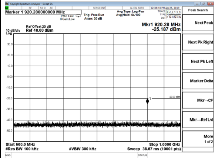
600 MHz – 1000 MHz
