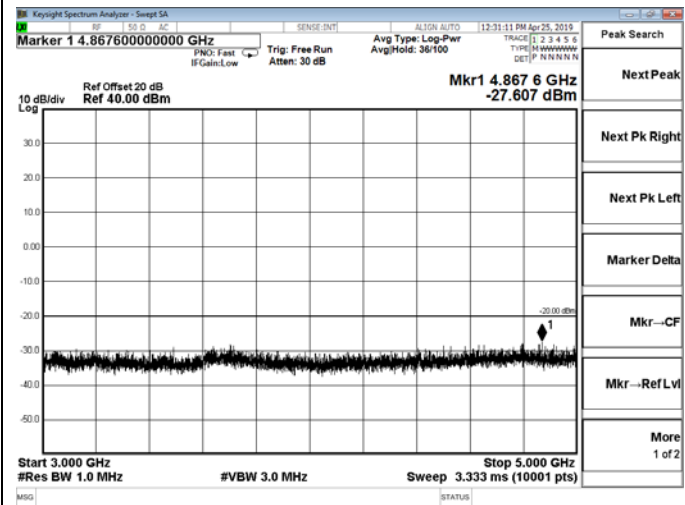
3 GHz – 5 GHz
