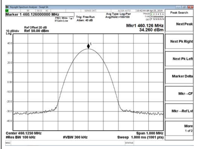
Channel 1 / 460.125 MHz
