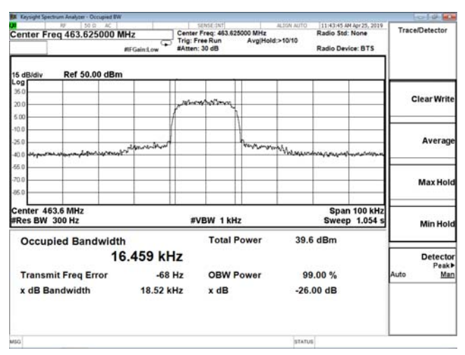
Channel 8 / 463.625 MHz
