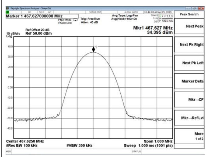
Channel 16 / 467.625 MHz
