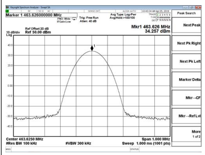
Channel 8 / 463.625 MHz
