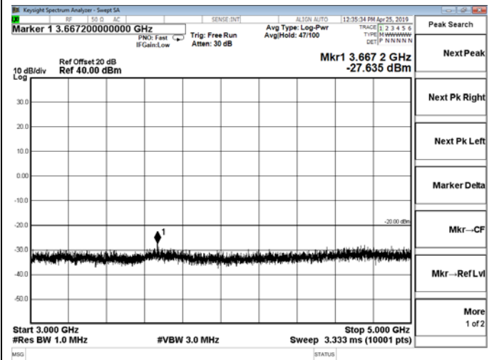
3 GHz – 5 GHz
