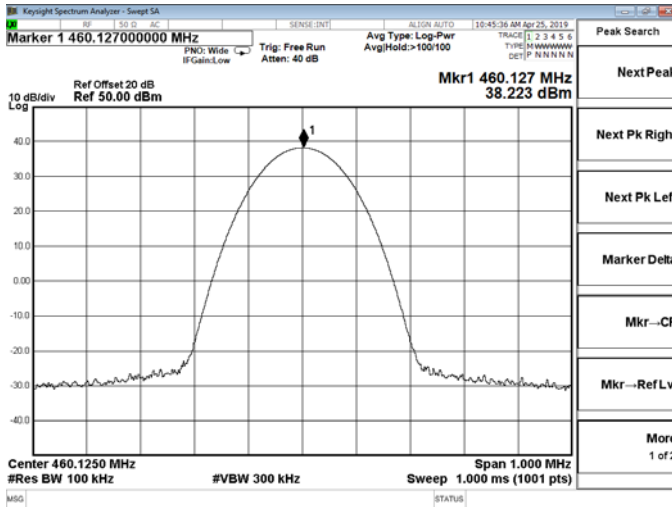
Channel 1 / 460.125 MHz
