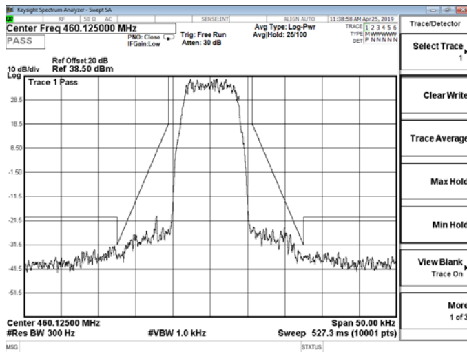
Channel 1 / 460.125 MHz
