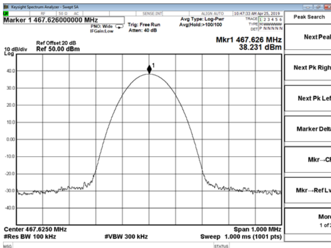
Channel 16 / 467.625 MHz
