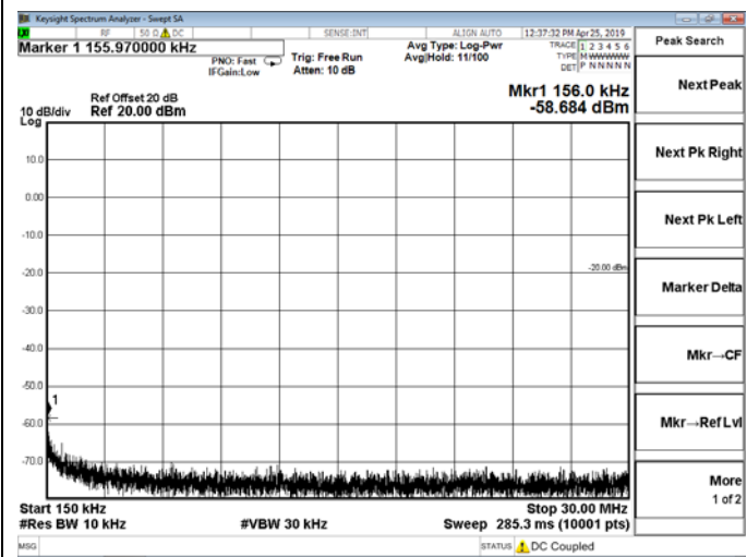
150 KHz – 30 MHz
