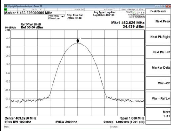
Channel 8 / 463.625 MHz
