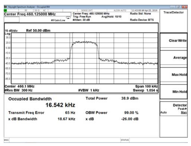
Channel 1 / 460.125 MHz
