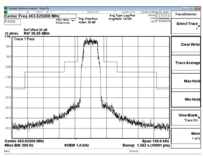
Channel 8 / 463.625 MHz
