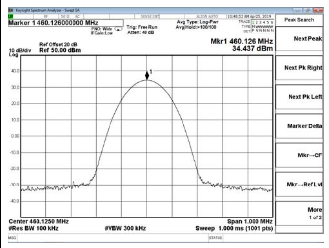
Channel 1 / 460.125 MHz
