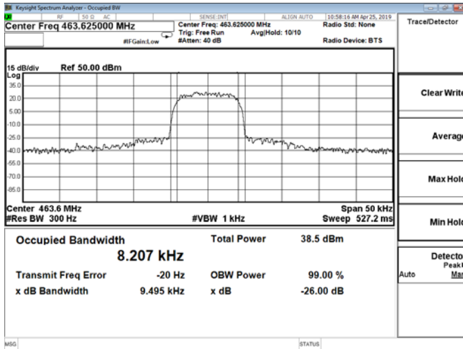
Channel 8 / 463.625 MHz
