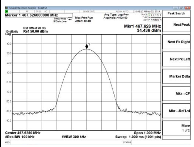
Channel 16 / 467.625 MHz
