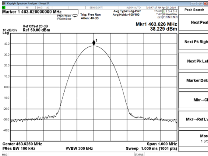
Channel 8 / 463.625 MHz
