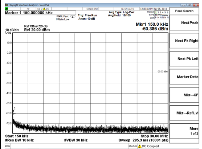
150 KHz – 30 MHz
