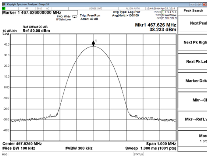
Channel 16 / 467.625 MHz
