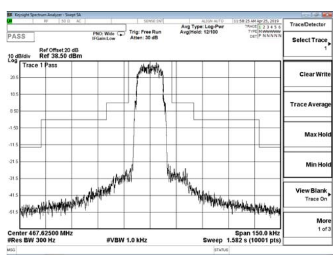
Channel 16 / 467.625 MHz
