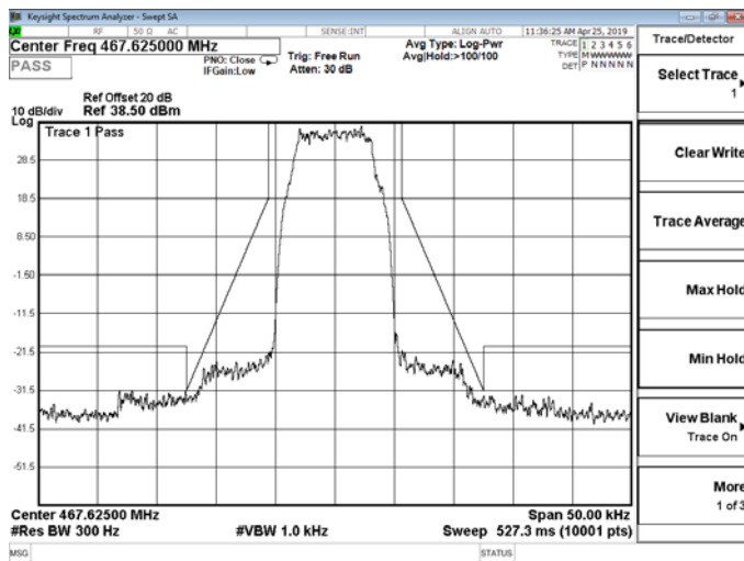
Channel 16 / 467.625 MHz
