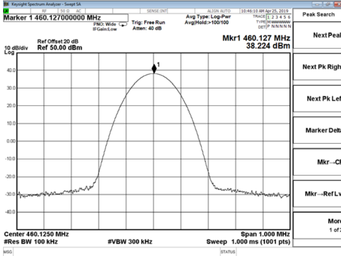
Channel 1 / 460.125 MHz
