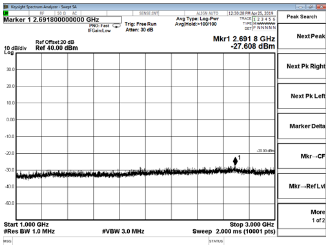
1 GHz – 3 GHz
