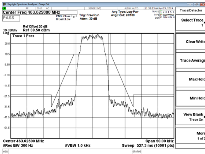
Channel 8 / 463.625 MHz
