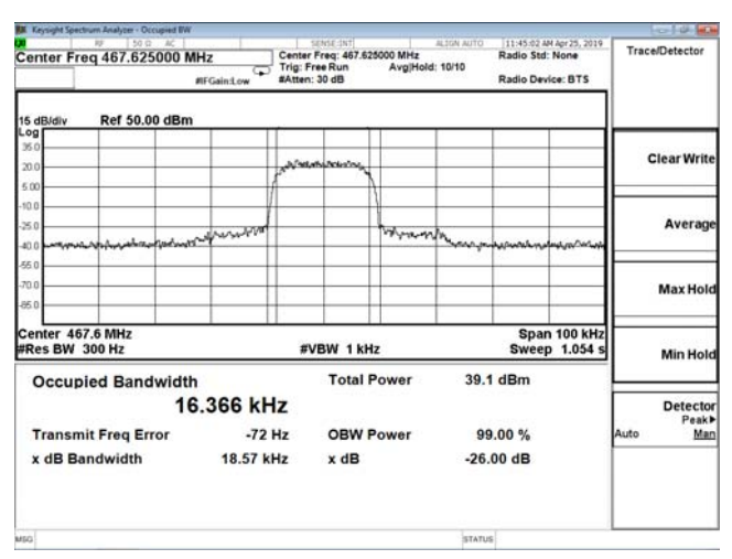
Channel 16 / 467.625 MHz
