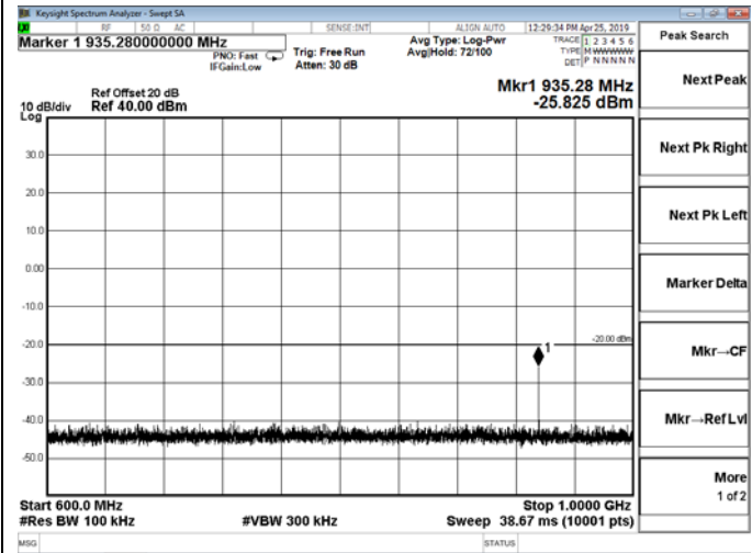
600 MHz – 1000 MHz
