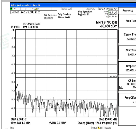
Band7_5MHz_QPSK_21425_1RB#0_0.009~0.15_0.009~0.15
