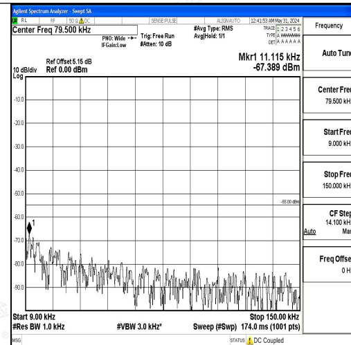
Band7_5MHz_16QAM_20775_1RB#0_0.009~0.15 _0.009~0.15
