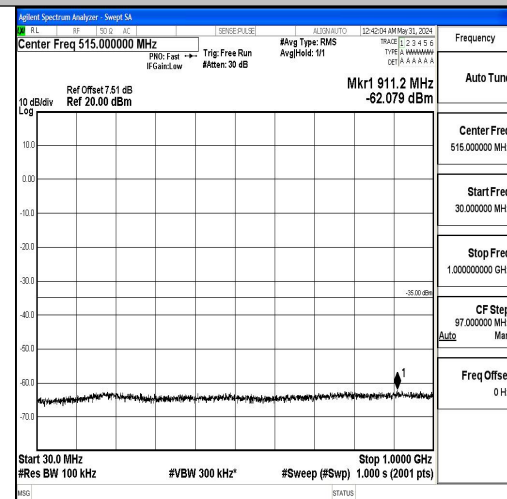
Band7_5MHz_16QAM_20775_1RB#0_30~1000_3 0~1000
