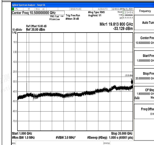
Band7_5MHz_16QAM_21100_1RB#0_1000~2000_1000~20000
