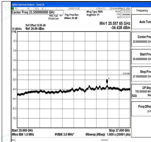
Band7_5MHz_QPSK_20775_1RB#0_20000~27000 00_20000~27000
