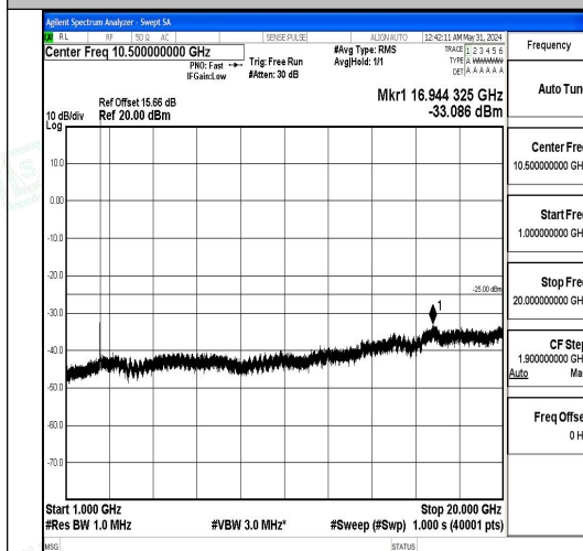
Band7_5MHz_16QAM_20775_1RB#0_1000~200 00_1000~20000
