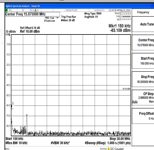
Band7_5MHz_QPSK_21425_1RB#0_0.15~30_0.15~30
