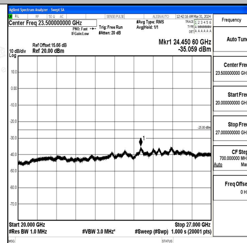
Band7_5MHz_16QAM_20775_1RB#0_20000~270 00_20000~27000
