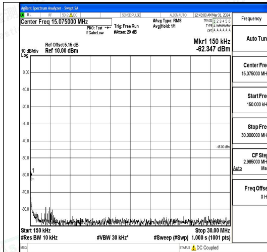
Band7_5MHz_16QAM_21100_1RB#0_0.15~30_0.15~30
