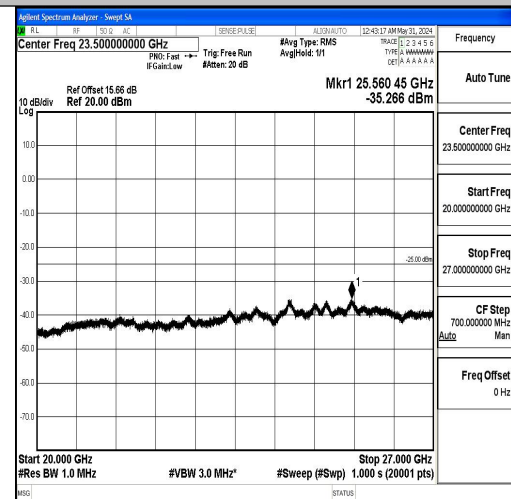
Band7_5MHz_16QAM_21100_1RB#0_20000~27000_20000~27000
