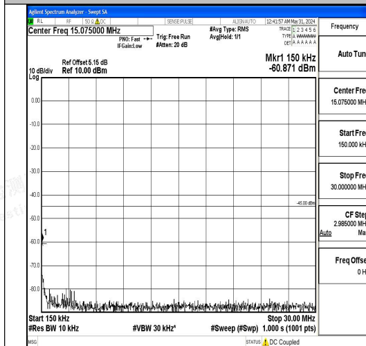
Band7_5MHz_16QAM_20775_1RB#0_0.15~30 0.15~30
