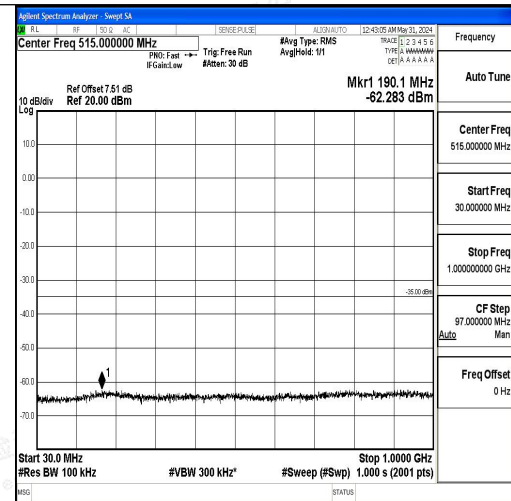
Band7_5MHz_16QAM_21100_1RB#0_30~1000_30~1000
