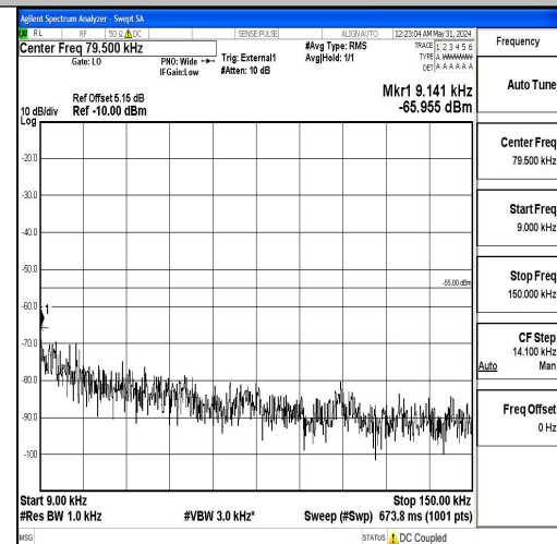
Band41_20MHz_16QAM_41490_1RB#0_0.009~0.15_0.009~0.15
