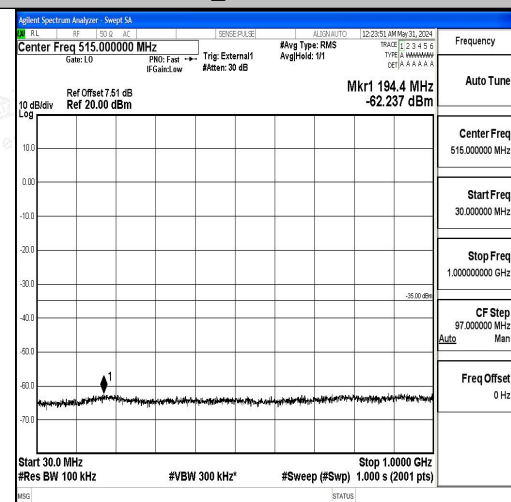
Band41_20MHz_16QAM_41490_1RB#0_30~1000_30~1000
