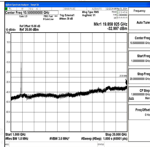
Band41_20MHz_QPSK_41490_1RB#0_1000~20000_1000~20000
