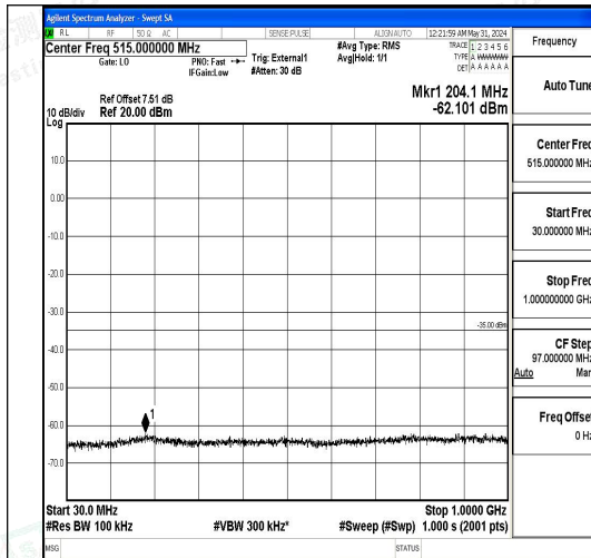
Band41_20MHz_QPSK_41490_1RB#0_30~1000_30~1000
