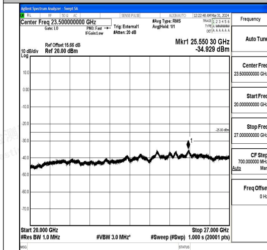
Band41_20MHz_QPSK_41490_1RB#0_20000~27000_20000~27000
