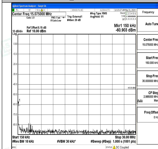
Band41_20MHz_16QAM_41490_1RB#0_0.15~30_0.15~30
