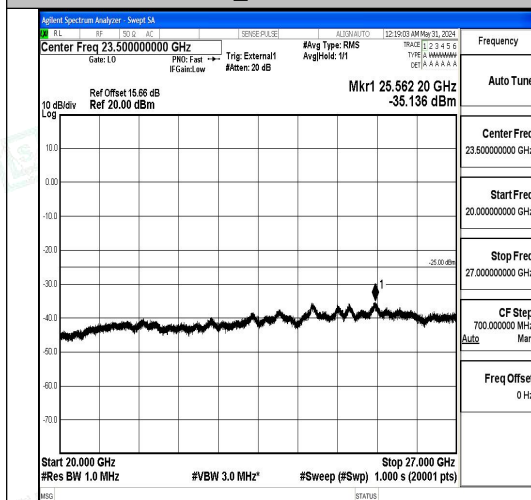
Band41_20MHz_QPSK_40620_1RB#0_20000~27000_20000~27000
