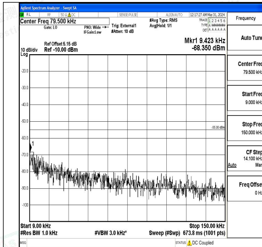
Band41_20MHz_QPSK_40620_1RB#0_0.009~0.15_0.009~0.15
