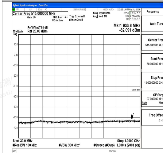
Band41_20MHz_QPSK_40620_1RB#0_30~1000_30~1000
