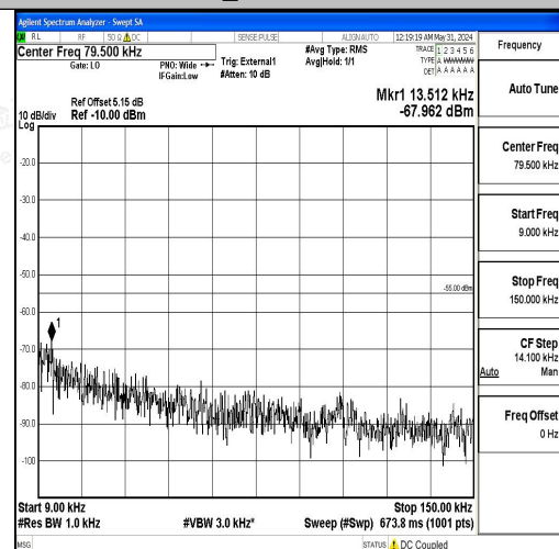
Band41_20MHz_16QAM_40620_1RB#0_0.009~0.15_0.009~0.15
