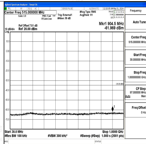
Band41_20MHz_16QAM_40620_1RB#0_30~1000 _30~1000
