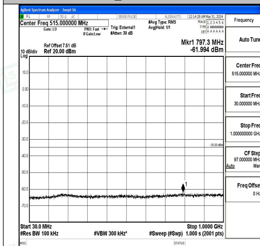
Band41_20MHz_QPSK_39750_1RB#0_30~1000
