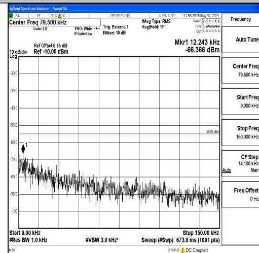
Band41_15MHz_16QAM_41515_1RB#0_0.009~0.15_0.009~0.15
