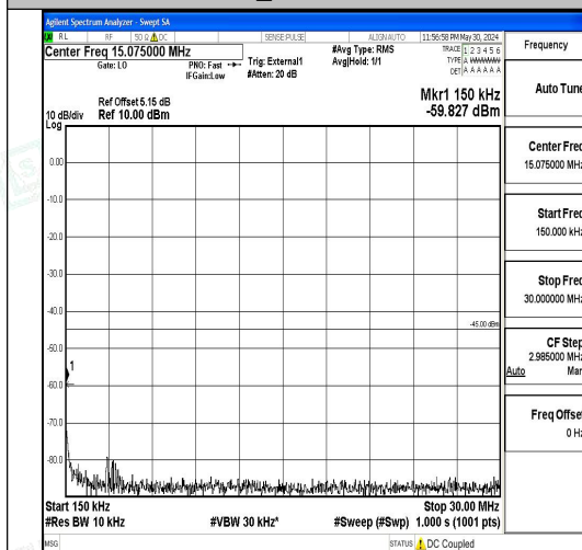
Band41_15MHz_16QAM_41515_1RB#0_0.15~30_0.15~30
