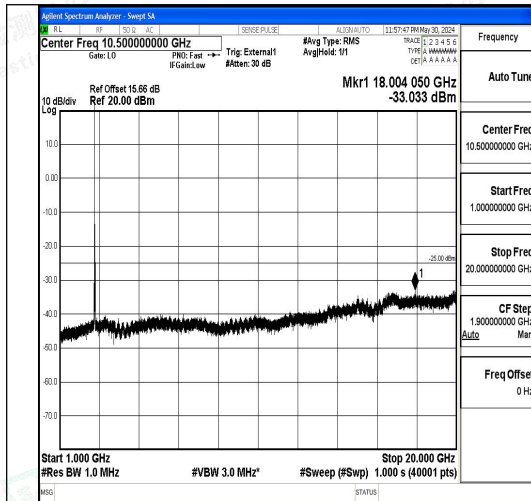
Band41_15MHz_16QAM_41515_1RB#0_1000~20000
