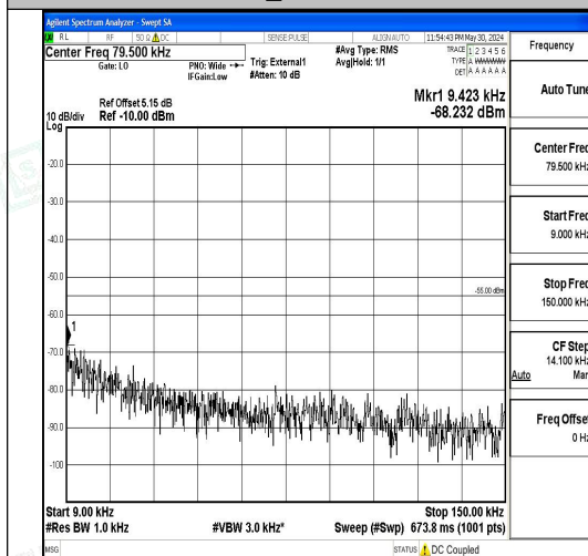
Band41_15MHz_QPSK_41515_1RB#0_0.009~0. 15_0.009~0.15
