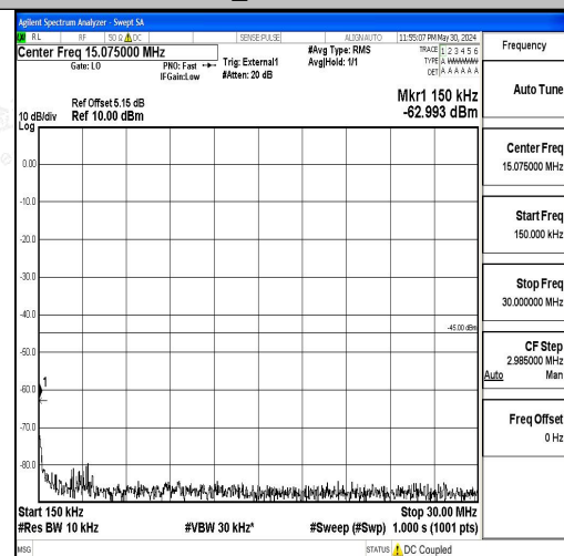
Band41_15MHz_QPSK_41515_1RB#0_0.15~30 0.15~30
