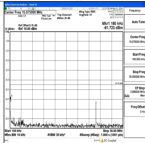
Band41_20MHz_QPSK_40620_1RB#0_0.15~30_0.15~30
