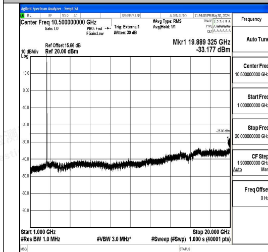
Band41_15MHz_16QAM_40620_1RB#0_1000~2 0000_1000~20000
