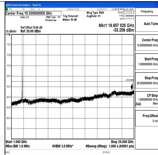
Band41_15MHz_QPSK_41515_1RB#0_1000~20000_1000~20000
