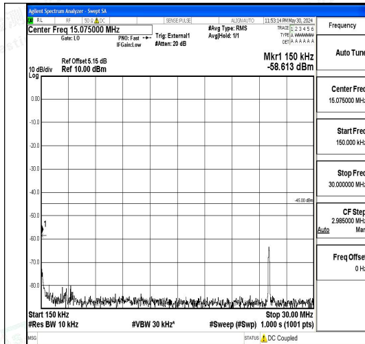
Band41_15MHz_16QAM_40620_1RB#0_0.15~3 0_0.15~30
