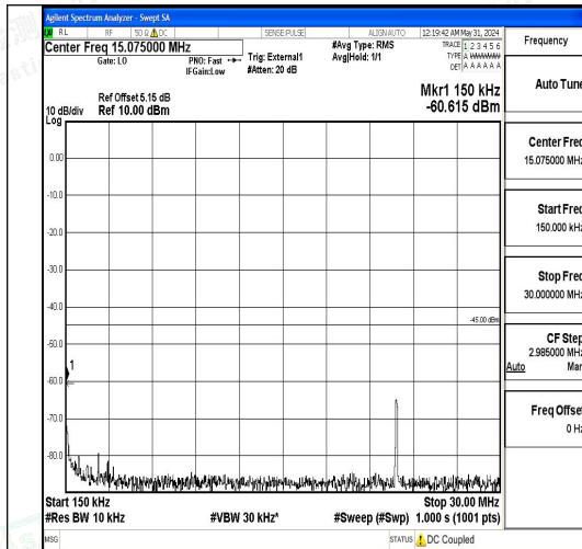
Band41_20MHz_16QAM_40620_1RB#0_0.15~30 0_0.15~30
