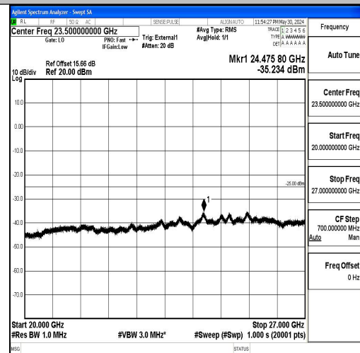
Band41_15MHz_16QAM_40620_1RB#0_20000~2 7000_20000~27000
