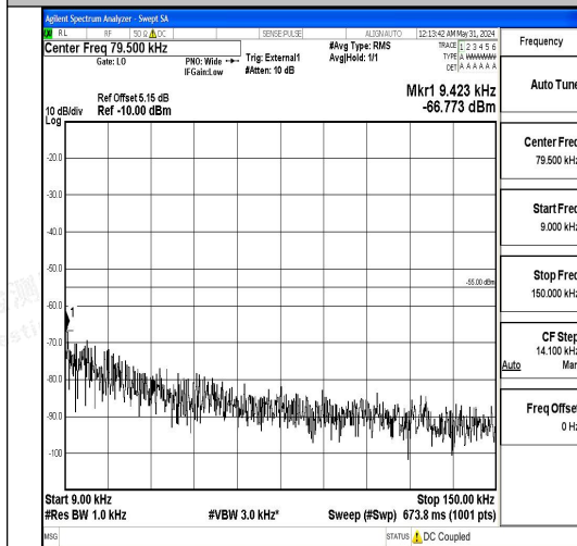
Band41_20MHz_QPSK_39750_1RB#0_0.009~0.15
