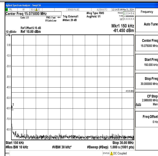
Band41_20MHz_QPSK_39750_1RB#0_0.15~30
