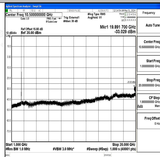
Band41_20MHz_QPSK_39750_1RB#0_1000~20000
