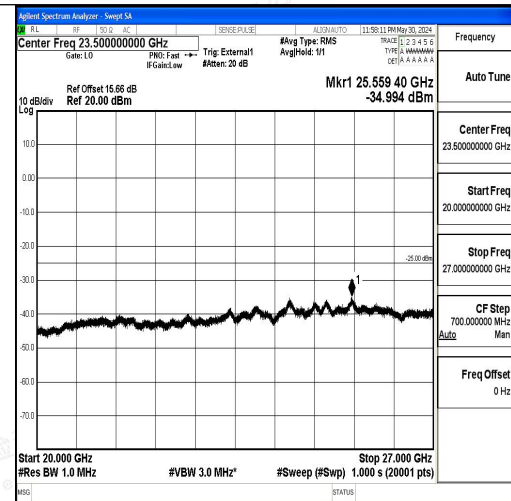
Band41_15MHz_16QAM_41515_1RB#0_20000~27000
