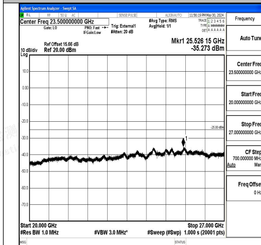
Band41_15MHz_QPSK_41515_1RB#0_20000~27000_20000~27000
