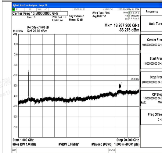
Band41_20MHz_16QAM_40620_1RB#0_1000~2 0000_1000~20000
