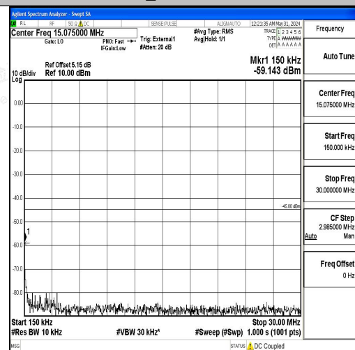
Band41_20MHz_QPSK_41490_1RB#0_0.15~30 0.15~30
