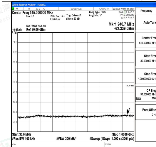
Band41_15MHz_QPSK_41515_1RB#0_30~1000_30~1000
