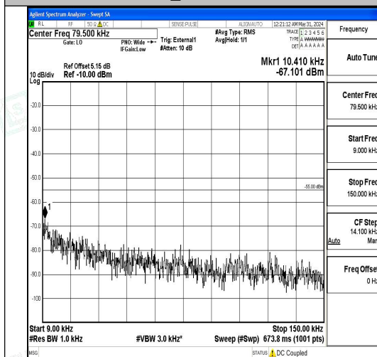
Band41_20MHz_QPSK_41490_1RB#0_0.009~0. 15_0.009~0.15
