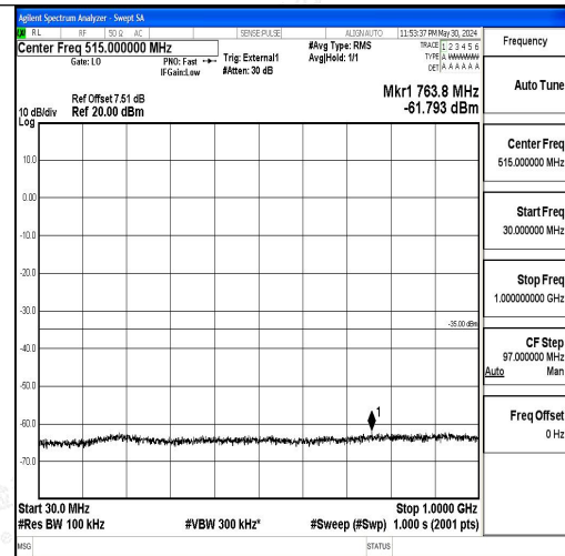
Band41_15MHz_16QAM_40620_1RB#0_30~1000 _30~1000
