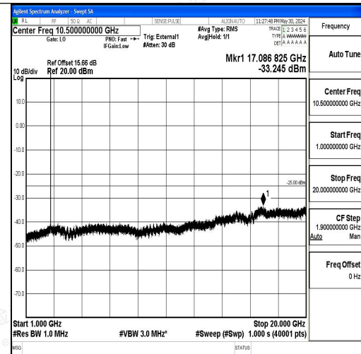
Band41_10MHz_QPSK_41540_1RB#0_1000~20000_1000~20000
