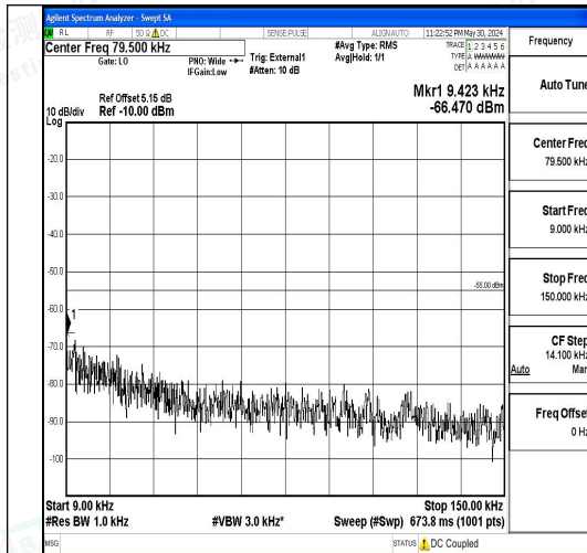
Band41_10MHz_QPSK_40620_1RB#0_0.009~0.15_0.009~0.15
