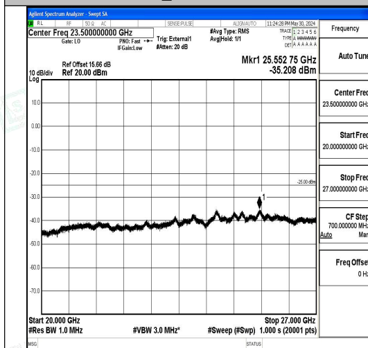
Band41_10MHz_QPSK_40620_1RB#0_20000~27000_7000_20000~27000
