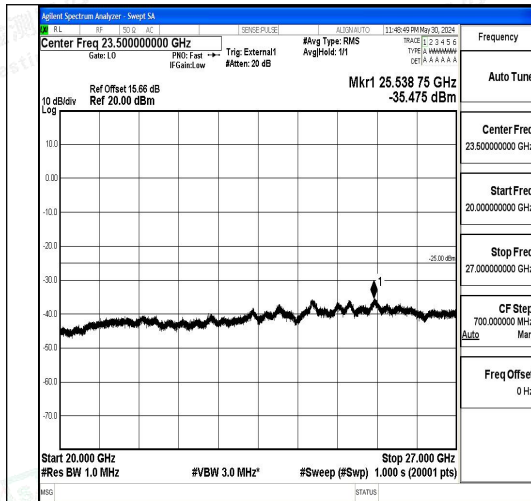
Band41_15MHz_QPSK_39725_1RB#0_20000~27000_20000~27000
