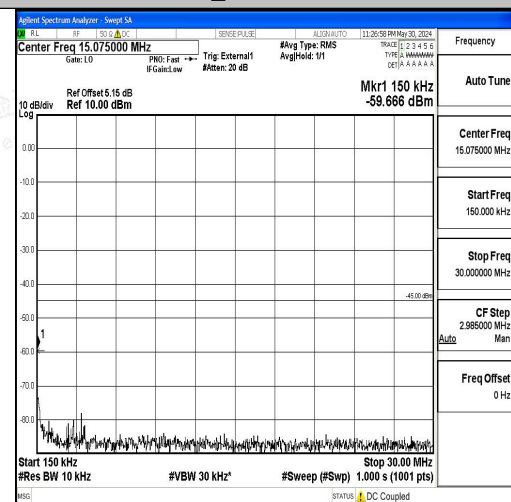
Band41_10MHz_QPSK_41540_1RB#0_0.15~30 0.15~30
