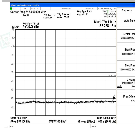
Band41_15MHz_QPSK_39725_1RB#0_30~1000
