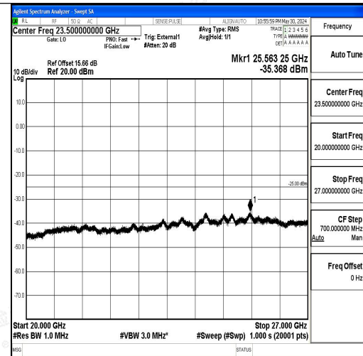
Band41_5MHz_16QAM_41565_1RB#0_20000~27000_000_20000~27000
