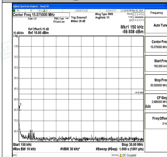
Band41_10MHz_16QAM_41540_1RB#0_0.15~30_0.15~30
