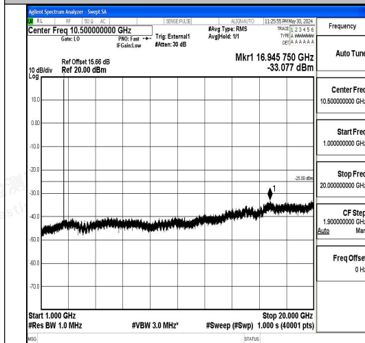
Band41_10MHz_16QAM_40620_1RB#0_1000~2 0000_1000~20000
