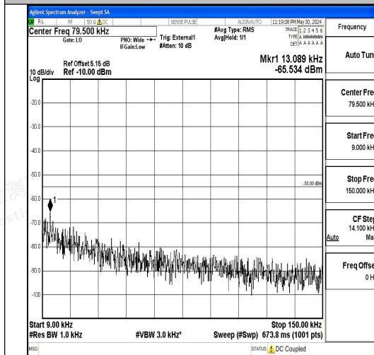
Band41_10MHz_QPSK_39700_1RB#0_0.009~0.15_0.009~0.15
