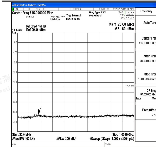
Band41_10MHz_QPSK_40620_1RB#0_30~1000_30~1000
