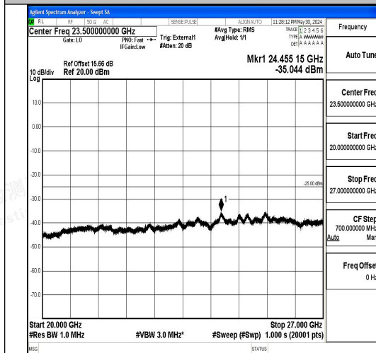
Band41_10MHz_QPSK_41540_1RB#0_20000~27000_20000~27000
