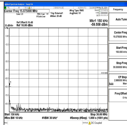
Band41_10MHz_QPSK_39700_1RB#0_0.15~30_0.15~30
