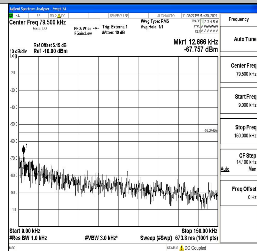
Band41_10MHz_16QAM_41540_1RB#0_0.009~0.15_0.009~0.15
