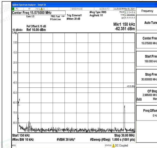
Band41_10MHz_16QAM_40620_1RB#0_0.15~30 0_0.15~30
