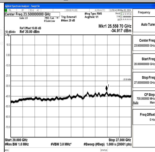
Band41_15MHz_16QAM_39725_1RB#0_20000~27000_20000~27000
