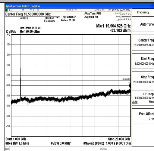
Band41_15MHz_QPSK_39725_1RB#0_1000~20000
