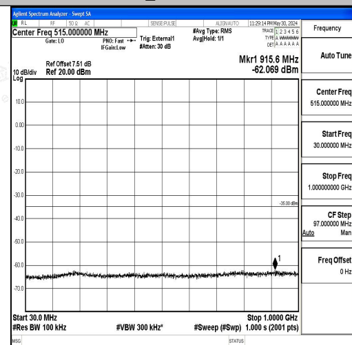
Band41_10MHz_16QAM_41540_1RB#0_30~1000_30~1000
