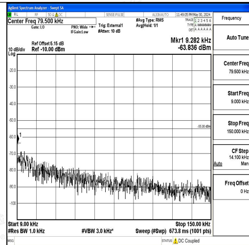
Band41_15MHz_16QAM_39725_1RB#0_0.009~0.15_0.009~0.15
