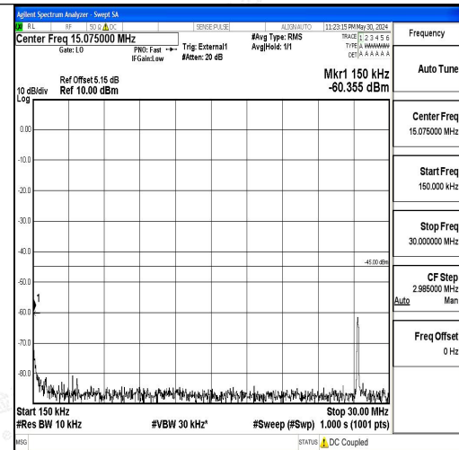
Band41_10MHz_QPSK_40620_1RB#0_0.15~30_0.15~30
