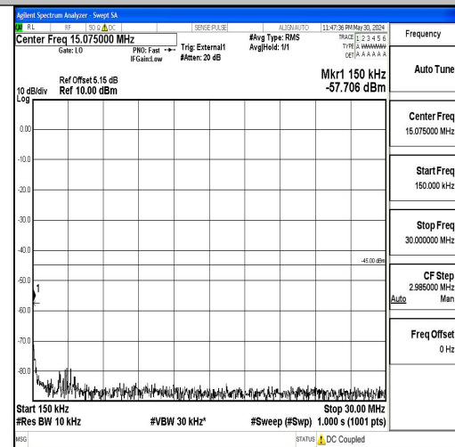
Band41_15MHz_QPSK_39725_1RB#0_0.15~30
