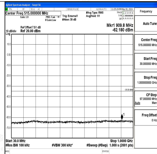
Band41_10MHz_16QAM_40620_1RB#0_30~1000 _30~1000
