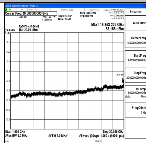
Band41_10MHz_QPSK_39700_1RB#0_1000~20000_00_1000~20000
