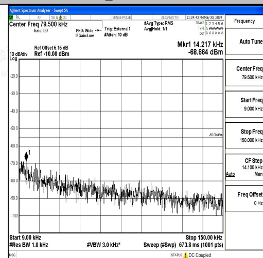
Band41_10MHz_16QAM_40620_1RB#0_0.009~0.15_0.009~0.15
