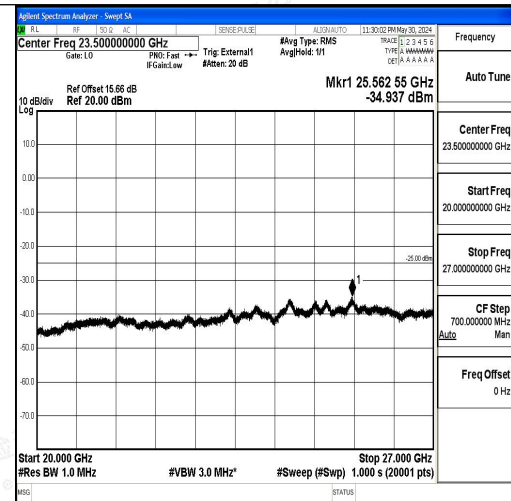
Band41_10MHz_16QAM_41540_1RB#0_20000~27000
