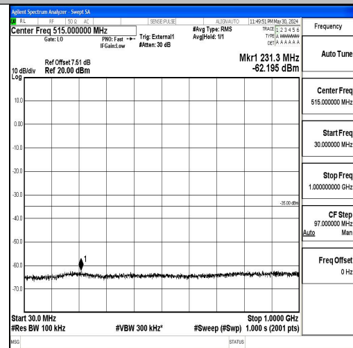
Band41_15MHz_16QAM_39725_1RB#0_30~1000_30~1000
