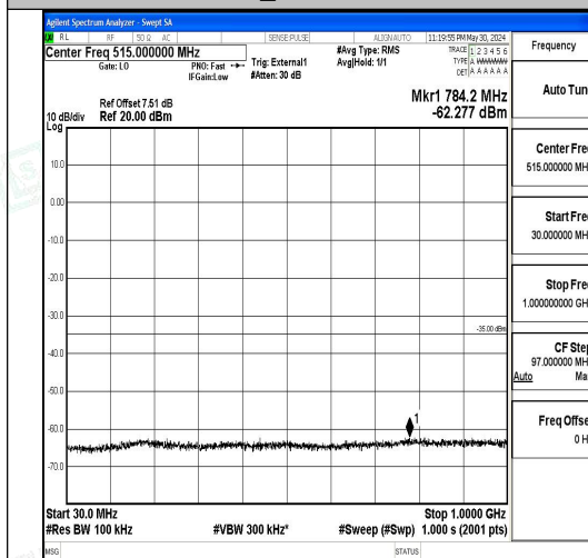
Band41_10MHz_QPSK_39700_1RB#0_30~1000_30~1000
