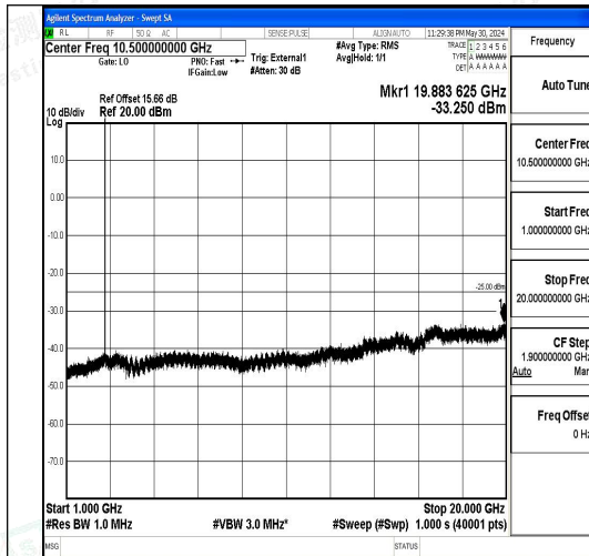
Band41_10MHz_16QAM_41540_1RB#0_1000~20000
