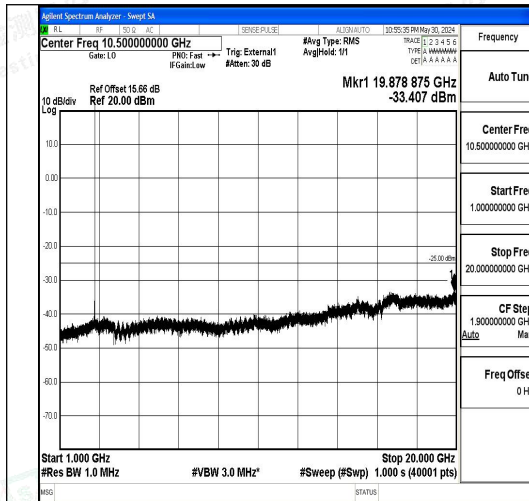
Band41_5MHz_16QAM_41565_1RB#0_1000~20000_000_1000~20000
