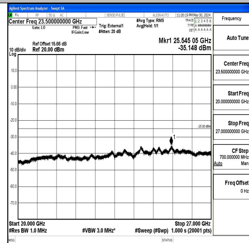
Band41_10MHz_16QAM_40620_1RB#0_2000~2 7000_20000~27000
