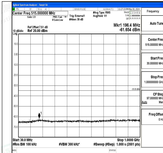
Band41_10MHz_QPSK_41540_1RB#0_30~1000_30~1000
