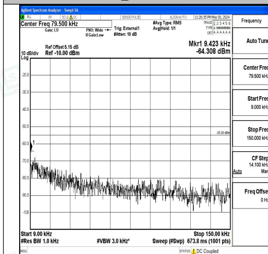
Band41_10MHz_QPSK_41540_1RB#0_0.009~0. 15_0.009~0.15
