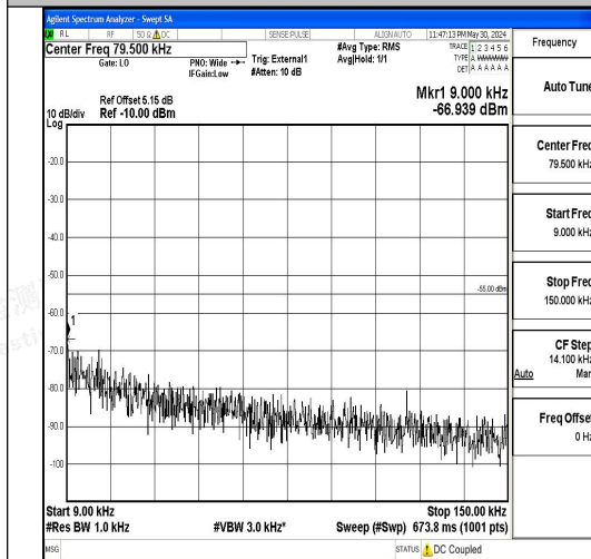
Band41_15MHz_QPSK_39725_1RB#0_0.009~0.15
