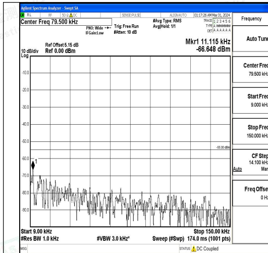
Band7_15MHz_QPSK_21100_1RB#0_0.009~0.15_5_0.009~0.15
