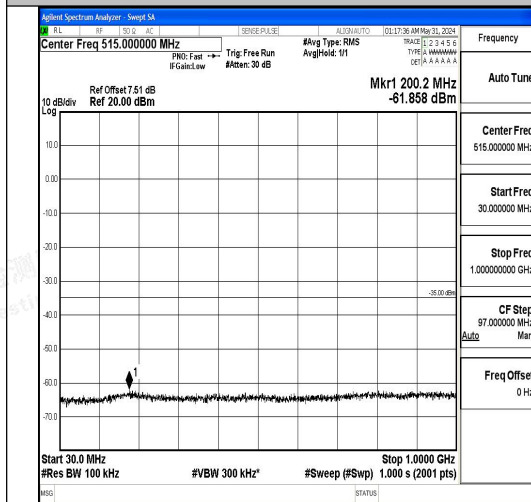
Band7_15MHz_QPSK_21100_1RB#0_30~1000_30~1000
