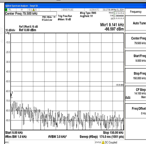
Band7_15MHz_16QAM_21100_1RB#0_0.009~0.15_5_0.009~0.15
