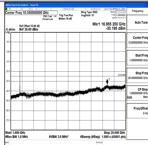
Band7_15MHz_QPSK_21100_1RB#0_1000~2000_0_1000~20000
