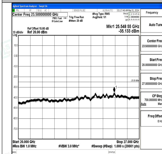
Band7_15MHz_QPSK_21100_1RB#0_20000~27000_000_20000~27000
