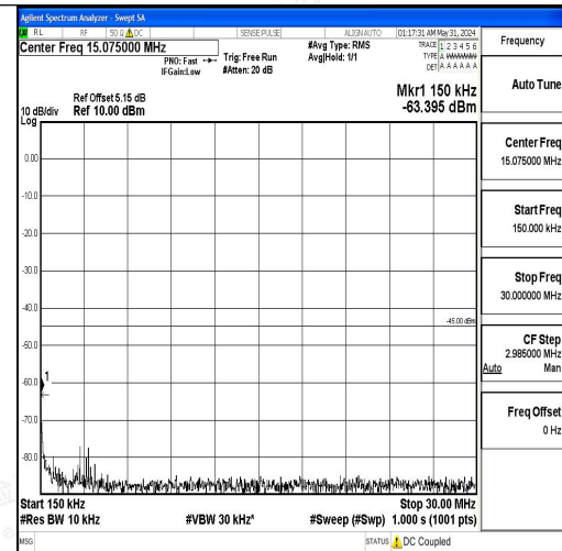
Band7_15MHz_QPSK_21100_1RB#0_0.15~30_0.15~30
