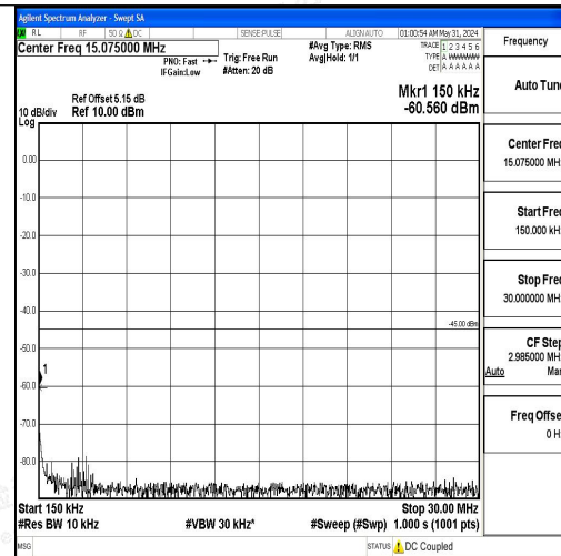
Band7_10MHz_QPSK_21100_1RB#0_0.15~30_0.15~30
