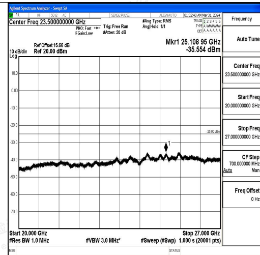
Band7_10MHz_16QAM_21400_1RB#0_20000~27000
