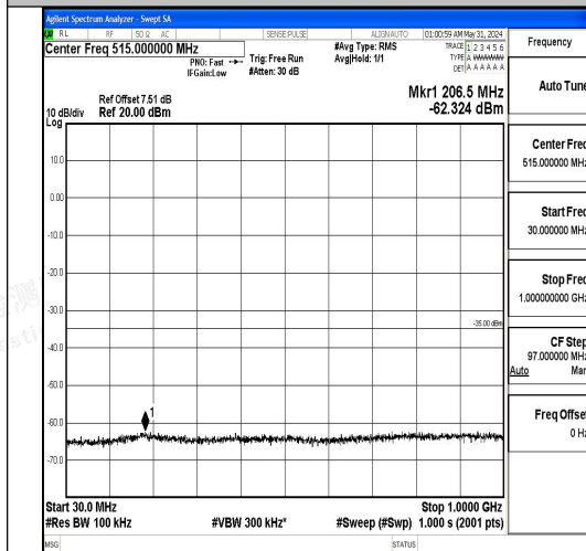
Band7_10MHz_QPSK_21100_1RB#0_30~1000_30~1000
