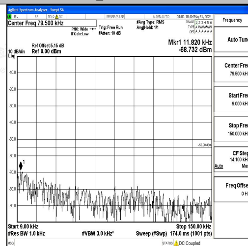
Band7_10MHz_16QAM_21100_1RB#0_0.009~0.15_5_0.009~0.15
