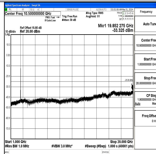
Band7_10MHz_QPSK_21100_1RB#0_1000~2000_0_1000~20000
