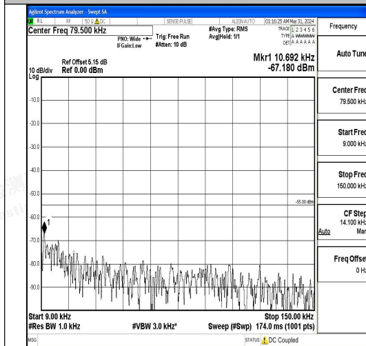
Band7_15MHz_QPSK_20825_1RB#0_0.009~0.15
