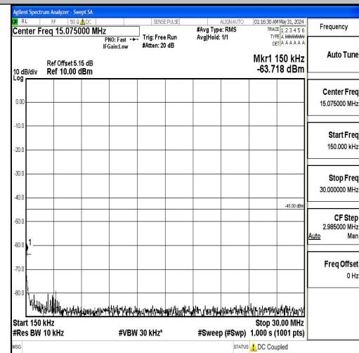
Band7_15MHz_QPSK_20825_1RB#0_0.15~30
