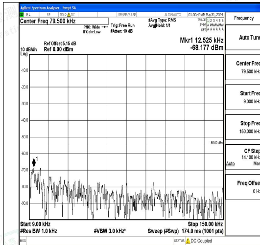
Band7_10MHz_QPSK_21100_1RB#0_0.009~0.15_5_0.009~0.15
