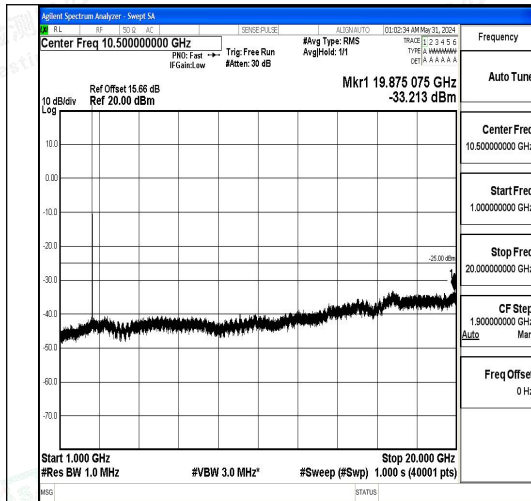
Band7_10MHz_16QAM_21400_1RB#0_1000~20000
