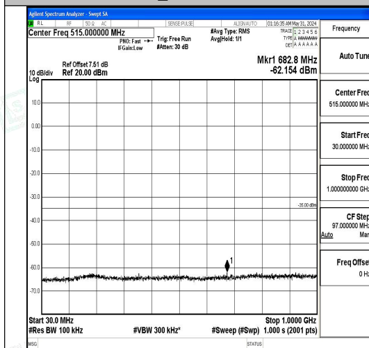
Band7_15MHz_QPSK_20825_1RB#0_30~1000
