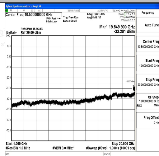
Band7_15MHz_QPSK_20825_1RB#0_1000~20000
