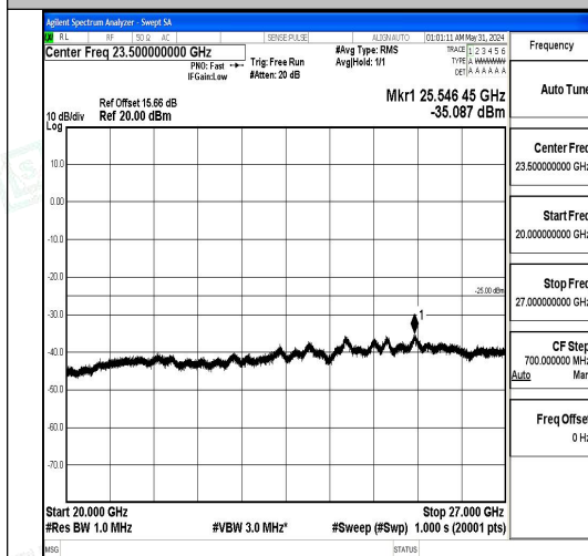
Band7_10MHz_QPSK_21100_1RB#0_20000~27000_000_20000~27000
