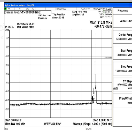
Band5_10MHz_16QAM_20600_1RB#0_30~1000_30~1000
