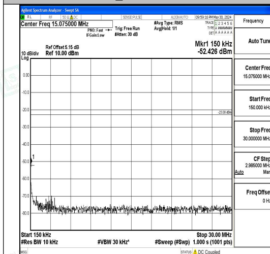
Band5_10MHz_16QAM_20600_1RB#0_0.15~30_0.15~30
