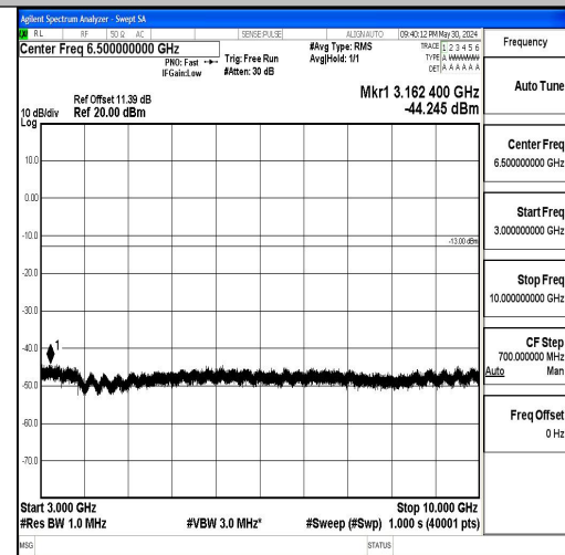
Band5_5MHz_16QAM_20525_1RB#0_3000~10000_0_3000~10000
