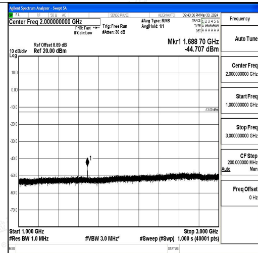
Band5_5MHz_QPSK_20625_1RB#0_1000~3000_1000~3000
