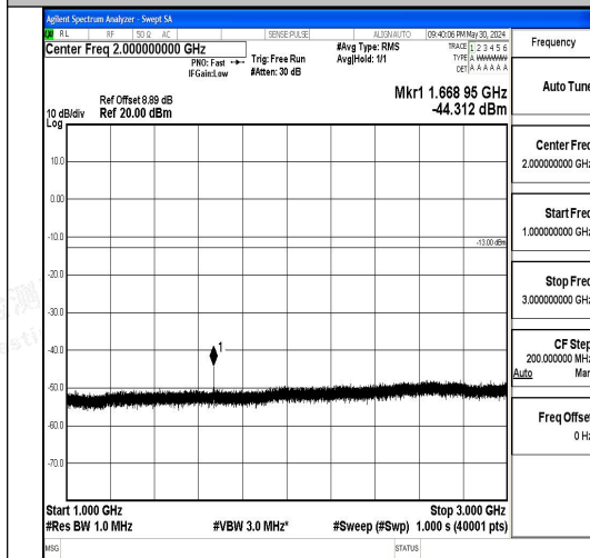
Band5_5MHz_16QAM_20525_1RB#0_1000~3000_0_1000~3000
