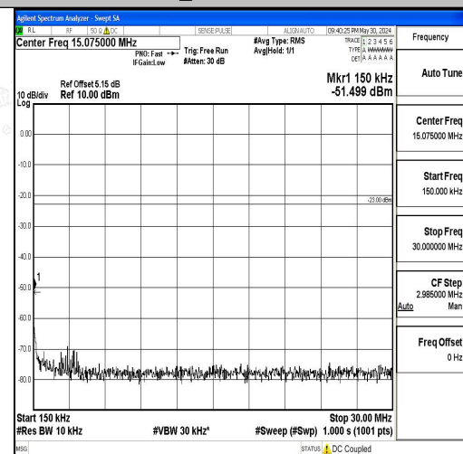
Band5_5MHz_QPSK_20625_1RB#0_0.15~30_0.15~30
