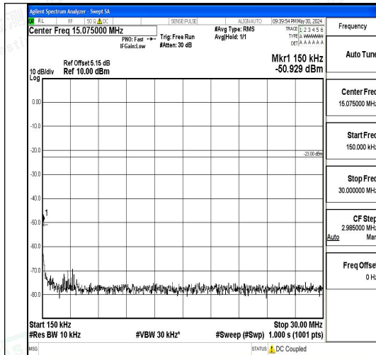
Band5_5MHz_16QAM_20525_1RB#0_0.15~30_0.15~30
