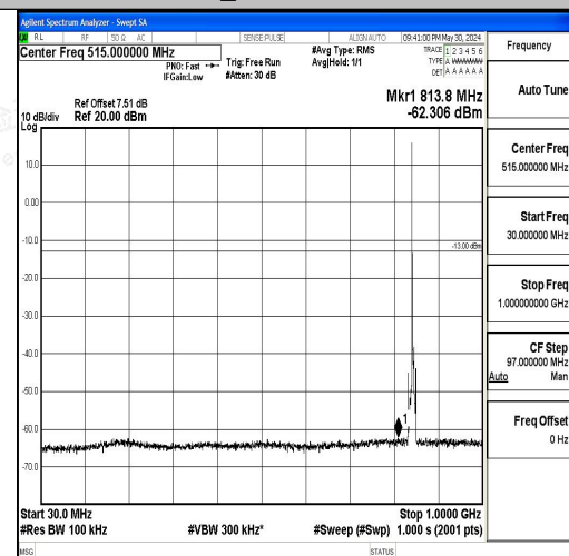
Band5_5MHz_16QAM_20625_1RB#0_30~1000_3_0~1000
