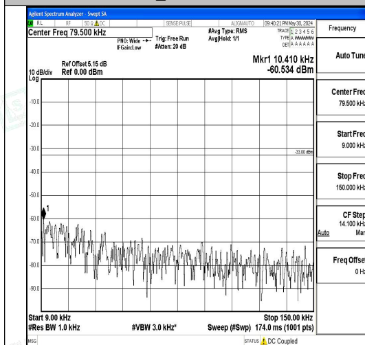
Band5_5MHz_QPSK_20625_1RB#0_0.009~0.15_0.009~0.15
