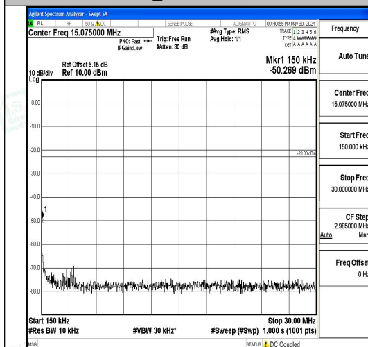
Band5_5MHz_16QAM_20625_1RB#0_0.15~30_0.15~30
