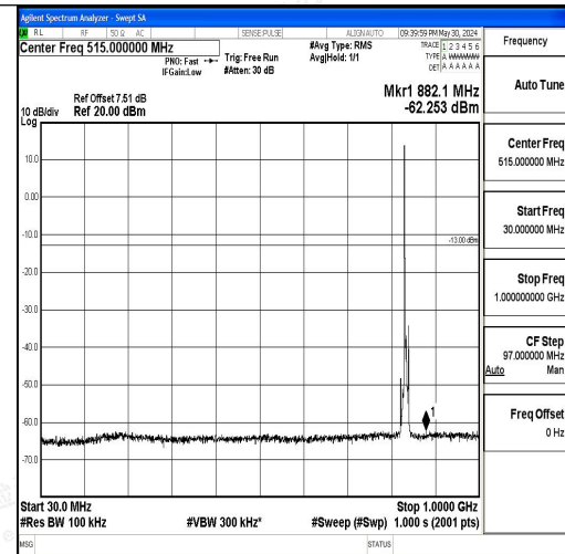
Band5_5MHz_16QAM_20525_1RB#0_30~1000_30~1000
