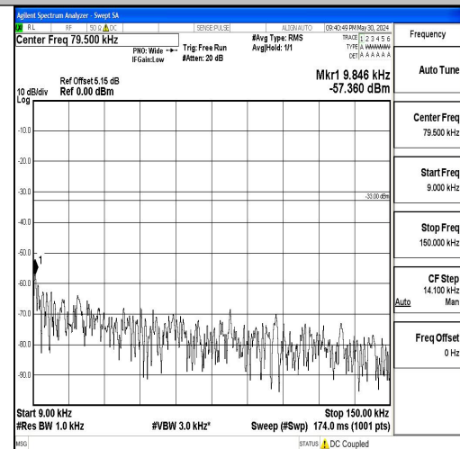
Band5_5MHz_16QAM_20625_1RB#0_0.009~0.15_0.009~0.15
